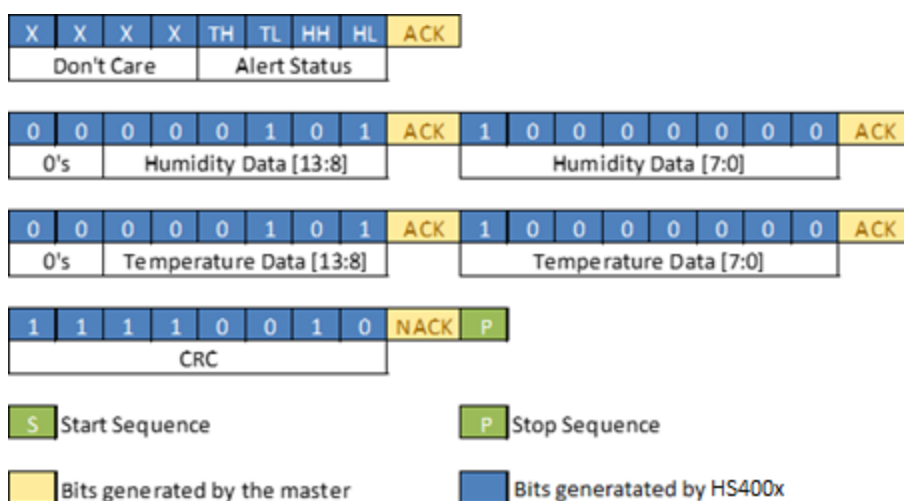
Figure 20. Data Returned from HS401x when the Alert Feature is Enabled in Periodic Measurement Mode
