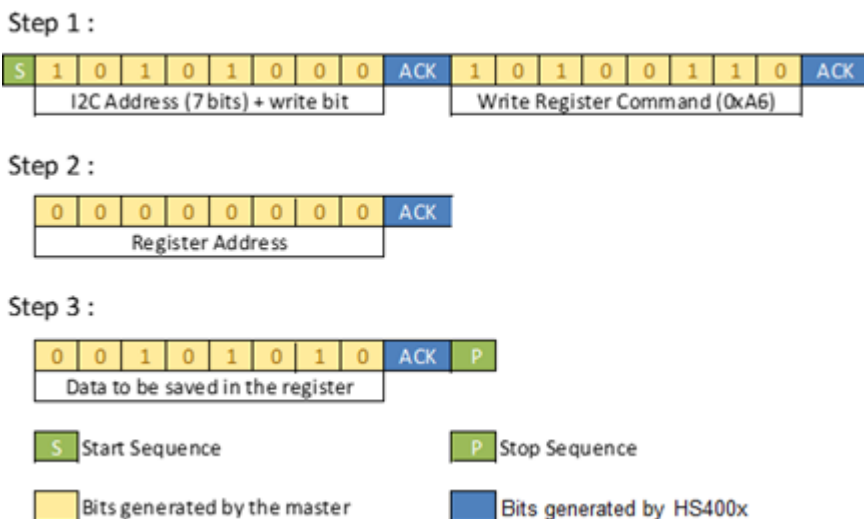
Figure 22. Write Register Command Sequence
