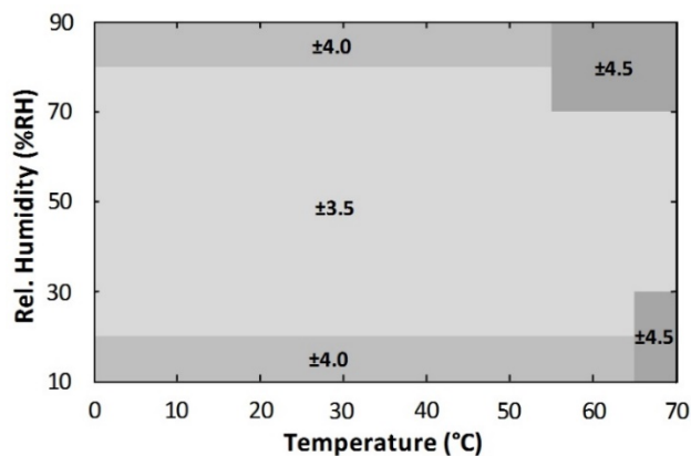
Figure 8. HS4014 RH Accuracy over Temperature
