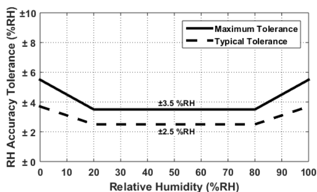
Figure 5. HS4013 RH Accuracy Tolerance at 25°C
