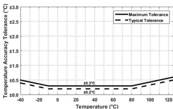
Figure 9. HS4011/HS4012 Temperature Sensor Accuracy Tolerance
