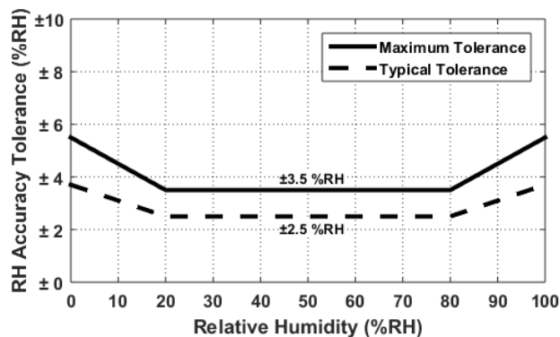
Figure 5. HS4103 RH Accuracy Tolerance at 25°C
