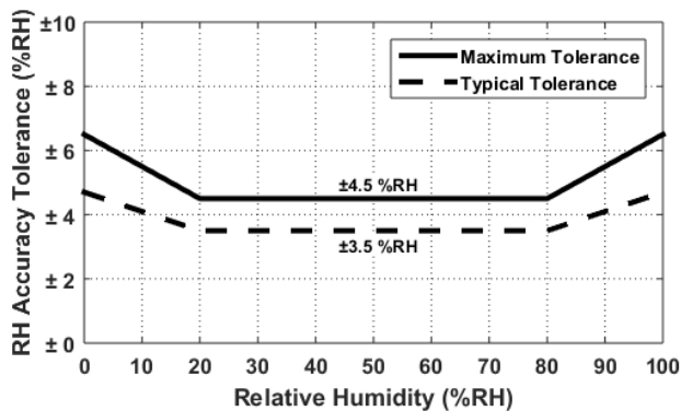
Figure 7. HS4104 RH Accuracy Tolerance at 25°C
