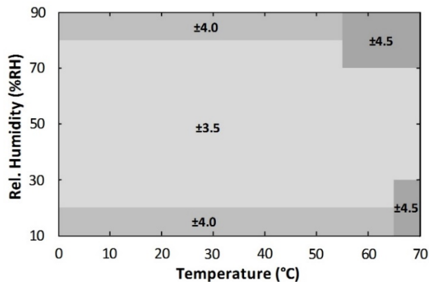
Figure 8. HS4104 RH Accuracy over Temperature
