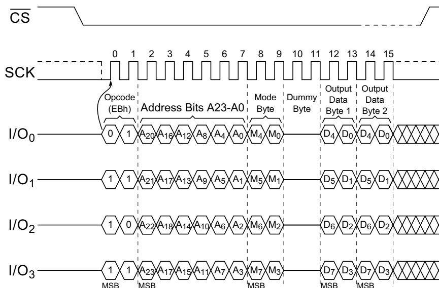
Figure 24. Fast Read Quad I/O Command (Initial command or previous M7-0 \neq Axx, QPI mode, 80 MHz)
