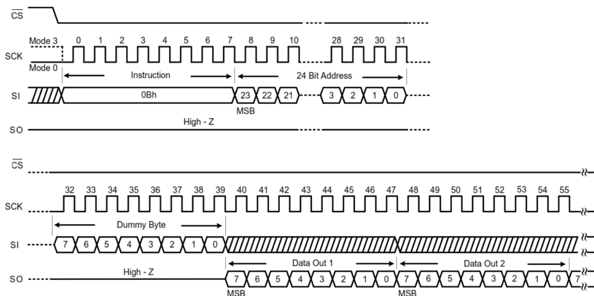
Figure 15. Fast Read Command (SPI Mode)
