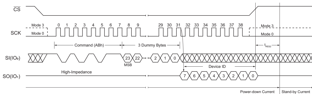
Figure 45. Release Power-Down / Device ID Command (SPI Mode)
