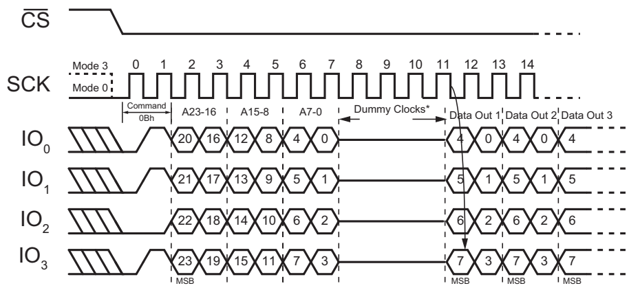
Figure 16. Fast Read Command (QPI Mode, 80MHz)
