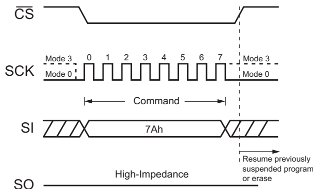
Figure 39. Erase / Program Resume command (SPI Mode)
