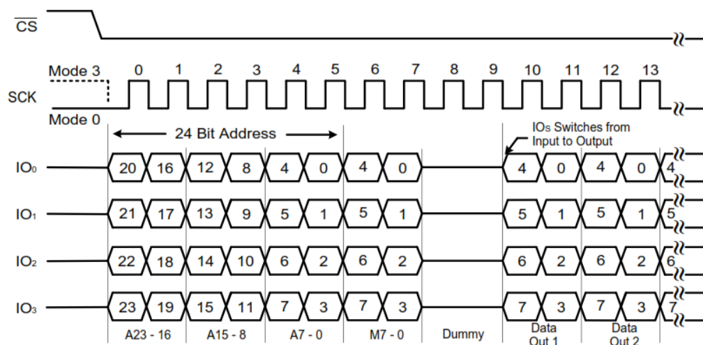
Figure 56. Set Burst with Wrap Command Sequence
