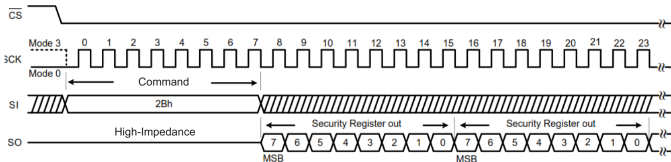
Figure 65. Read Security Register Command (SPI Mode)
