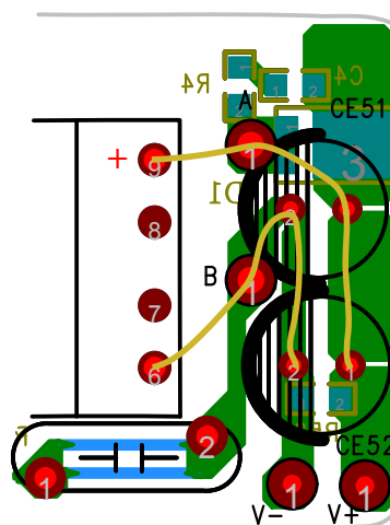
Figure 10.9b : Secondary-Side Layout Path Recommendation
