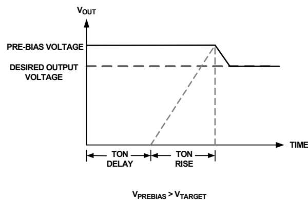
FIGURE 7. OUTPUT RESPONSES TO PREBIAS VOLTAGES
