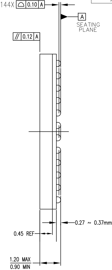
SIDE VIEW
