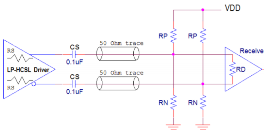
Figure 45. AC-Coupling Termination
