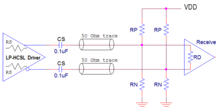
Figure 46. AC-Coupling Termination
