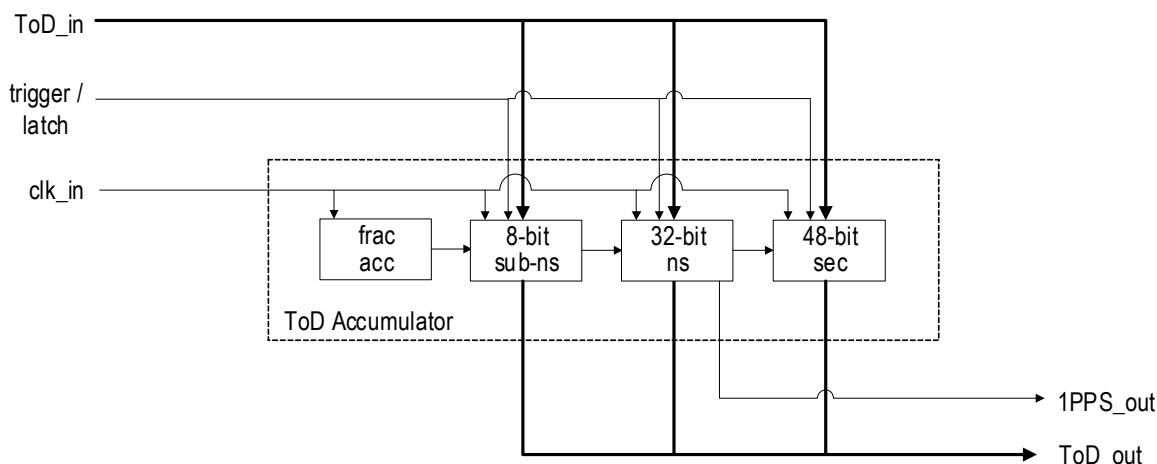
Figure 33. ToD Accumulator
