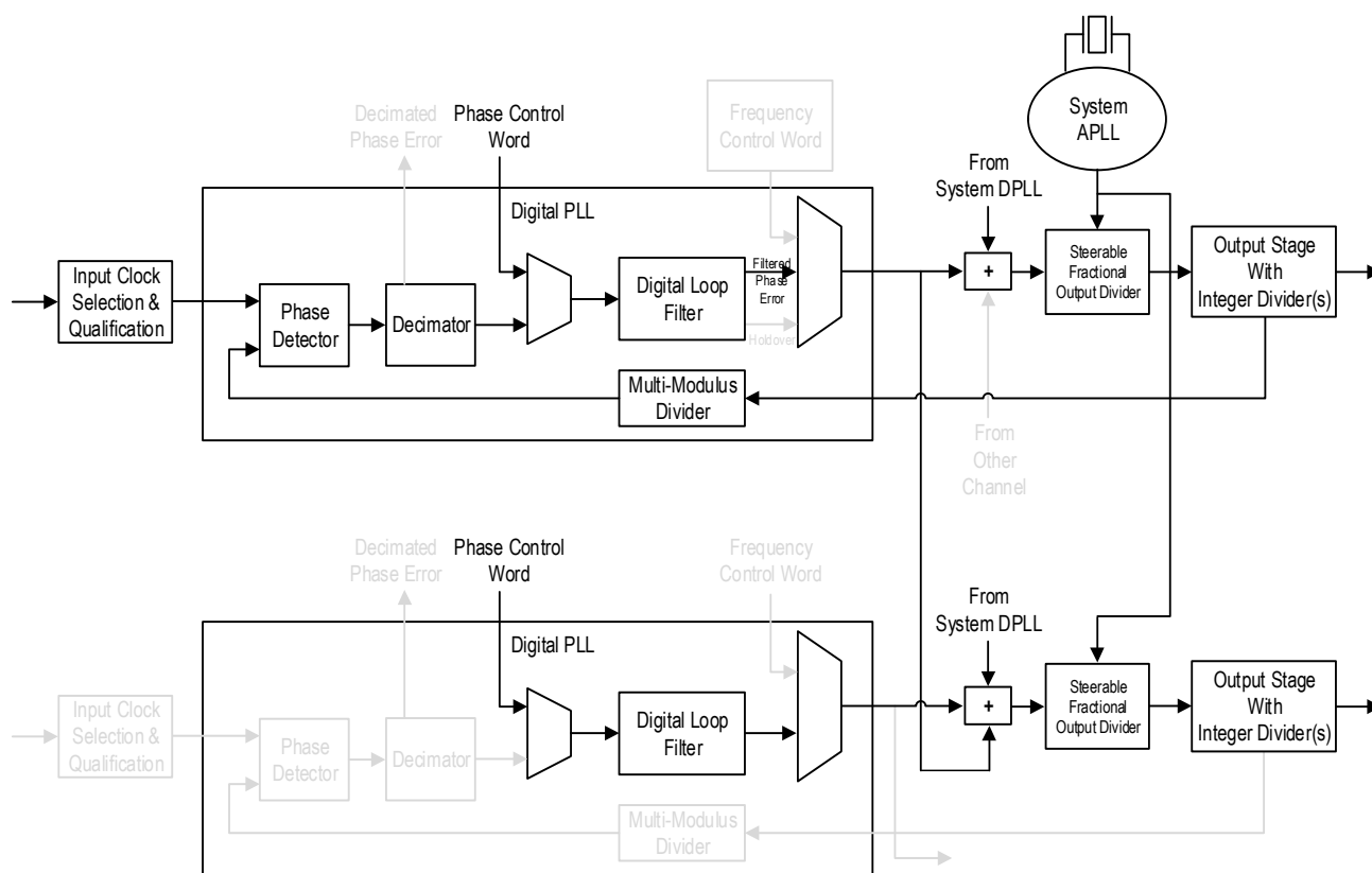
Figure 31. Combo Mode
