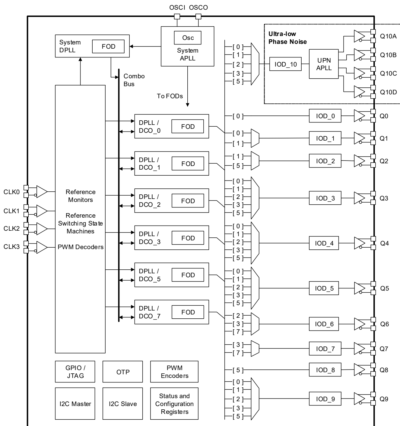
Figure 1. Block Diagram [1]
