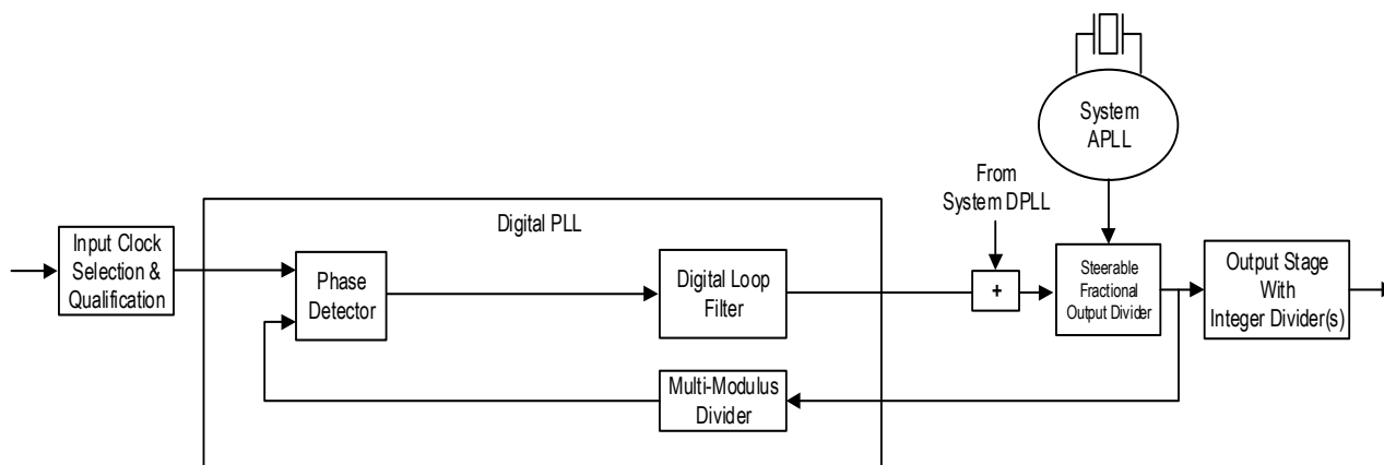
Figure 27. Jitter Attenuator Disciplined with Oscillator Operation
