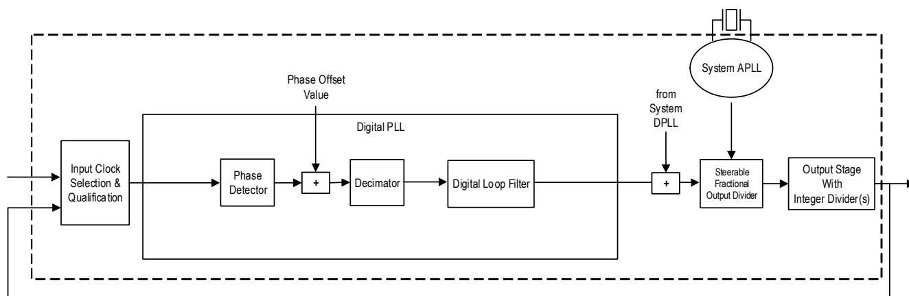
Figure 13. External Feedback
