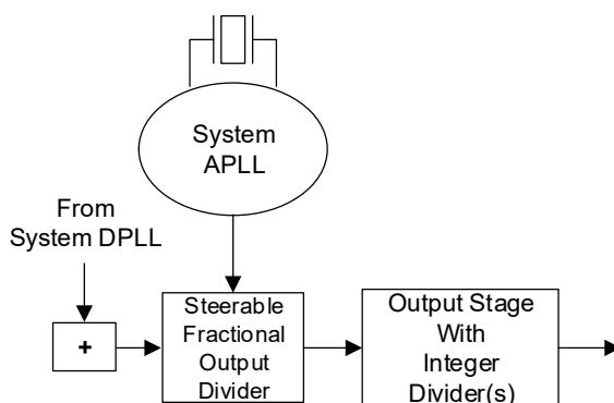
Figure 24. Synthesizer Disciplined with Oscillator Operation
