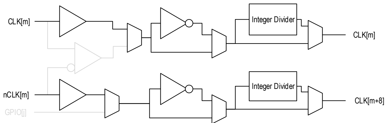
Figure 7. Input Stage Configured as Dual Single-Ended
