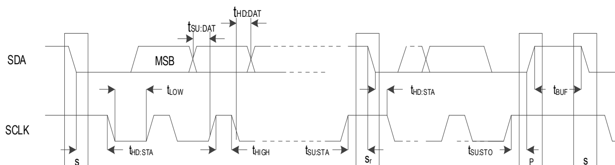
Figure 20. I²C Slave Timing Diagram
