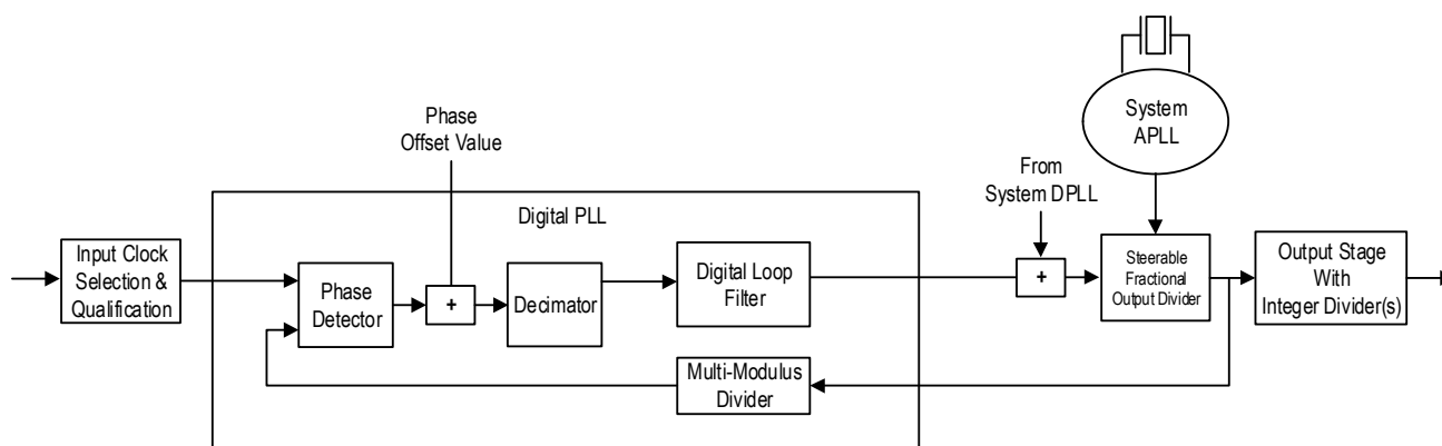
Figure 30. Phase Control in Closed Loop Operation
