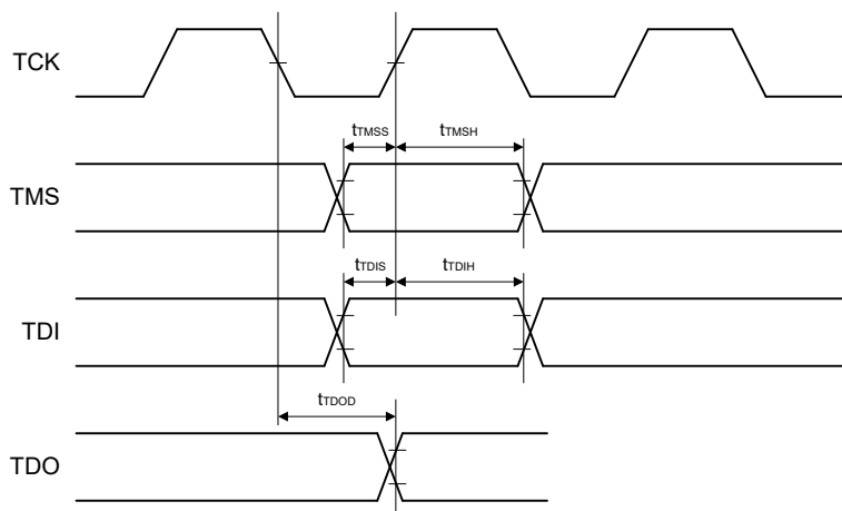
Figure 2.68 Boundary scan input/output timing
