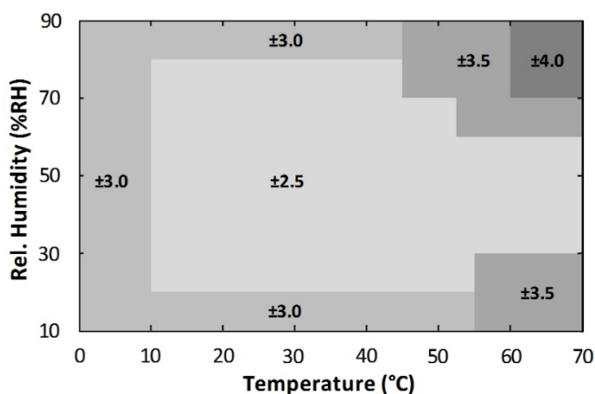
Figure 5. HS3003-MC1 RH Accuracy over Temperature
