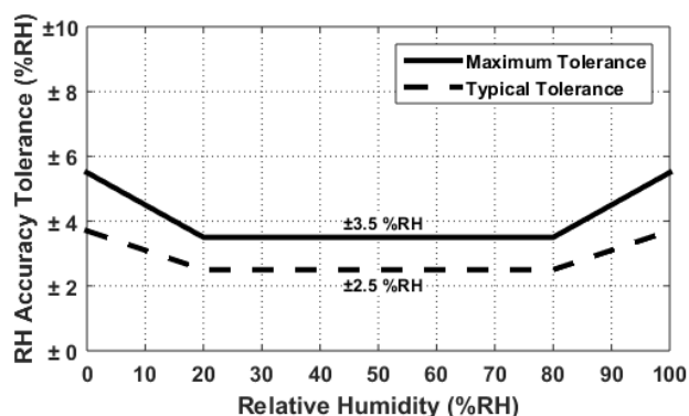
Figure 4. HS3003-MC1 RH Accuracy Tolerance at 25°C
