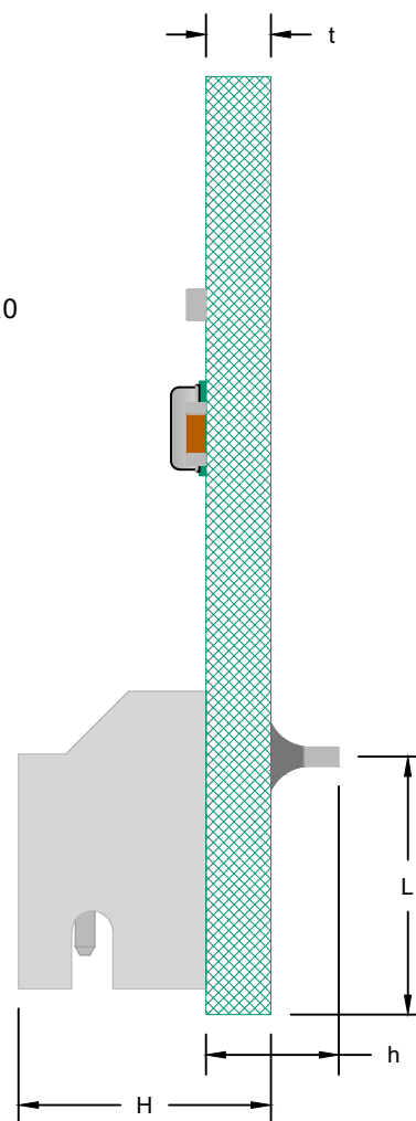
SIDE VIEW
