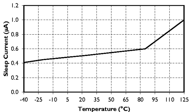
Figure 1. Sleep Current Variation over Temperature, V_{DD} at 3.3\text{V}
