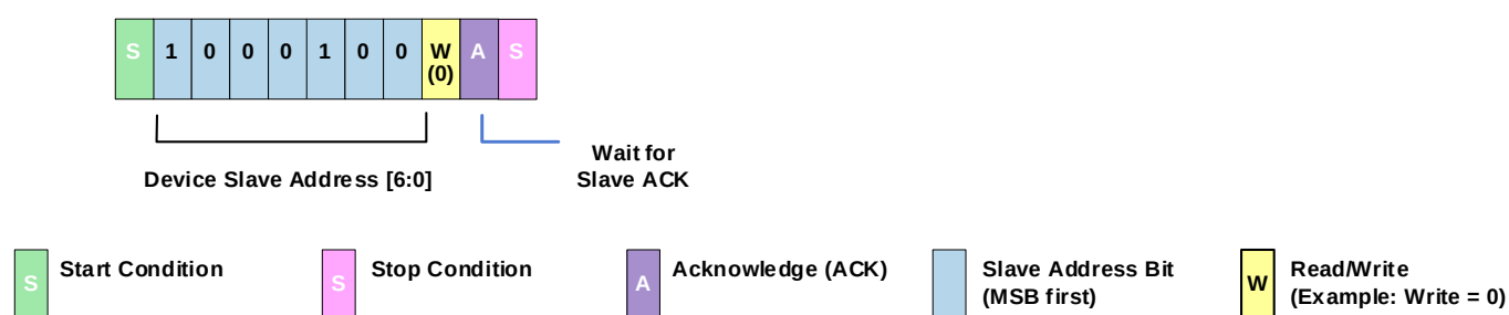
Figure 10. Measurement Request
