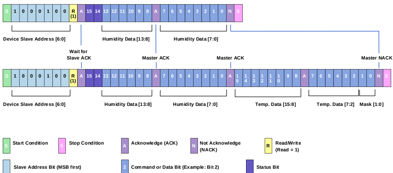
Figure 11. Data Fetch
