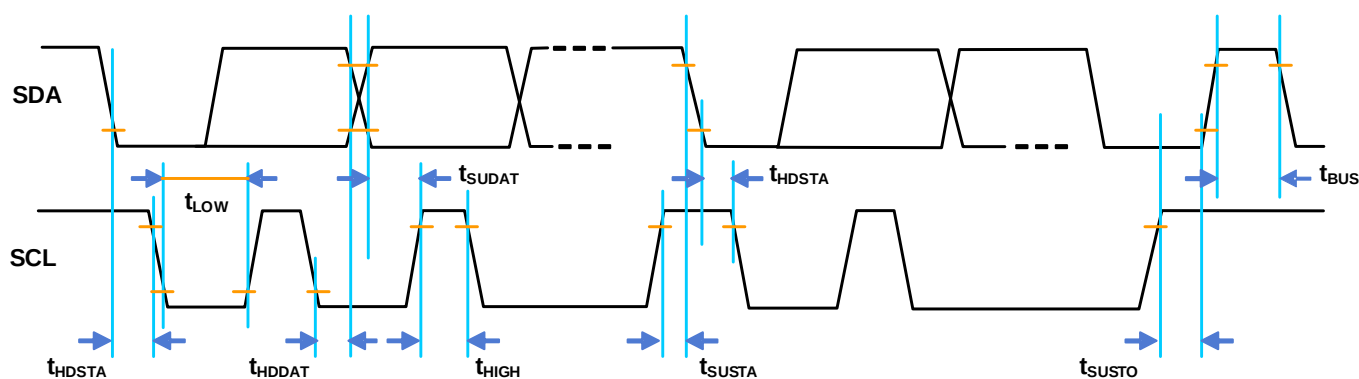
Figure 8. Timing Diagram
