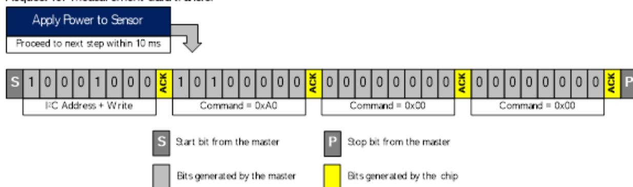
Figure 12. Sequence of Commands to Enter Programming Mode
