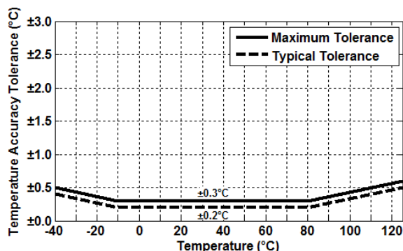
Figure 6. HS3001-MC1 Temperature Sensor Accuracy Tolerance
