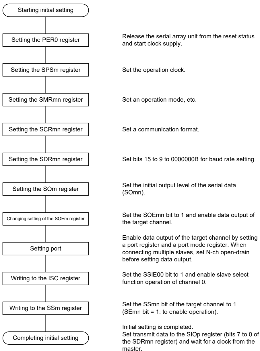
Figure 19 - 99 Initial Setting Procedure for Slave Transmission/Reception
