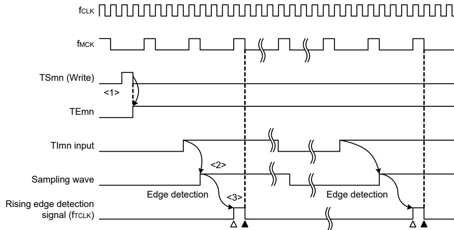
Figure 6 - 28 Timing of f TCLK and Count Clock (f TCLK ) (When CCSmn = 1, noise filter unused)
