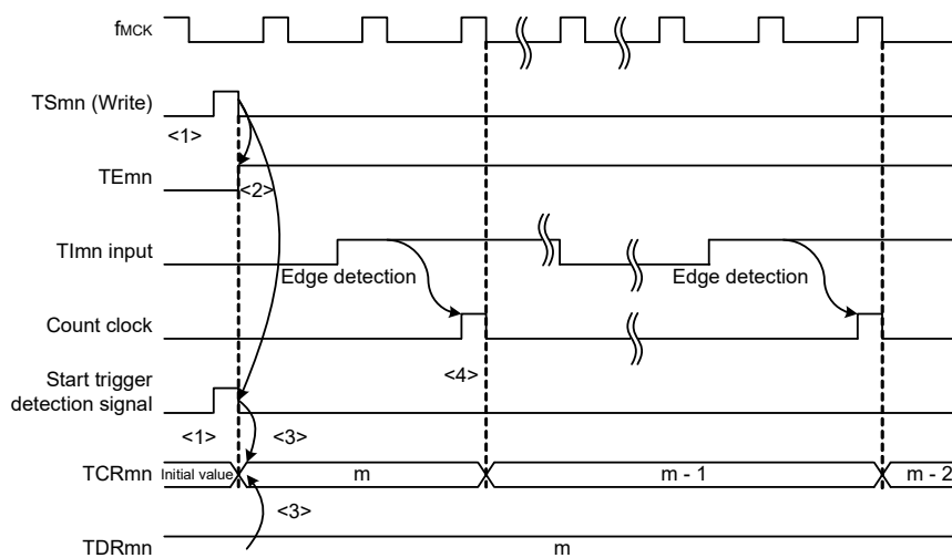
Figure 6 - 30 Operation Timing (In Event Counter Mode)
