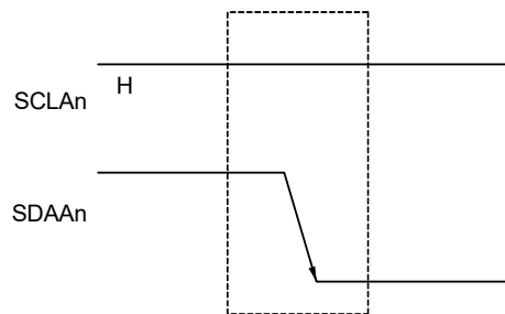
Figure 20 - 21 Start Conditions
