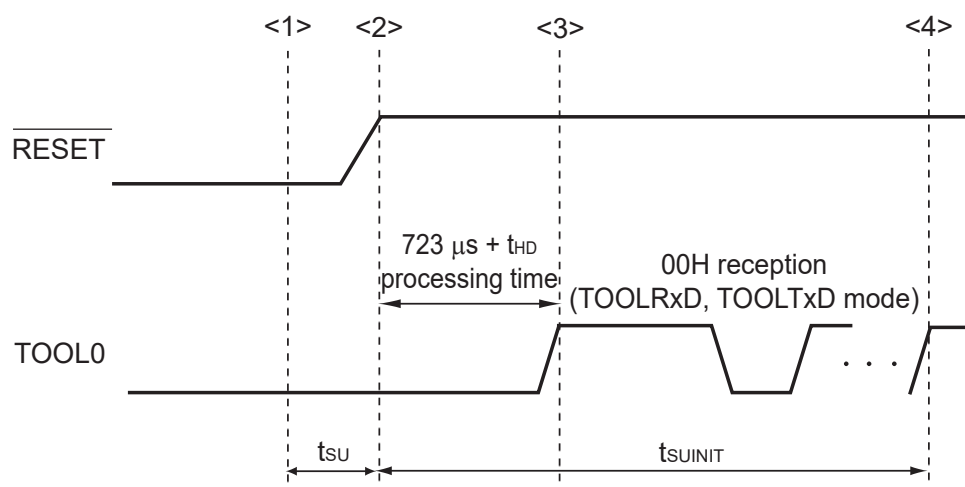
Figure 33 - 7 Setting of Flash Memory Programming Mode
