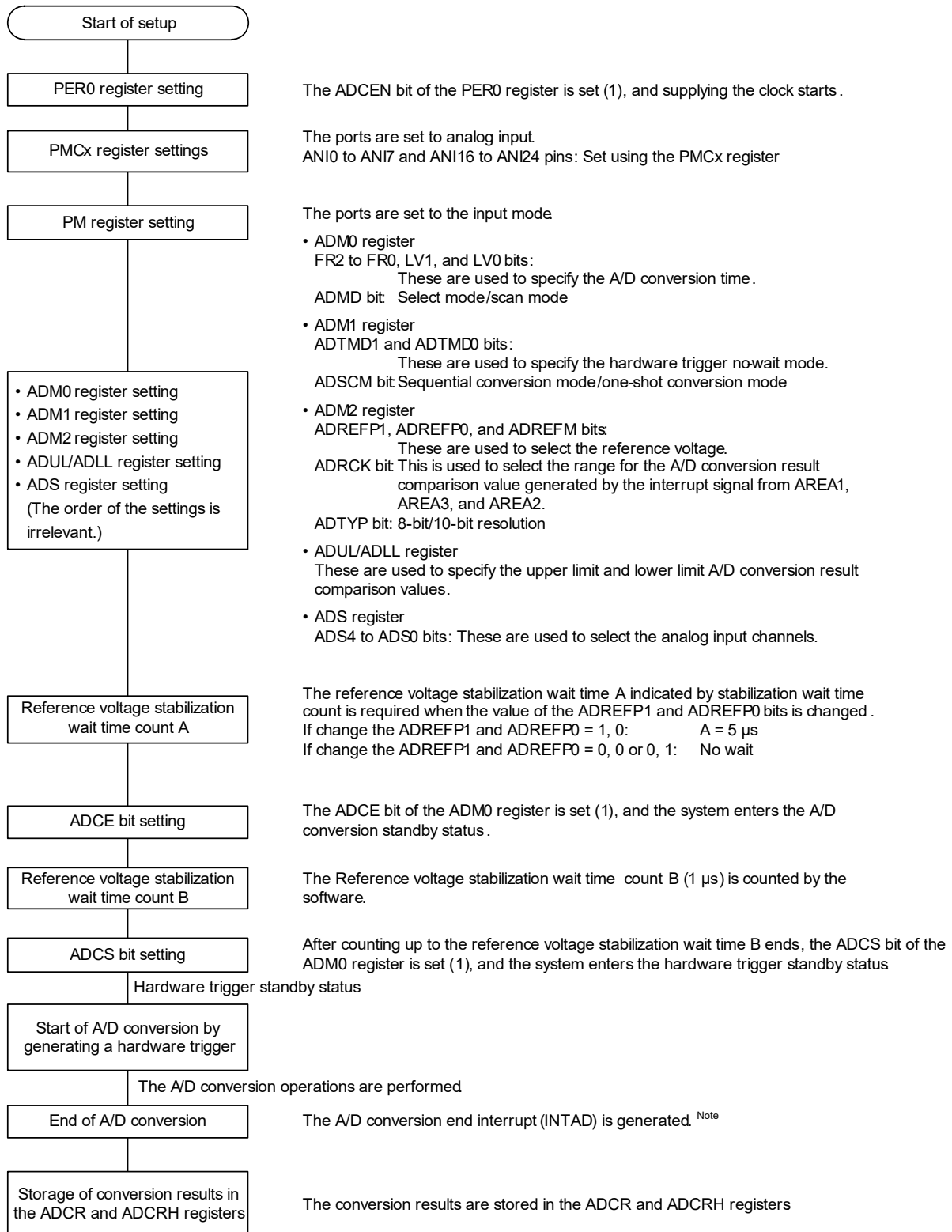
Figure 15 - 32 Setting up Hardware Trigger No-Wait Mode
