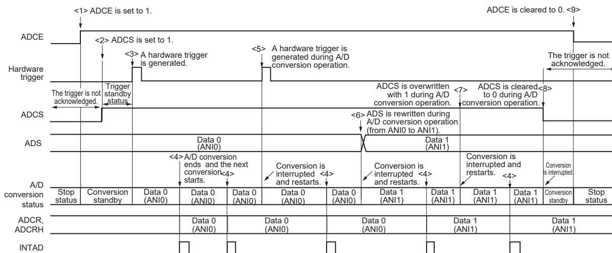
Figure 15 - 23 Example of Hardware Trigger No-Wait Mode (Select Mode, Sequential Conversion Mode) Operation Timing
