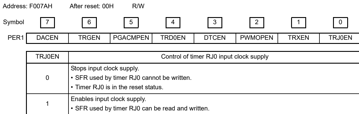
Figure 7 - 2 Format of Peripheral enable register 1 (PER1)
