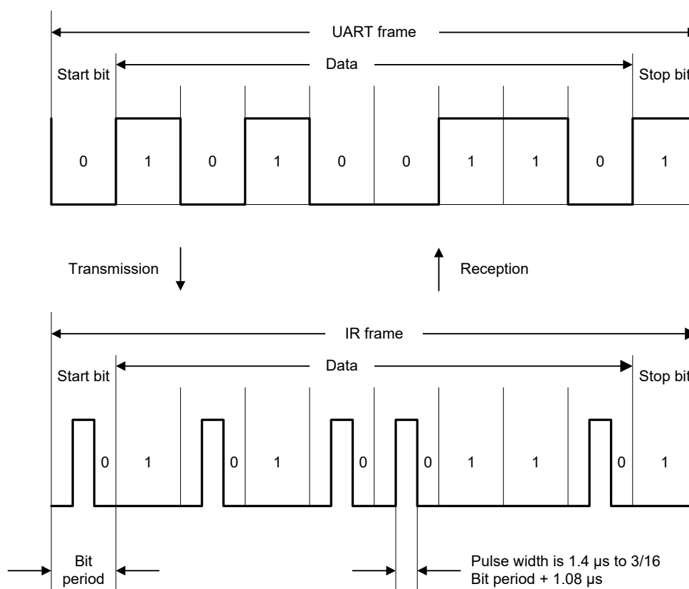
Figure 21 - 4 IrDA Transmission/Reception
