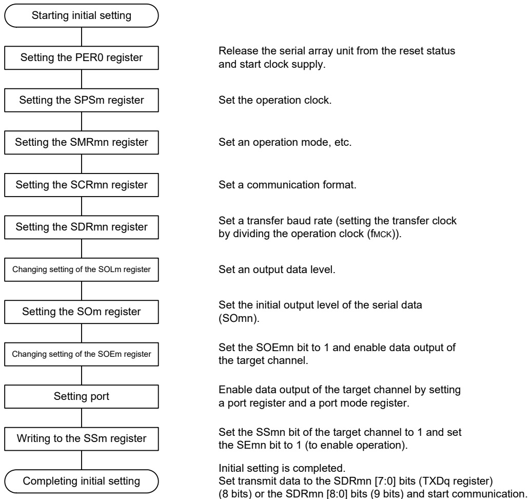
Figure 19 - 109 Initial Setting Procedure for UART Transmission
