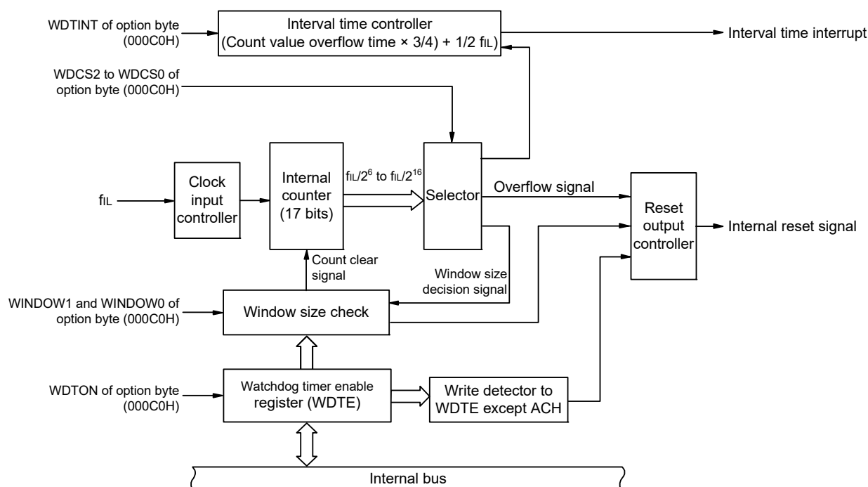
Figure 14 - 1 Block Diagram of Watchdog Timer
