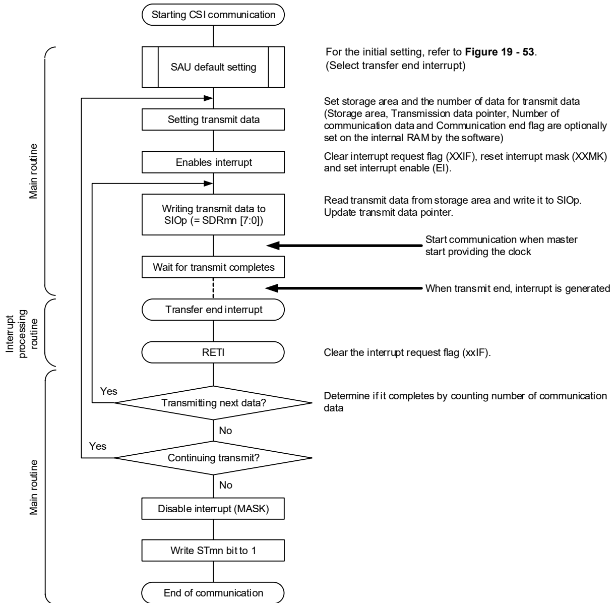
Figure 19 - 57 Flowchart of Slave Transmission (in Single-Transmission Mode)
