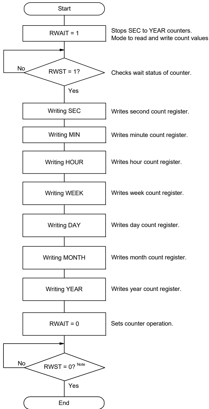
Figure 11 - 23 Procedure for Writing Real-time Clock
