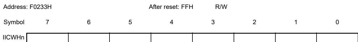
Figure 20 - 17 Format of IICA high-level width setting register n (IICWHn)
