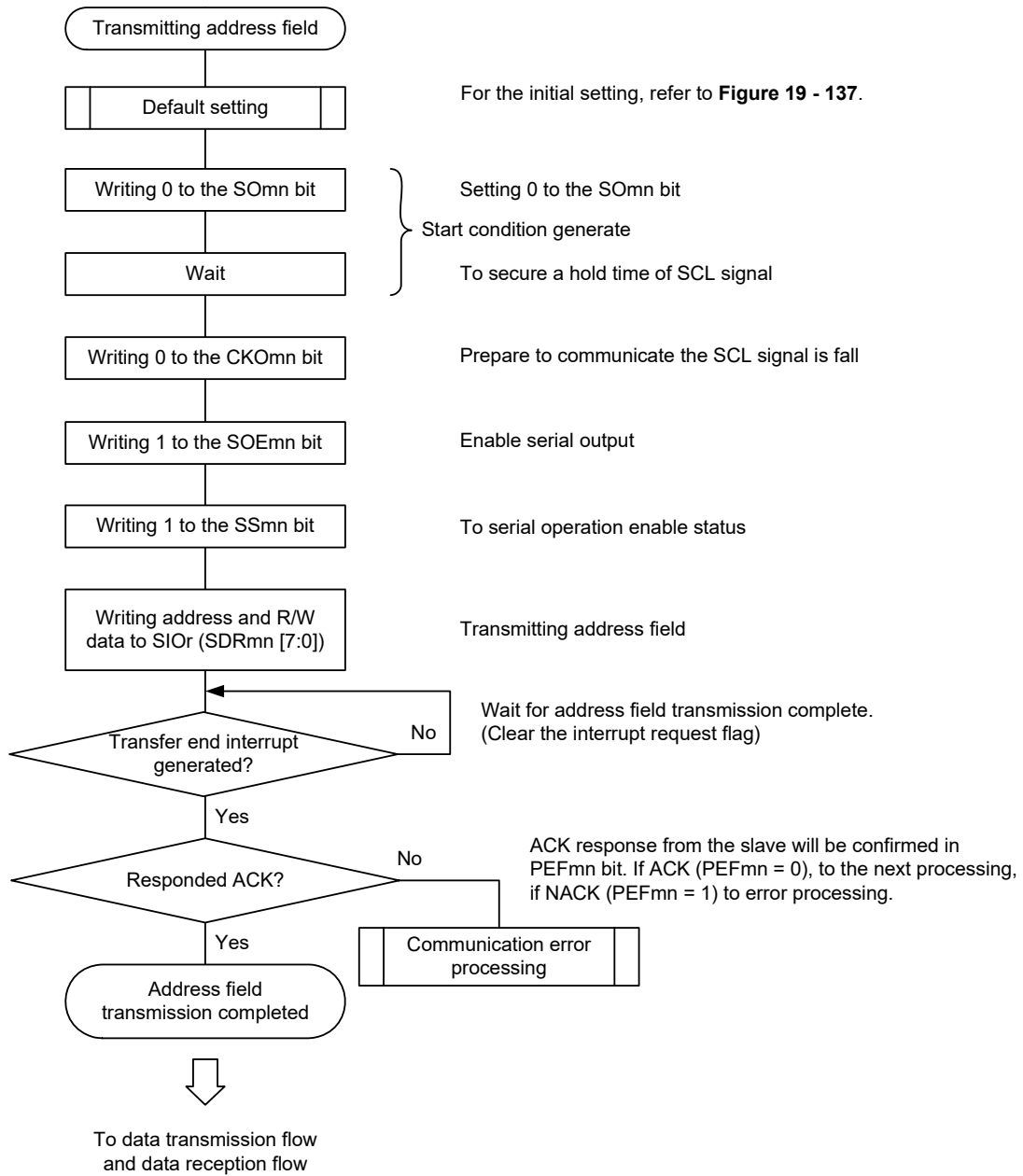
Figure 19 - 139 Flowchart of Address Field Transmission
