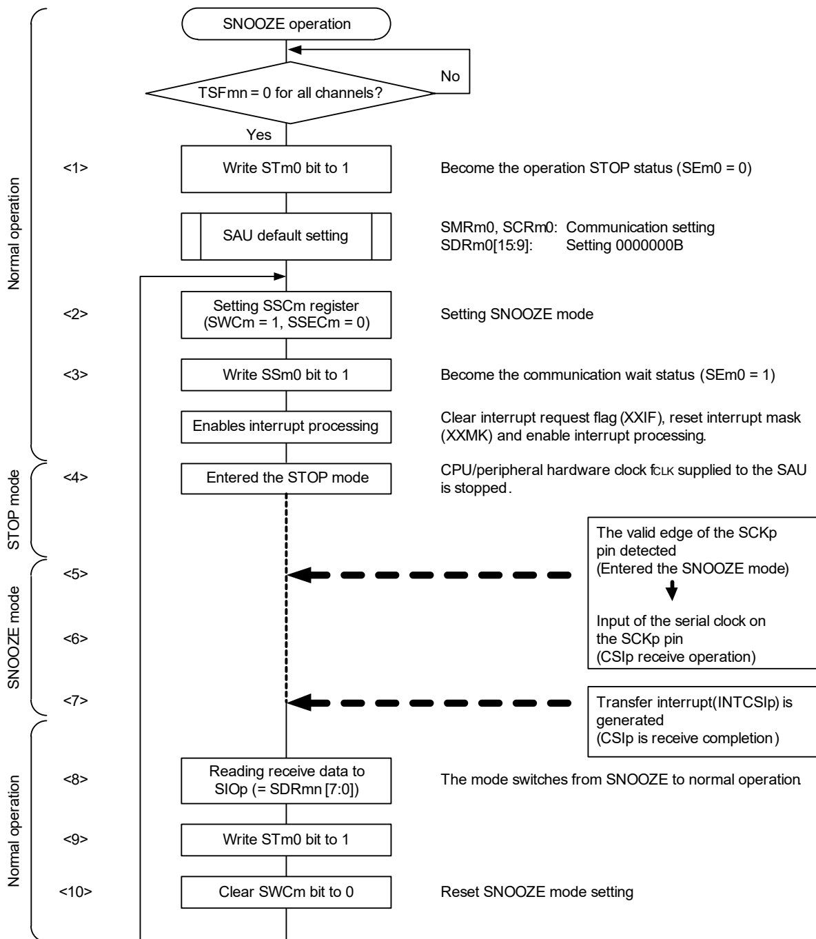
Figure 19 - 77 Flowchart of SNOOZE Mode Operation (continuous startup)
