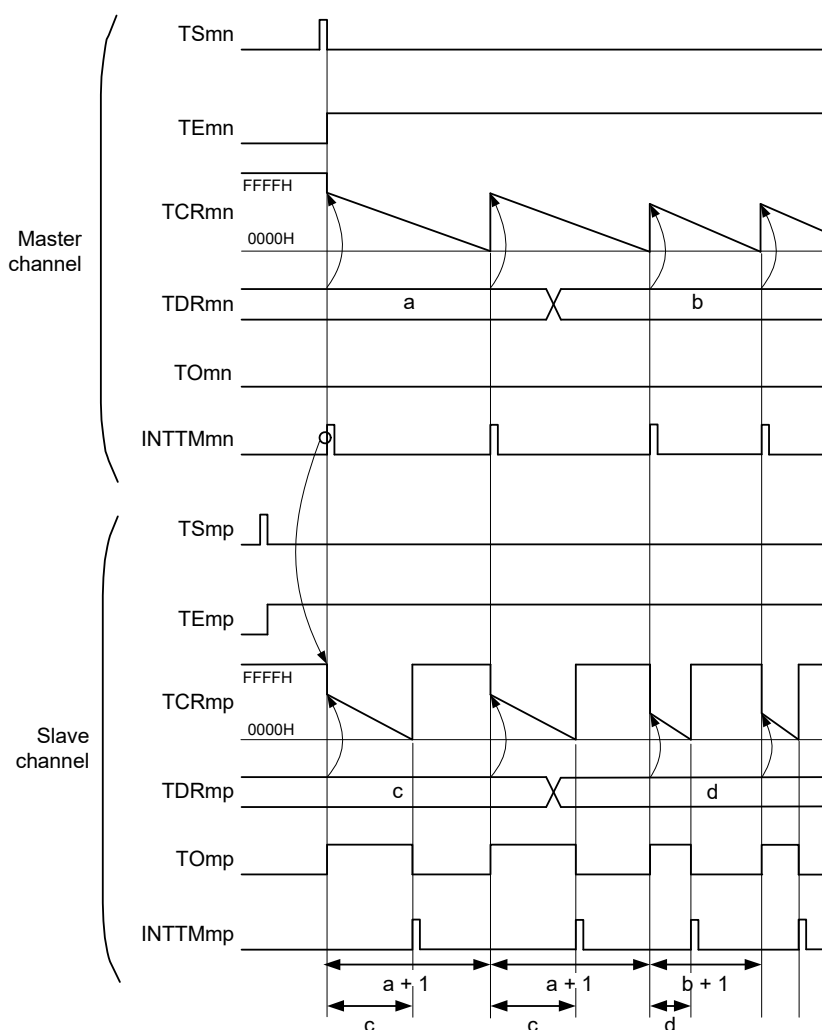
Figure 6 - 77 Example of Basic Timing of Operation as PWM Function
