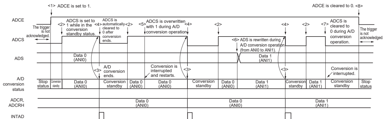
Figure 15 - 20 Example of Software Trigger Mode (Select Mode, One-Shot Conversion Mode) Operation Timing
