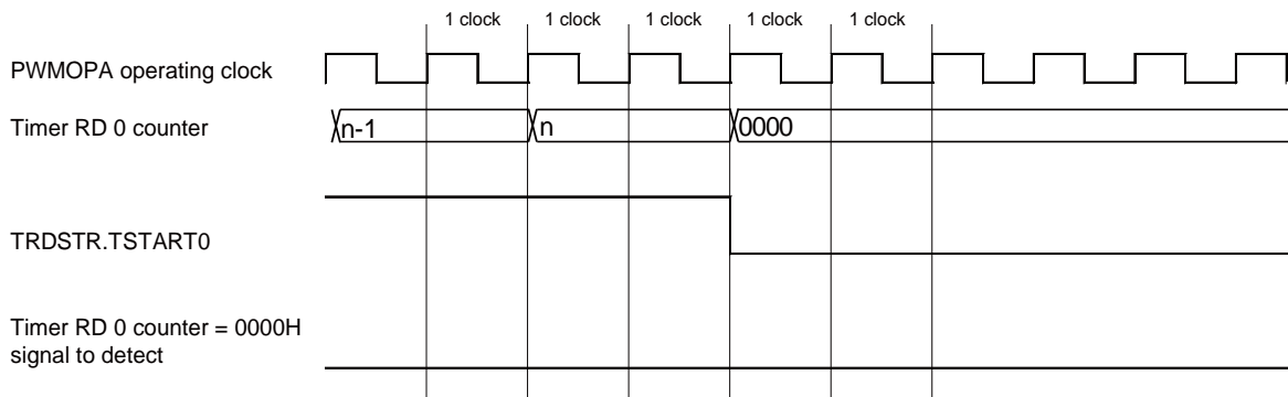
Figure 8 - 95 Judgment timing for count value = 0000H (count source = f_{CLK}/2 , count stops simultaneously when timer RD counter value becomes 0000H)
