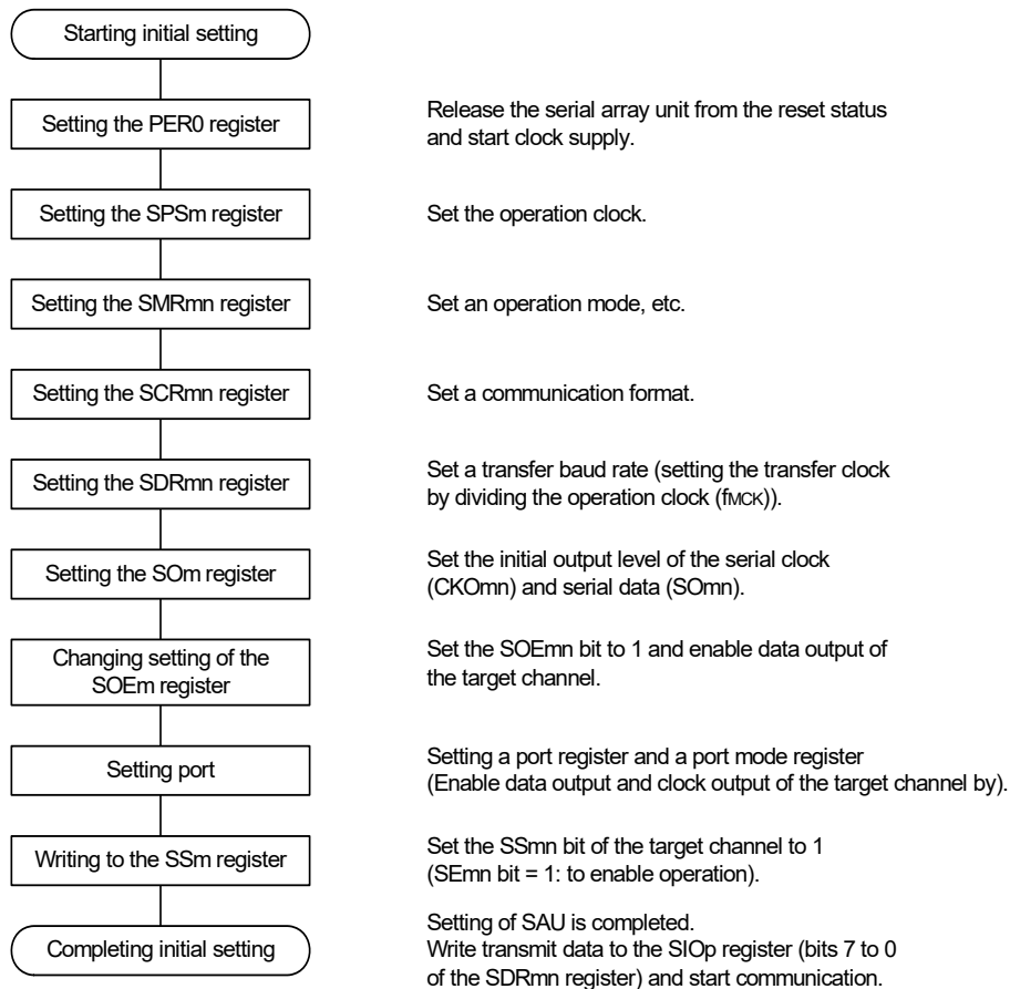
Figure 19 - 29 Initial Setting Procedure for Master Transmission
