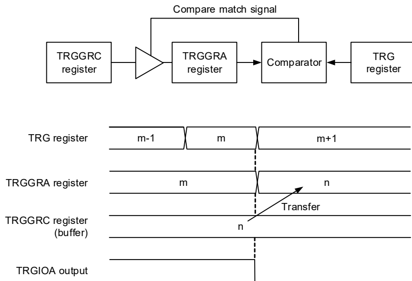
Figure 9 - 14 Buffer Operation for Output Compare Function
