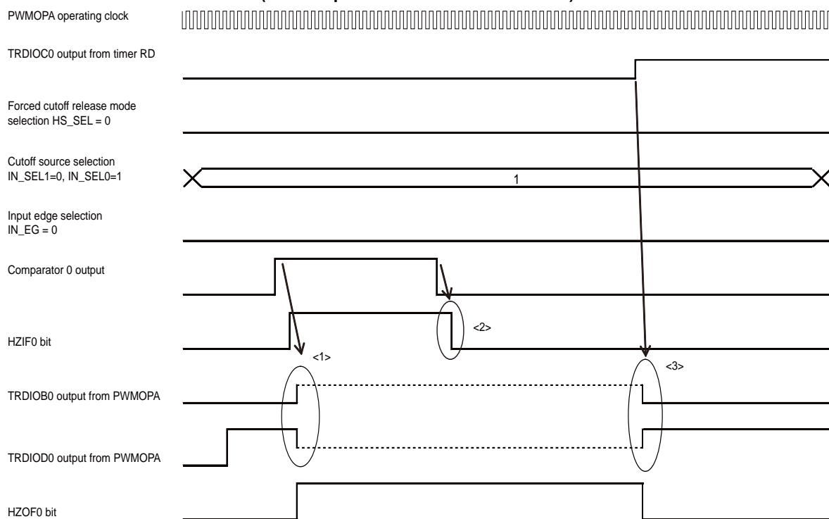
Figure 8 - 79 Operation example of hardware cutoff release function (an example of TRDIOB0 and TRDIOD0)
