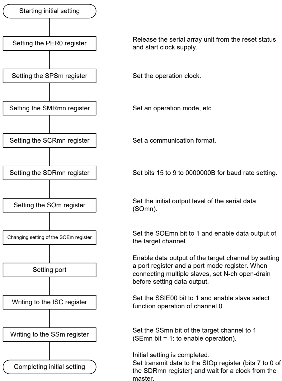
Figure 19 - 83 Initial Setting Procedure for Slave Transmission
