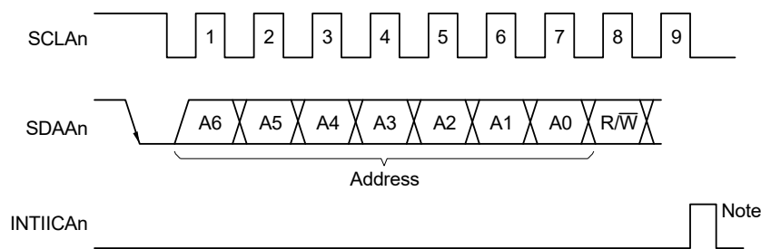
Figure 20 - 22 Address
