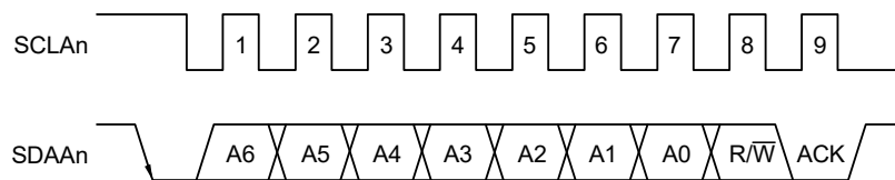
Figure 20 - 24 ACK
