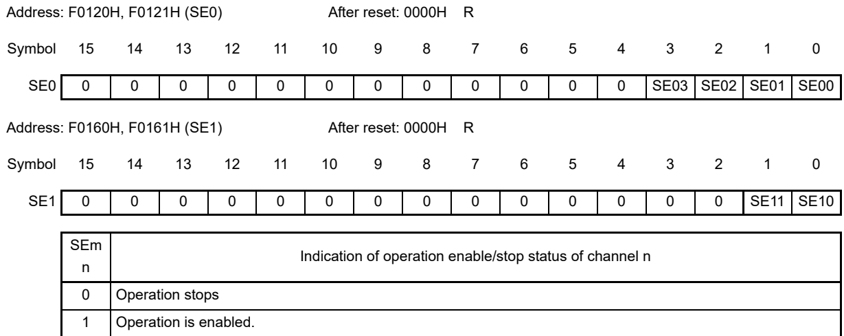
Figure 19 - 17 Format of Serial channel enable status register m (SEm)
