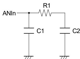
Figure 15 - 48 Internal Equivalent Circuit of ANIn Pin
