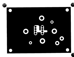
FIGURE 1C. BOTTOM LAYOUT
