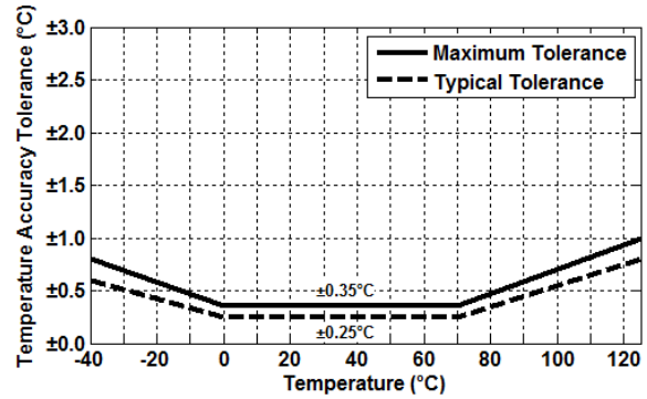
Figure 11. HS3003-MC1 Temperature Sensor Accuracy Tolerance
