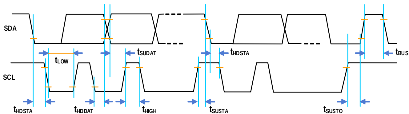
Figure 13. Timing Diagram
