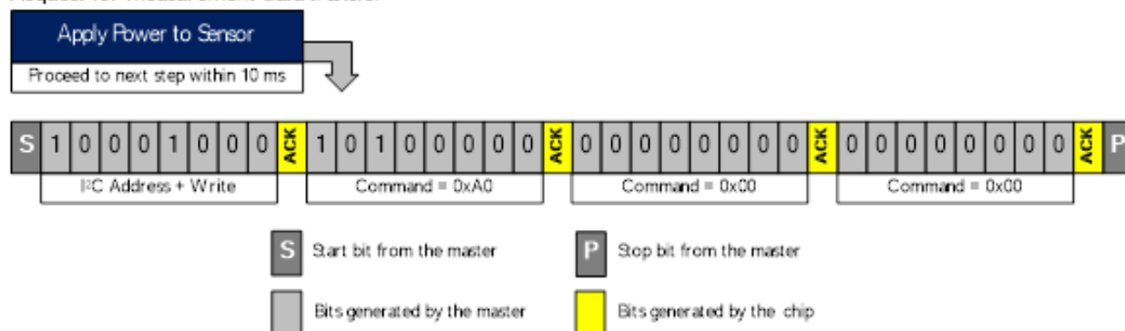
Figure 17. Sequence of Commands to Enter Programming Mode
