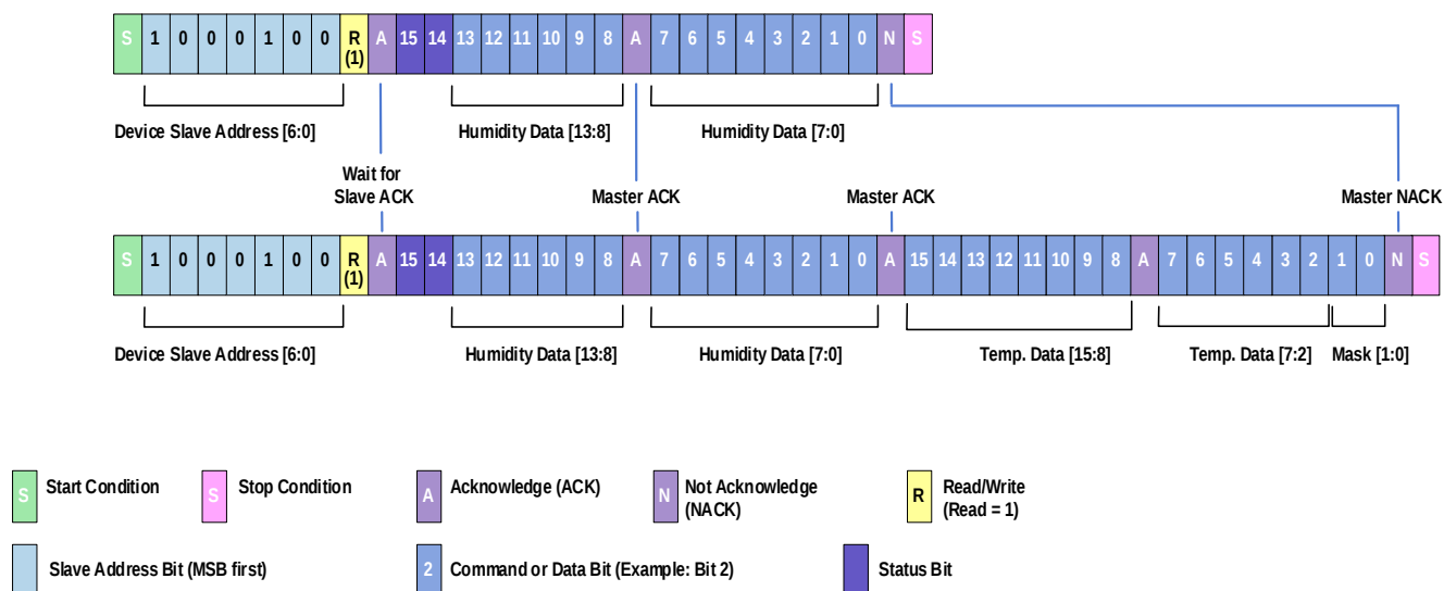
Figure 16. Data Fetch
