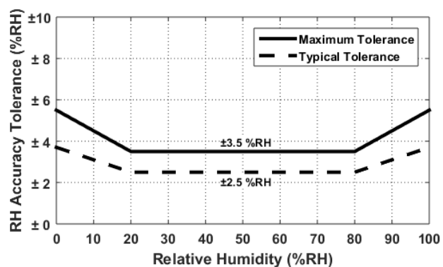
Figure 6. HS3003-MC1 RH Accuracy Tolerance at 25°C
