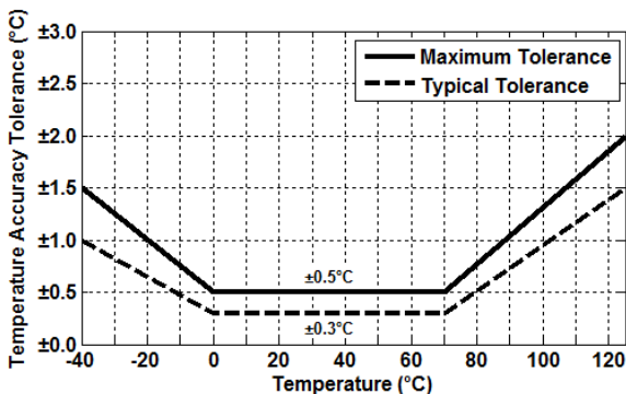
Figure 12. HS3004-MC1 Temperature Sensor Accuracy Tolerance
