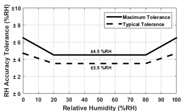
Figure 8. HS3004-MC1 RH Accuracy Tolerance at 25°C
