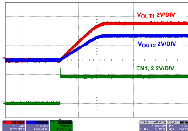
FIGURE 30. RATICMETRIC START-UP SEQUENCING AT NO LOAD
