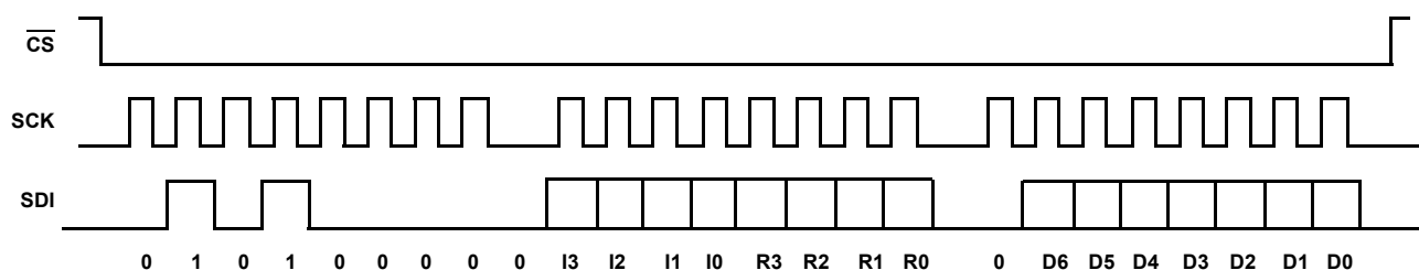
FIGURE 12. THREE BYTE WRITE SEQUENCE
