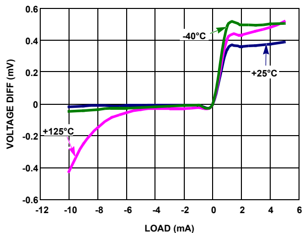
FIGURE 51. LOAD REGULATION
