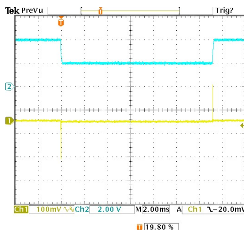
FIGURE 12. LOAD TRANSIENT RESPONSE, 1nF LOAD CAPACITANCE
