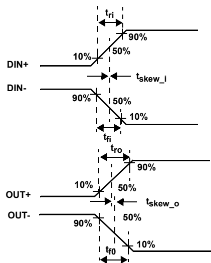
FIGURE 7A. MEASUREMENT POINTS
