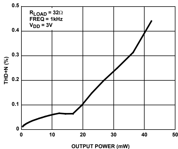
FIGURE 13. THD+N vs OUTPUT POWER
