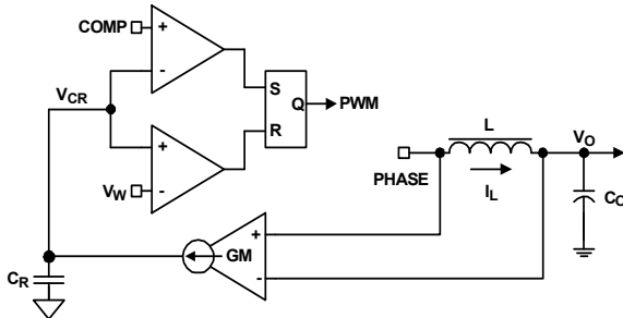
Figure 44. R3 Modulator
