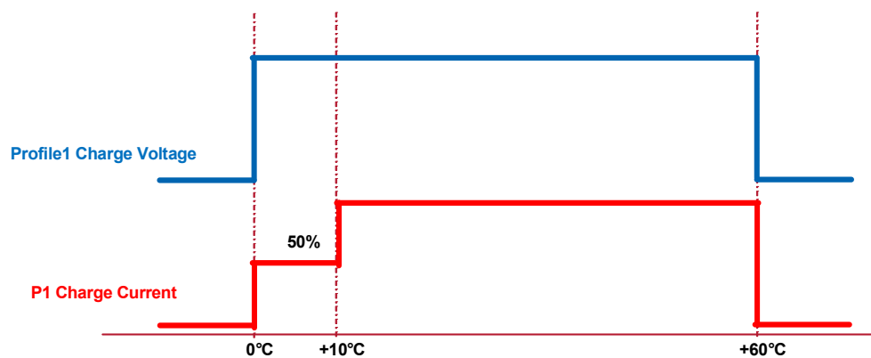
Figure 33. JEITA Profile 1
