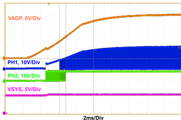
Figure 10. Adapter Voltage Ramp Up, Boost --&gt; Buck_Boost --&gt; Buck Operation Mode Transition
