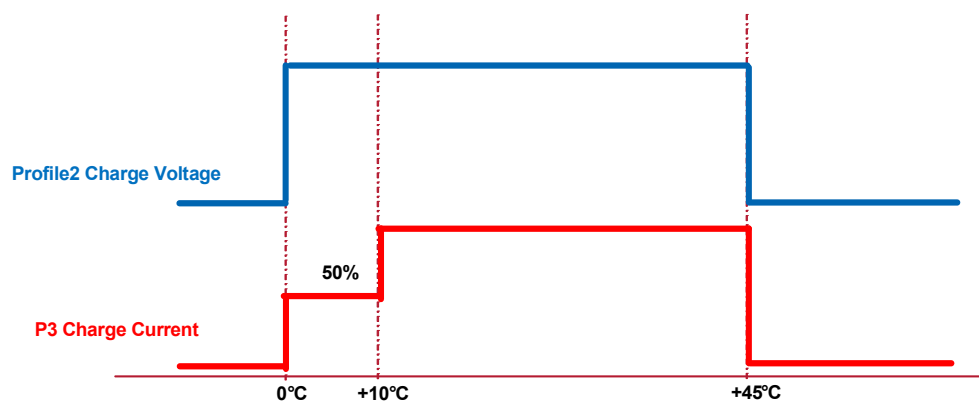
Figure 34. JEITA Profile 2
