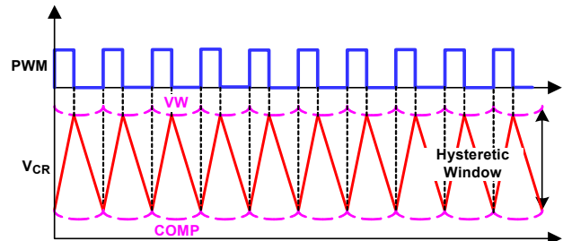
Figure 45. R3 Modulator Operation Principles in Steady State
