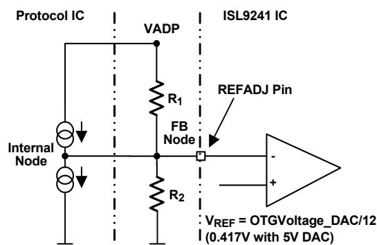
Figure 39. Simplified REFADJ Application
