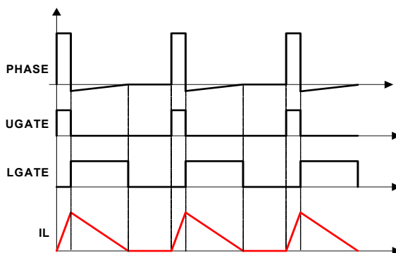
Figure 47. Diode Emulation
