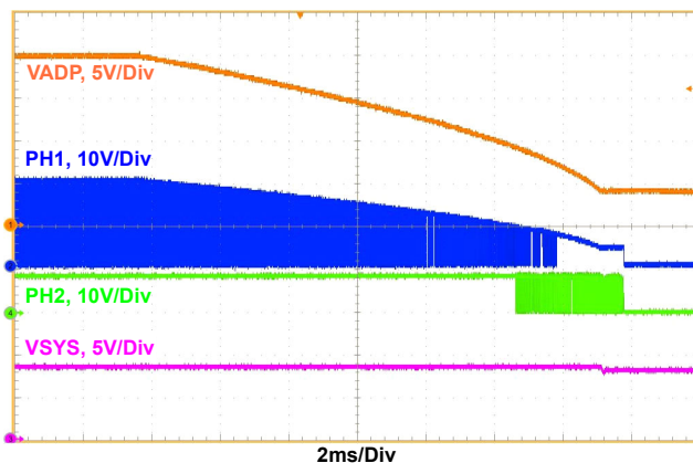
Figure 11. Adapter Voltage Ramp Down, Buck --&gt; Buck_Boost --&gt; Boost Operation Mode Transition
