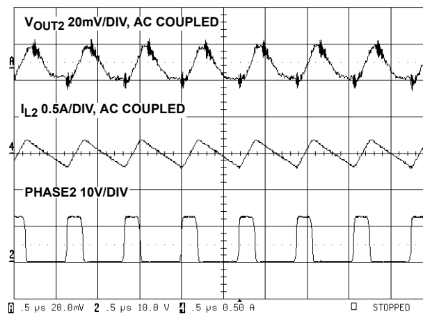
FIGURE 6. PWM2 WAVEFORMS
