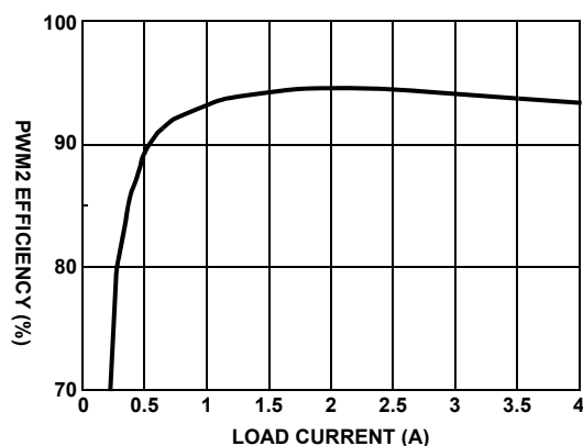
FIGURE 12. PWM2 EFFICIENCY vs LOAD, VIN=5V, VOUT=3.3V
