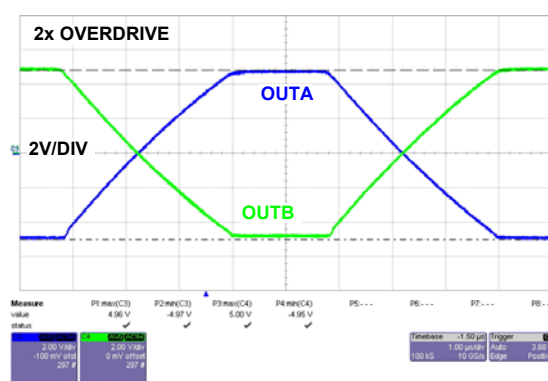
FIGURE 30. OVERDRIVE RECOVERY
