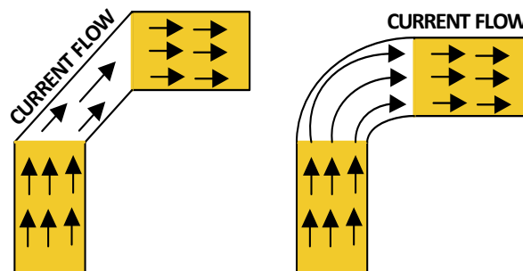
FIGURE 87. USE ARCS AND 45° TRACES TO SAFELY ROUTE TRACES WITH LARGE CURRENT FLOWS
