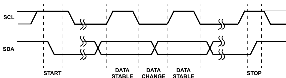
FIGURE 71. VALID DATA CHANGES, START AND STOP CONDITIONS
