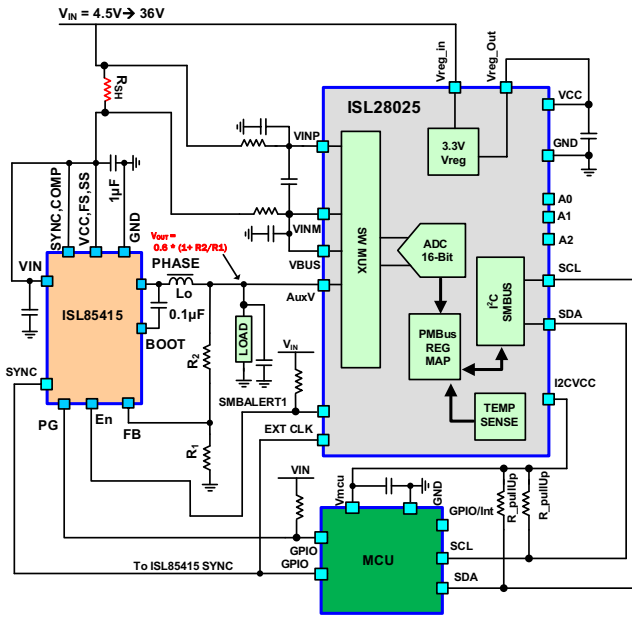
FIGURE 78. SIMPLIFIED SCHEMATIC OF THE ISL28025 SYNCHRONIZED TO A MCU SYSTEM CLOCK
