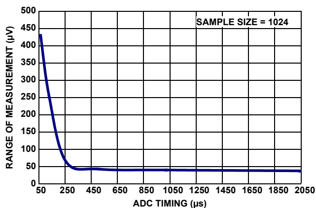
FIGURE 60. PRIMARY SHUNT STABILITY: RANGE vs ACQUISITION TIME
