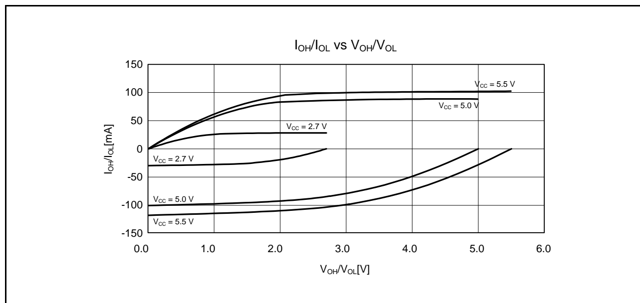
Figure 35.8 V_{OH}/V_{OL} and I_{OH}/I_{OL} Voltage Characteristics at T_a = 25^\circ\text{C} When Normal Output is Selected (Reference Data)
