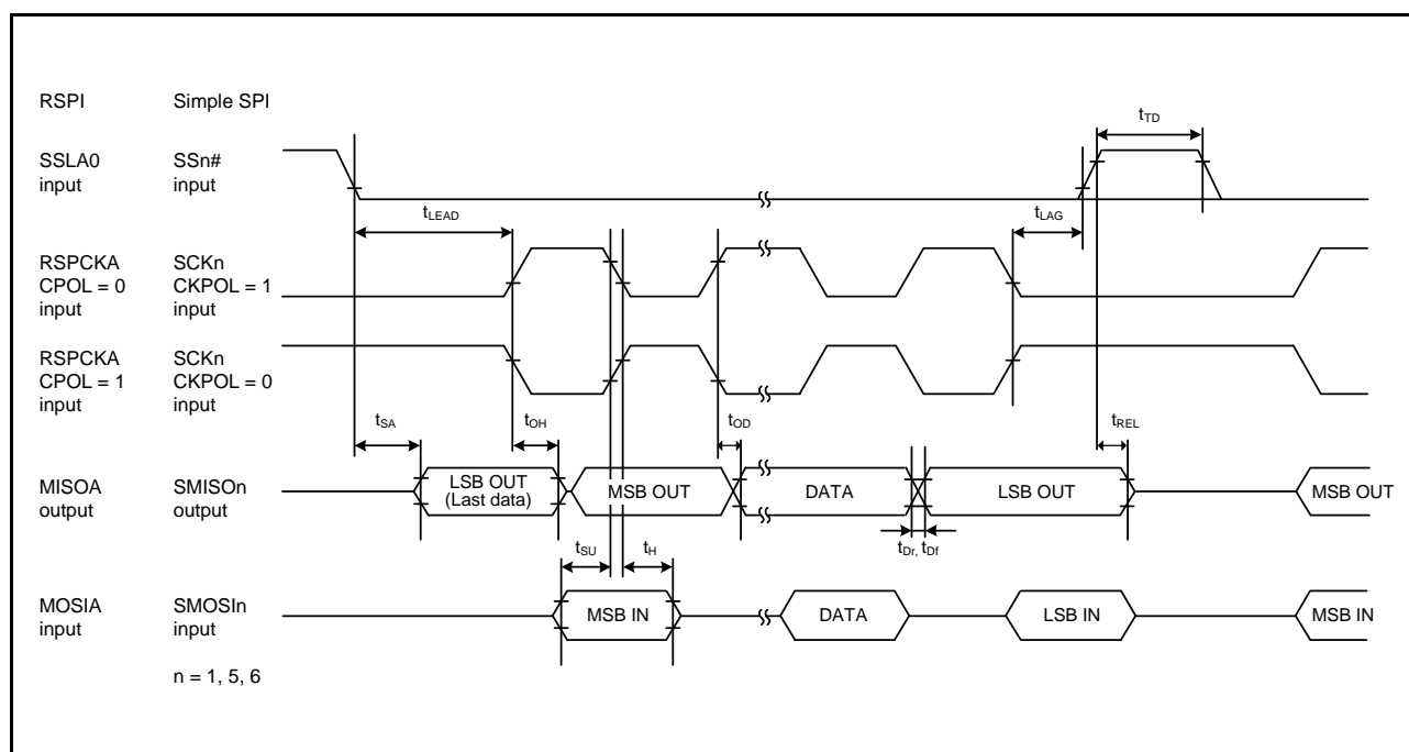
Figure 35.44 RSPI Timing (Slave, CPHA = 1) and Simple SPI Clock Timing (Slave, CKPH = 0)
