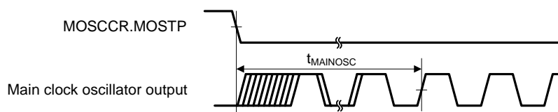
Figure 35.21 Main Clock Oscillation Start Timing
