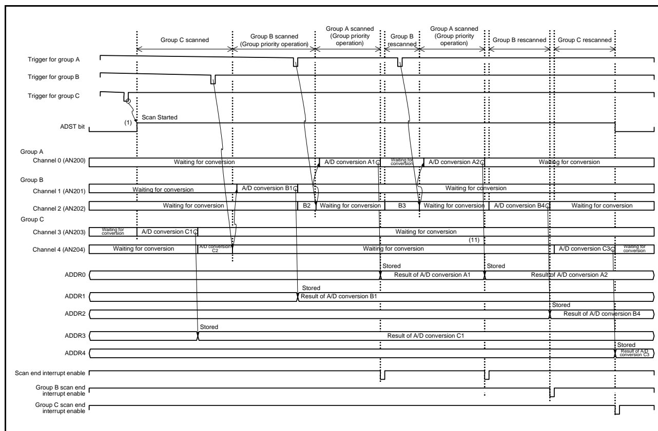
Figure 29.25 Example 2 of Group Priority Operation: Priority Group Trigger Input during Low-Priority Group Rescan, With Rescan Setting (ADGSPCR.GBRSCN = 1, ADGSPCR.GBRP = 0, ADGSPCR.LGRRS = 1)
