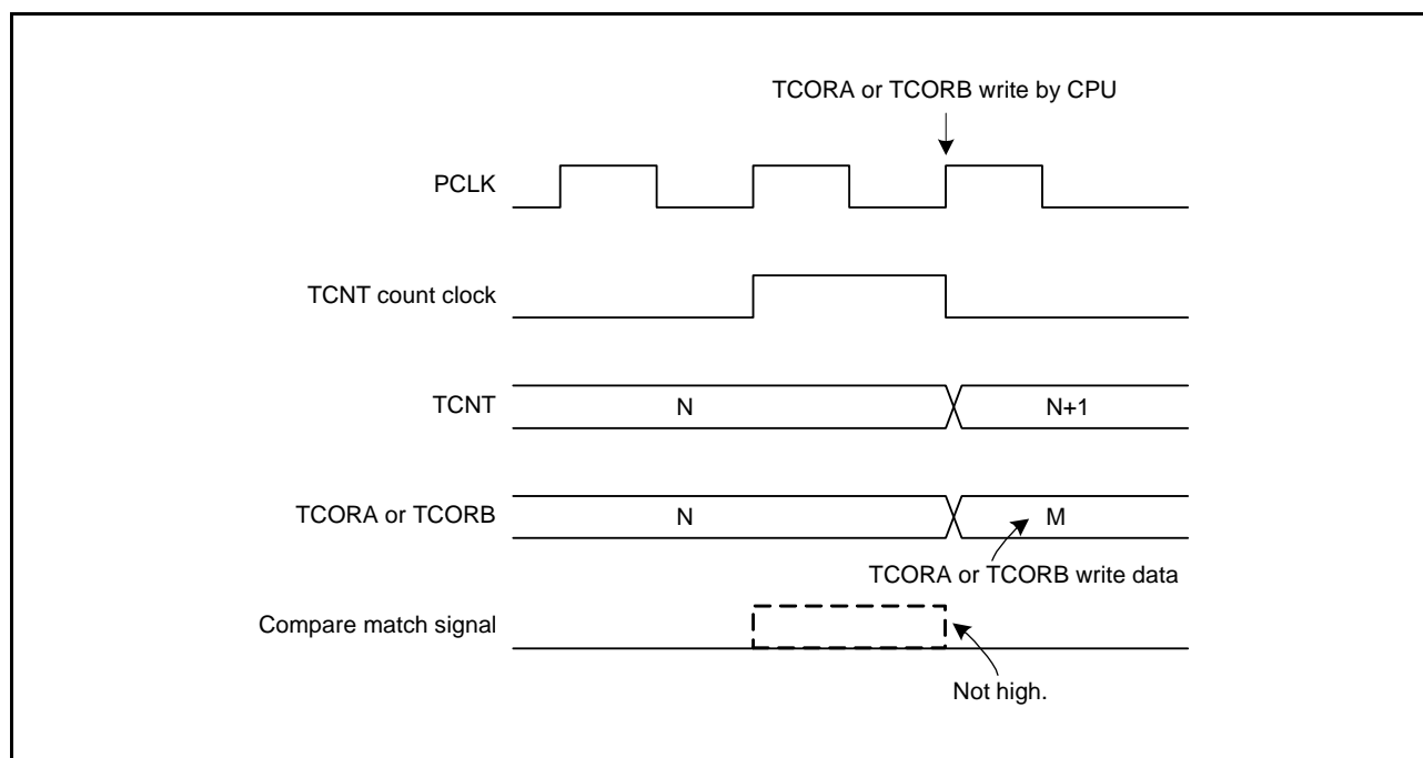
Figure 22.17 Conflict between TCORA or TCORB Write and Compare Match
