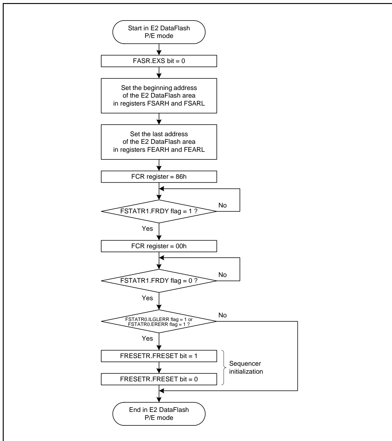
Figure 34.17 Procedure to Issue the All-Block Erase Command for the E2 DataFlash
