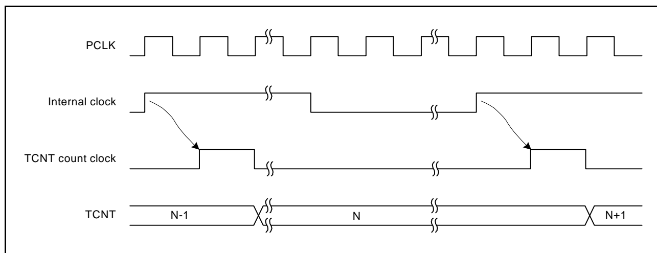
Figure 22.7 Count Timing for Internal Clock
