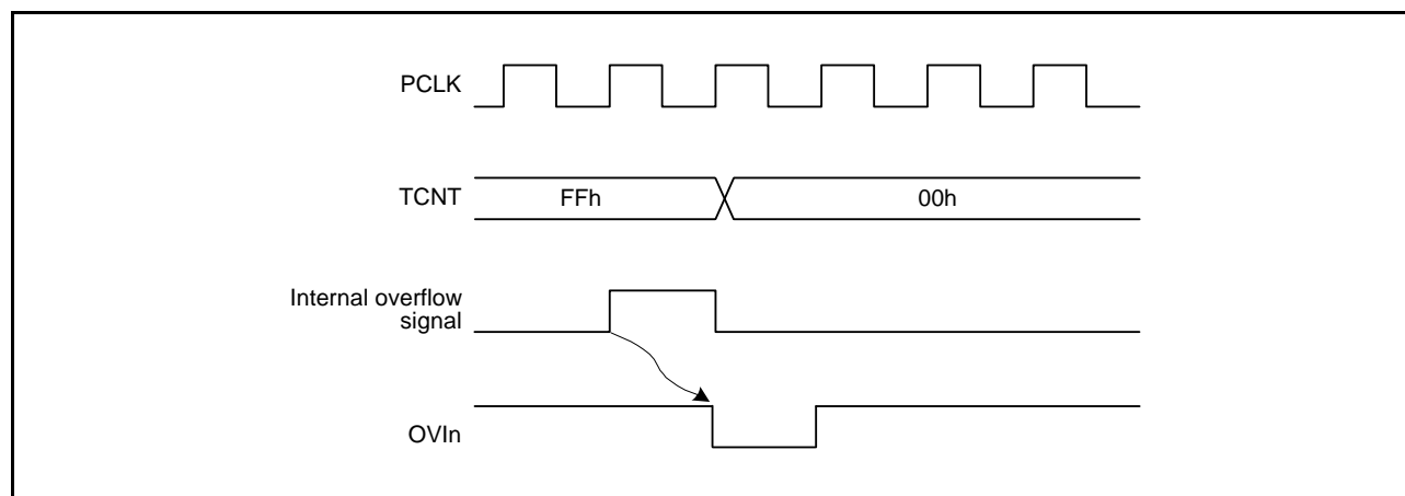
Figure 22.14 Timing of Overflow Interrupt Flag Setting to 1 (n = 0 to 7)
