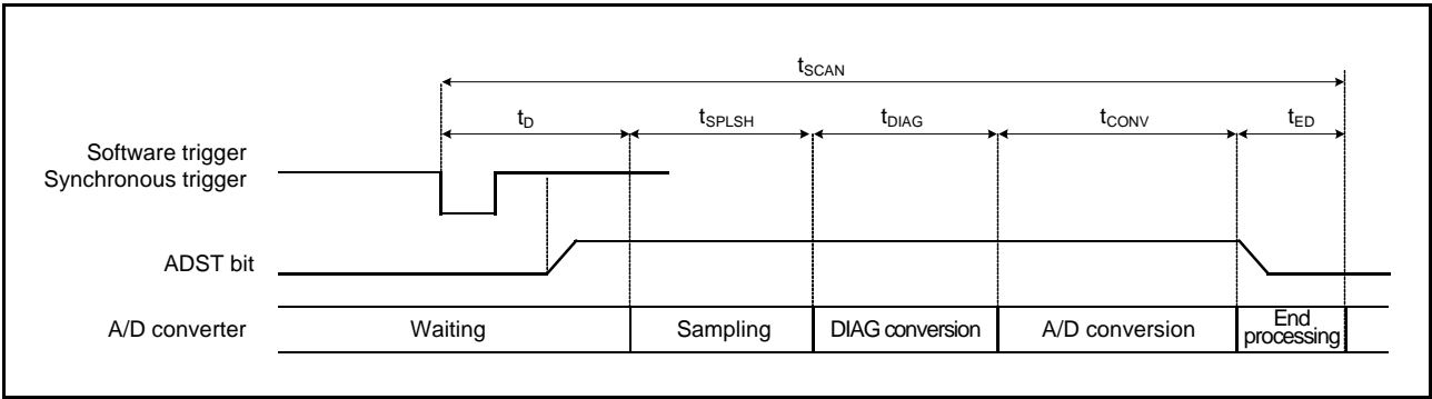
Figure 29.29 Scan Conversion Timing (Activated by Software or Synchronous Trigger)
