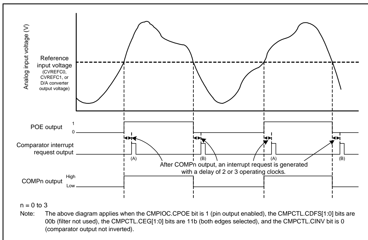
Figure 31.2 Comparator Operation Example
