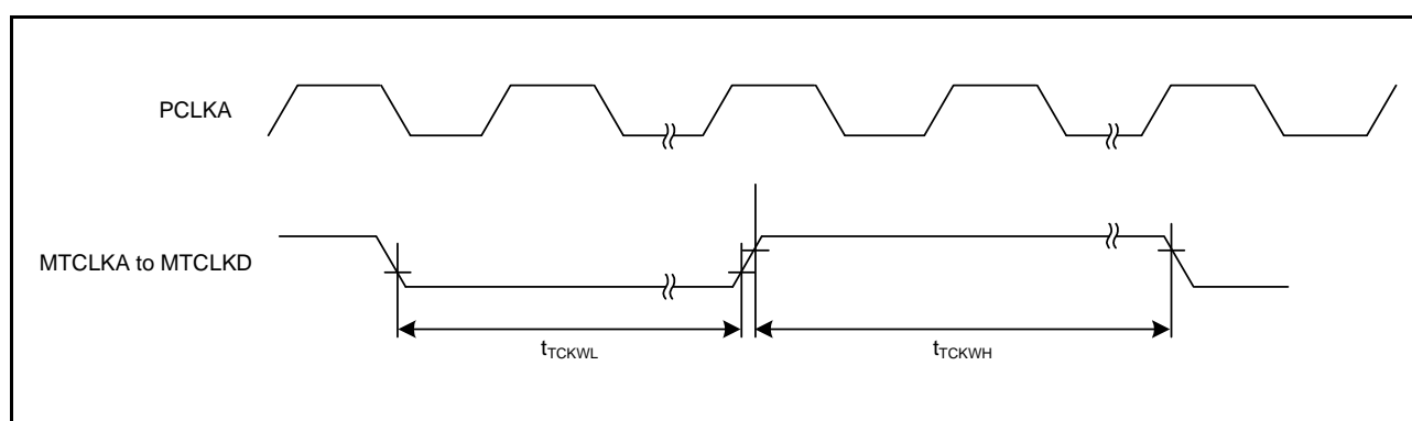
Figure 35.34 MTU3 Clock Input Timing
