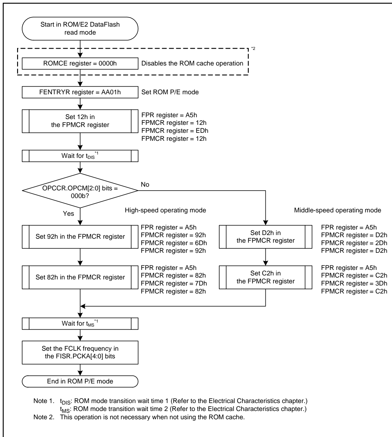
Figure 34.8 Procedure for Transition from ROM/E2 DataFlash Read Mode to ROM P/E Mode
