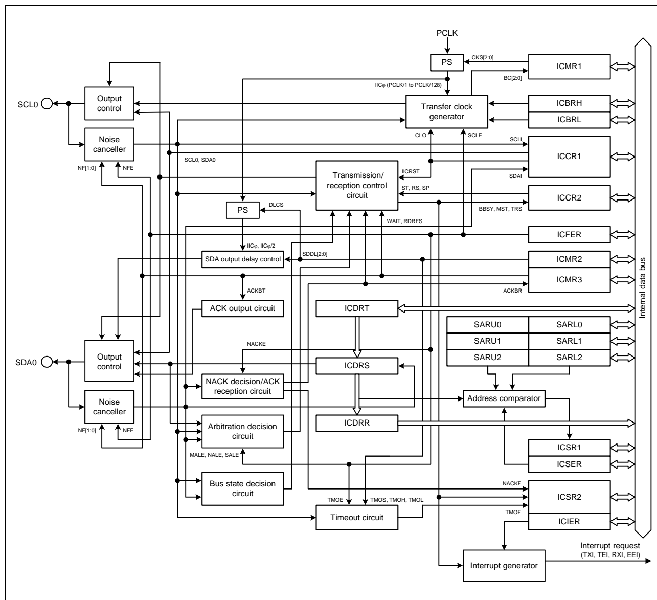
Figure 26.1 RIIC Block Diagram
