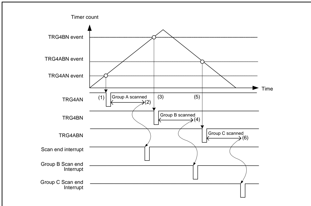
Figure 29.16 Example of Operation in Group Scan Mode (Basic Operation: Synchronous Triggers from MTU Used)
