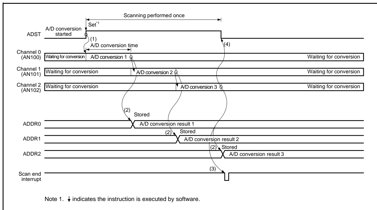
Figure 29.5 Example of Operation in Single Scan Mode (Basic Operation: AN100, AN101, AN102 Selected)
