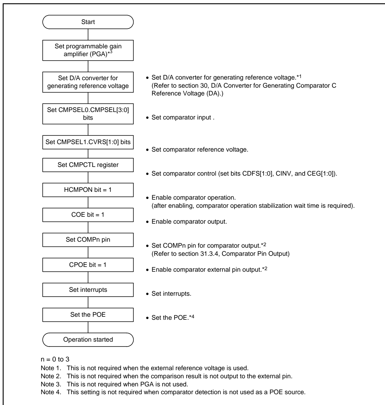
Figure 31.5 Comparator Operation Setting Flowchart
