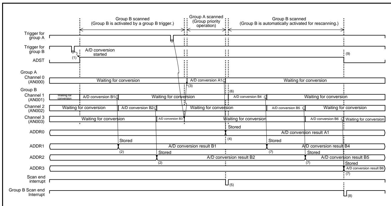
Figure 29.19 Example 1 of Group Priority Operation: Group A Trigger Input during Group B Scan, With Rescan Setting (ADGSPCR.GBRSCN = 1, ADGSPCR.GBRP = 0, ADGSPCR.LGRRS = 0)
