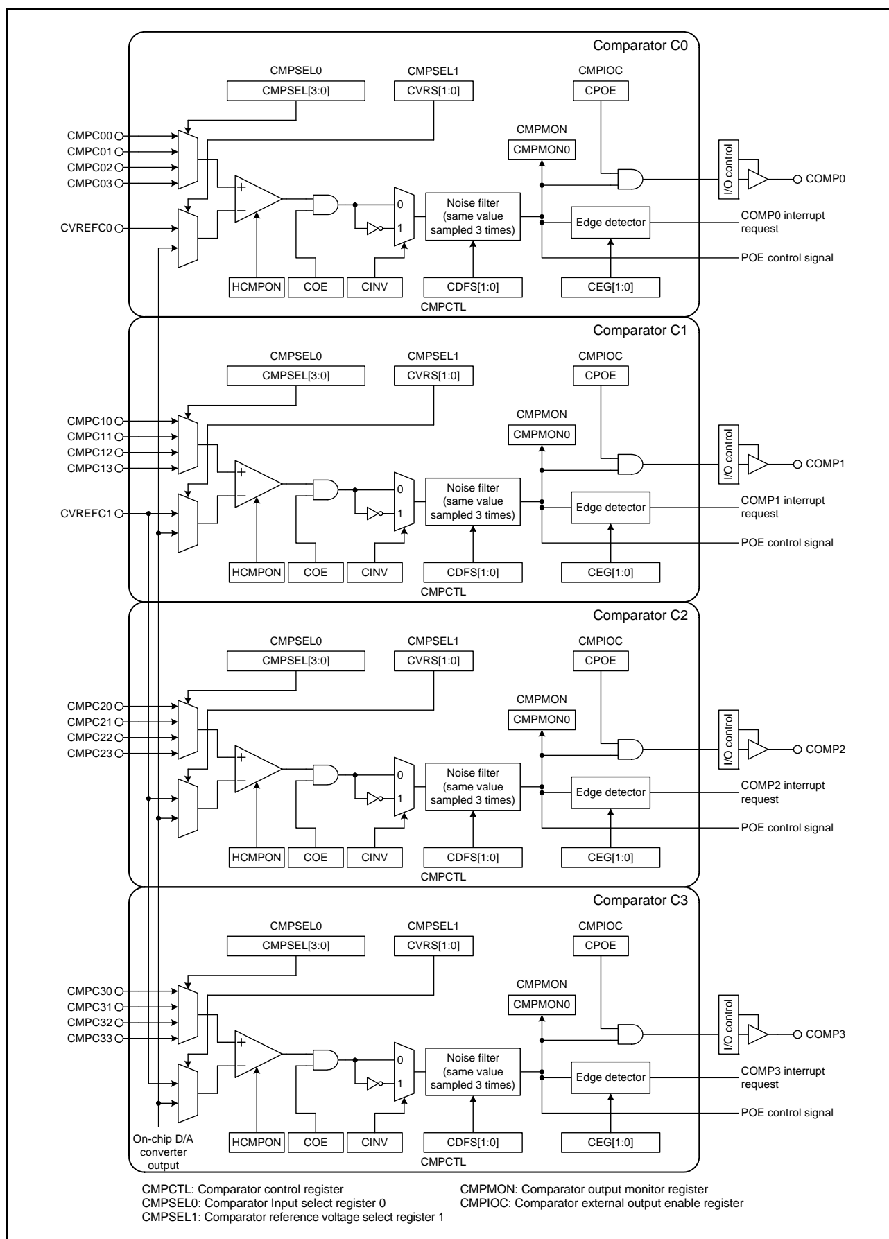
Figure 31.1 Comparator C Block Diagram
