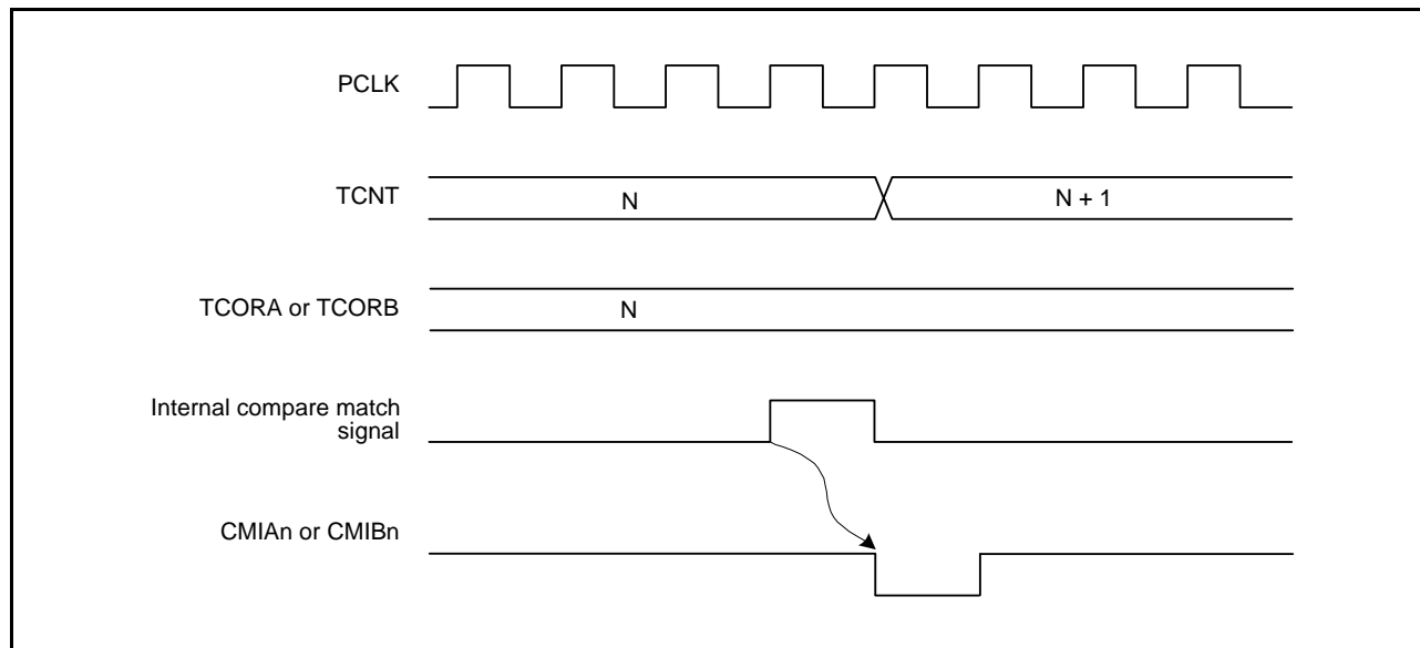
Figure 22.9 Timing of Interrupt Flag Setting to 1 at Compare Match ( n = 0 to 7)
