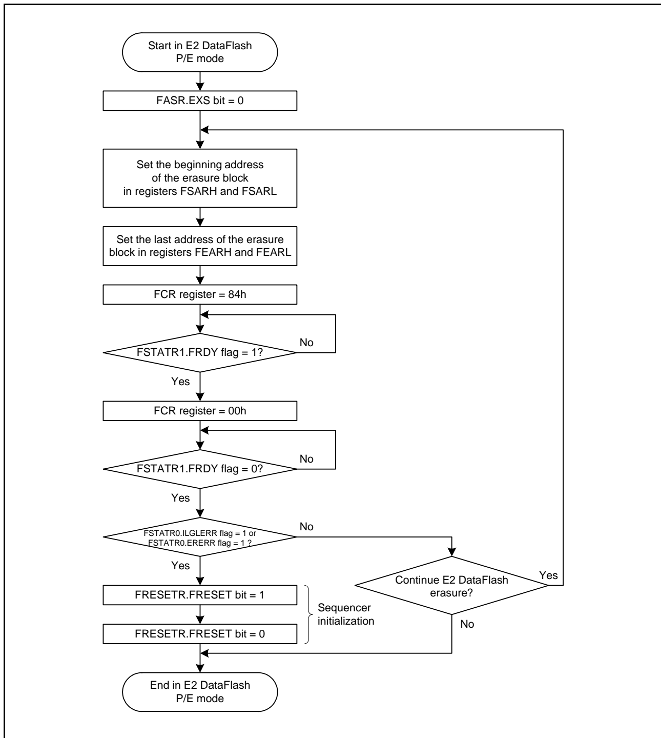
Figure 34.15 Procedure to Issue the Block Erase Command for the E2 DataFlash
