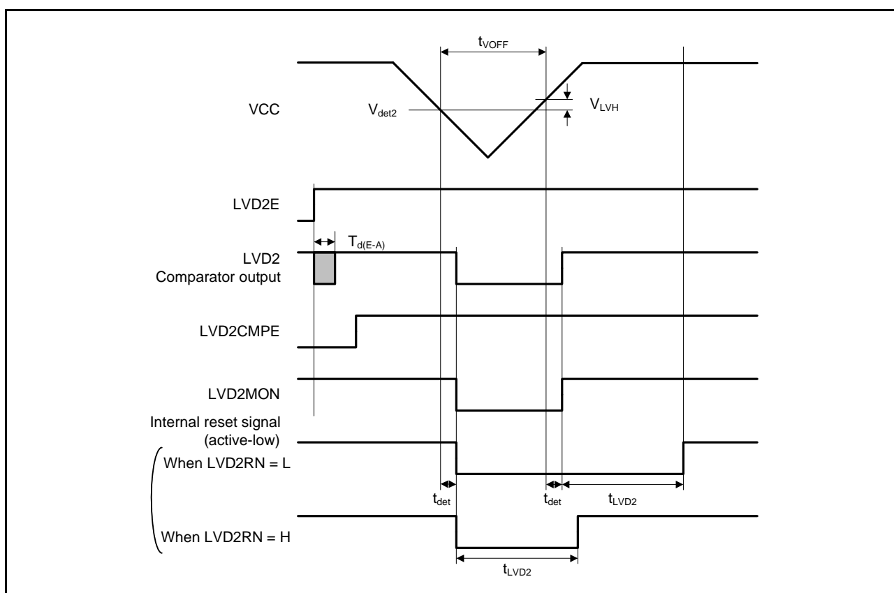
Figure 35.52 Voltage Detection Circuit Timing ( V_{det2} )
