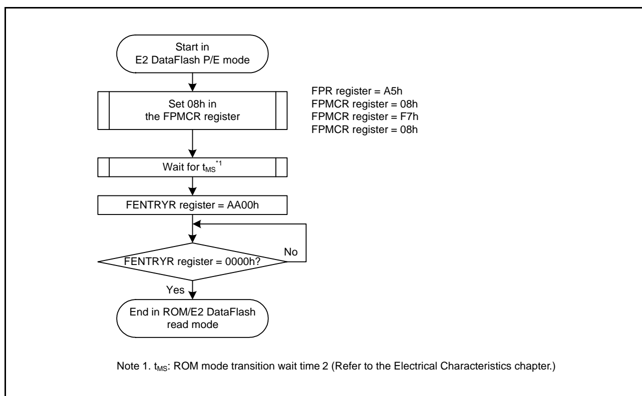
Figure 34.11 Procedure for Transition from E2 DataFlash P/E Mode to ROM/E2 DataFlash Read Mode
