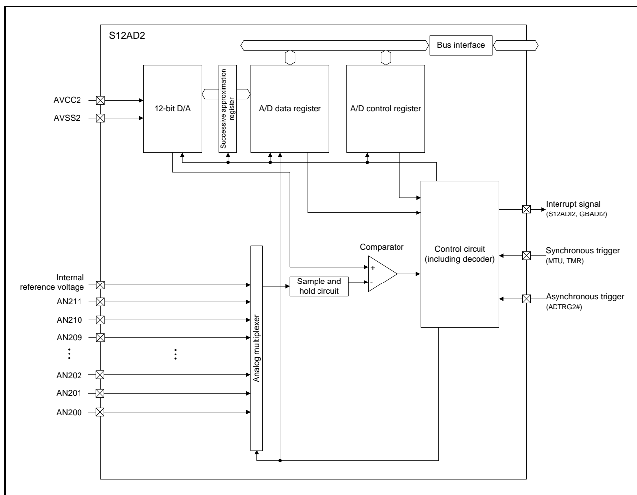
Figure 29.3 Block Diagram of 12-Bit A/D Converter (Unit 2)
