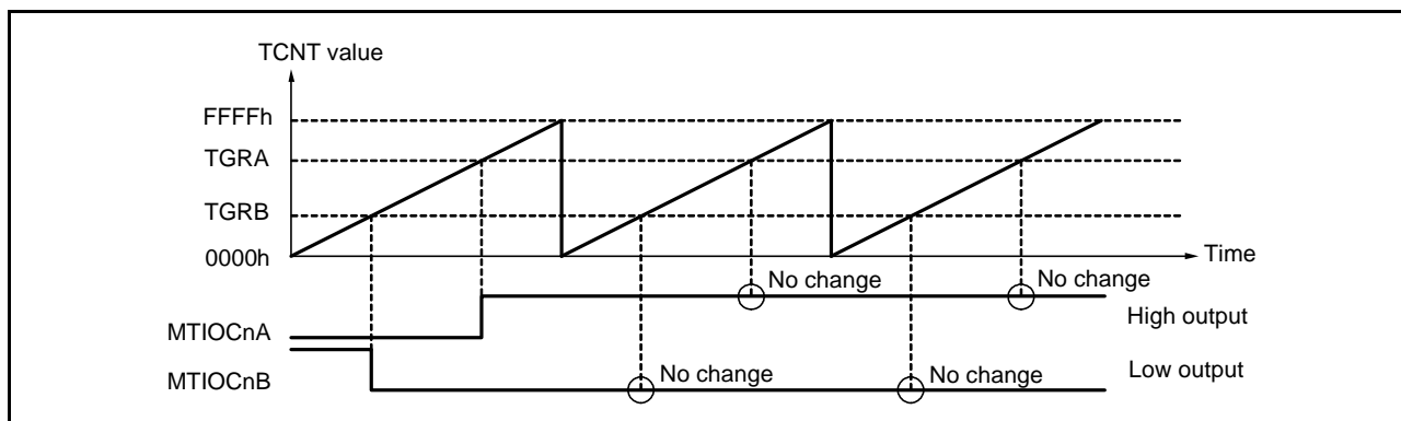
Figure 20.9 Example of low output and high output Operation (n = 0 to 4, 6, 7, 9)
