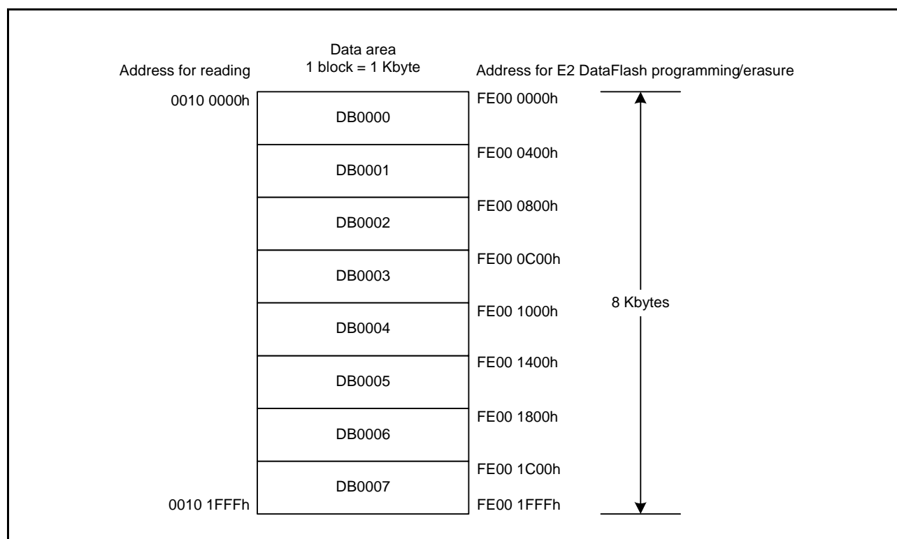
Figure 34.2 E2 DataFlash Area and Block Configuration
