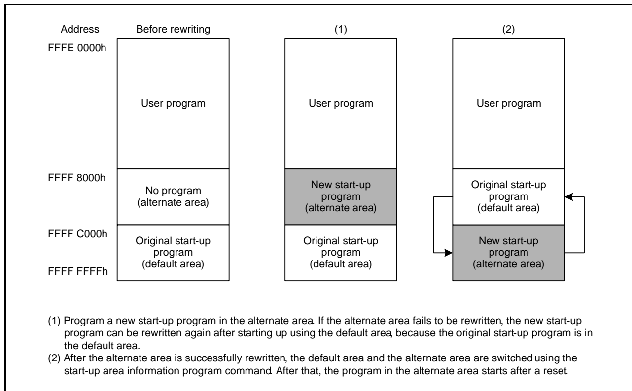
Figure 34.4 Overview of the Start-Up Program Protection
