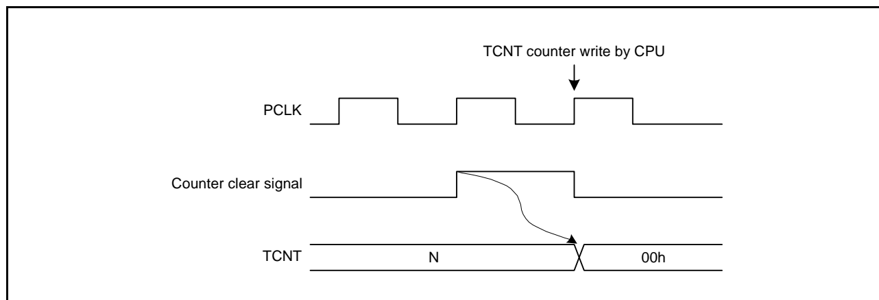
Figure 22.15 Conflict between TCNT Write and Counter Clear
