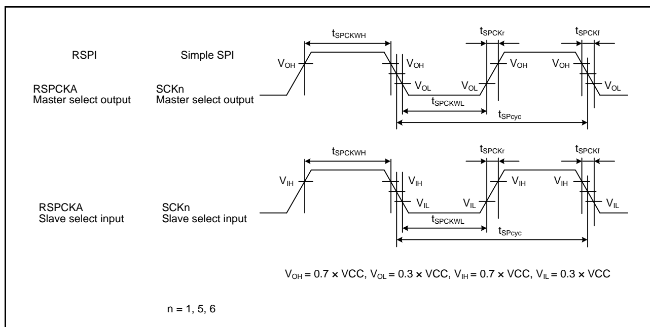
Figure 35.40 RSPI Clock Timing and Simple SPI Clock Timing
