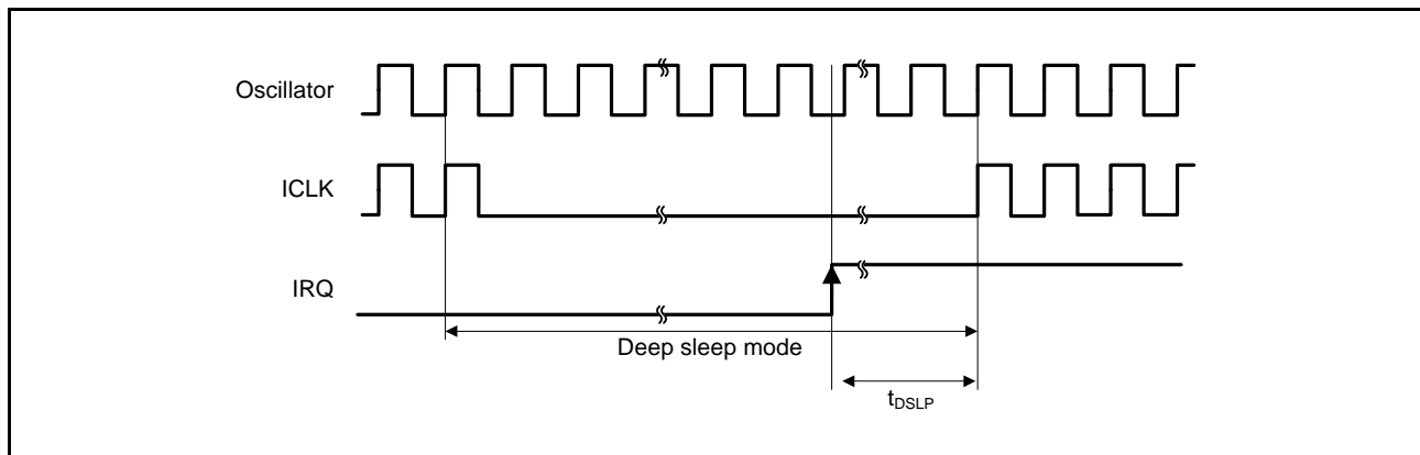
Figure 35.29 Deep Sleep Mode Recovery Timing
