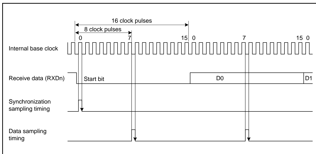
Figure 25.5 Receive Data Sampling Timing in Asynchronous Mode
