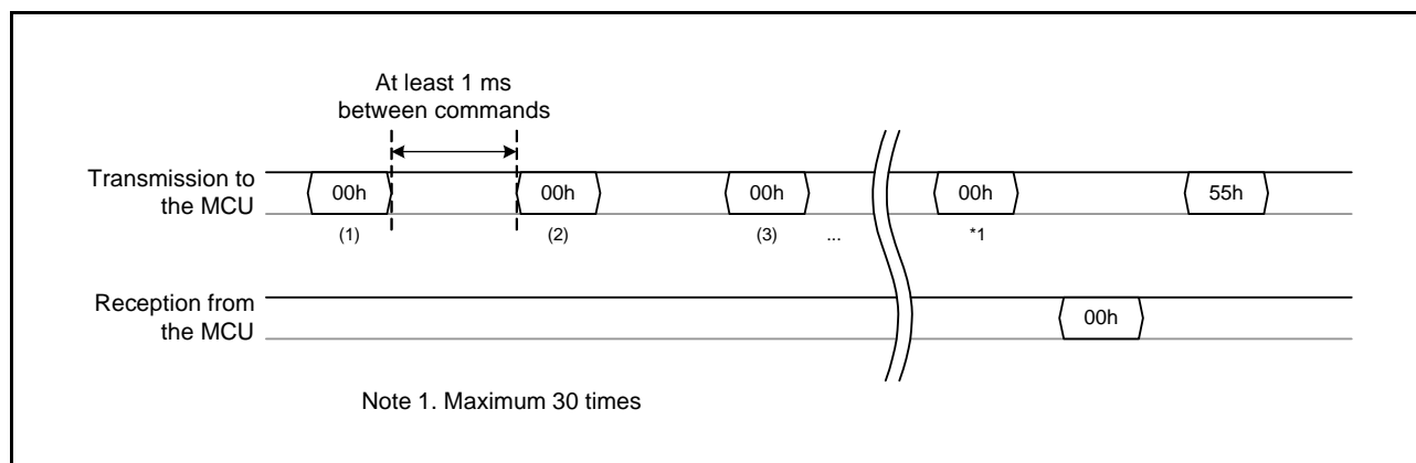
Figure 34.30 Transmit/Receive Data for Bit Rate Automatic Adjustment
