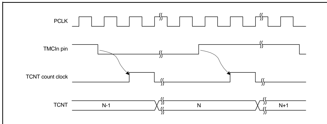
Figure 22.8 Count Timing for External Clock (at Both Edges)
