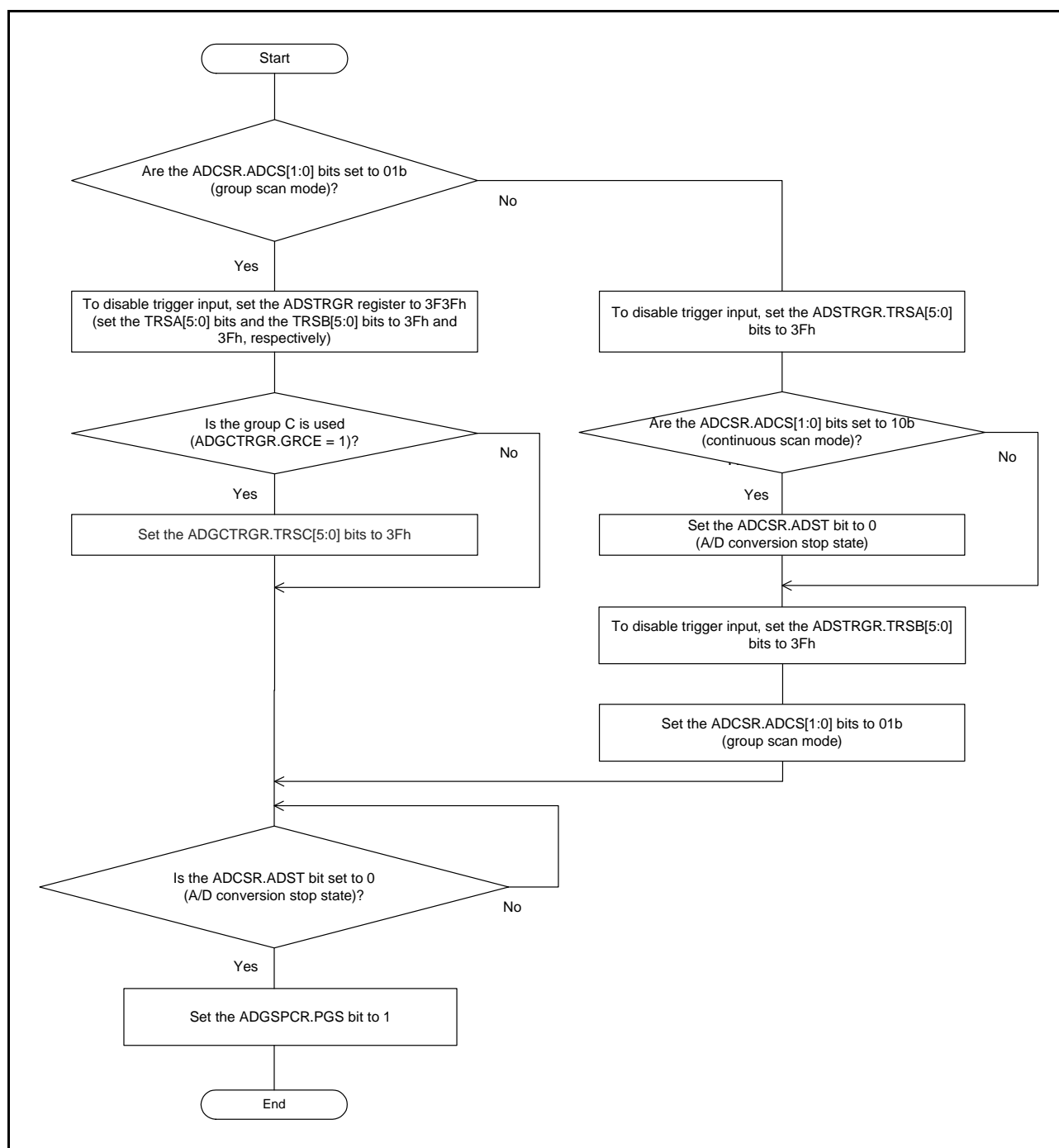
Figure 29.18 Flow of Setting the ADGSPCR.PGS Bit
