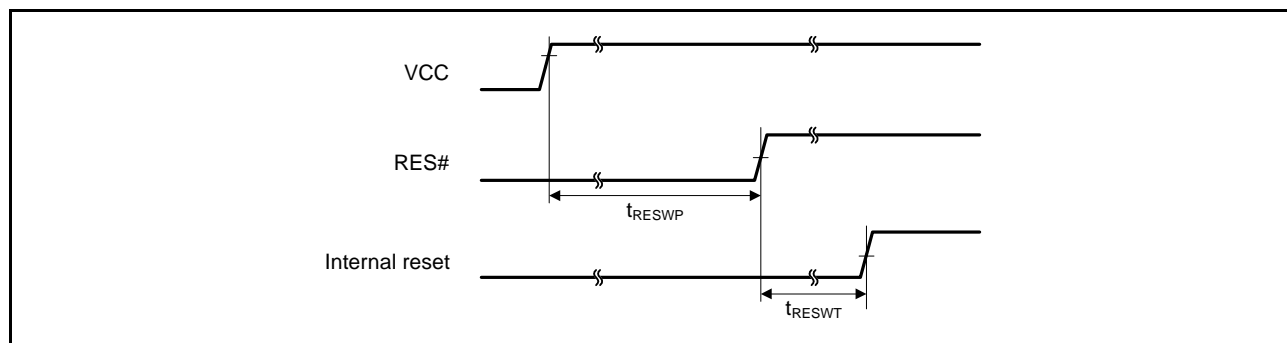
Figure 35.25 Reset Input Timing at Power-On
