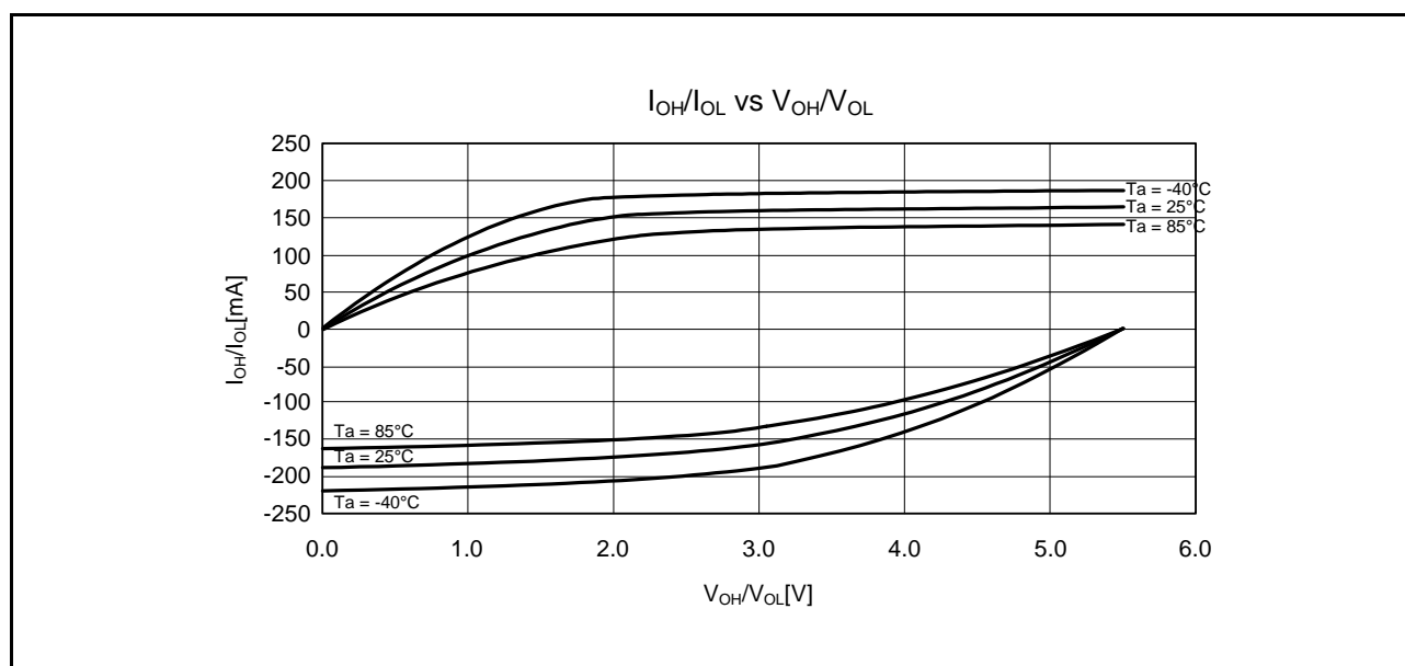
Figure 35.15 V_{OH}/V_{OL} and I_{OH}/I_{OL} Temperature Characteristics of Large Current Ports at V_{CC} = 5.5 V (Reference Data)
