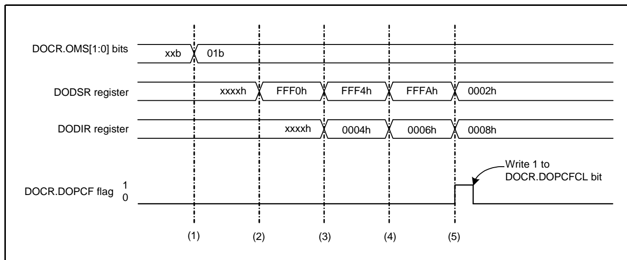
Figure 32.3 Example of Operation in Data Addition Mode
