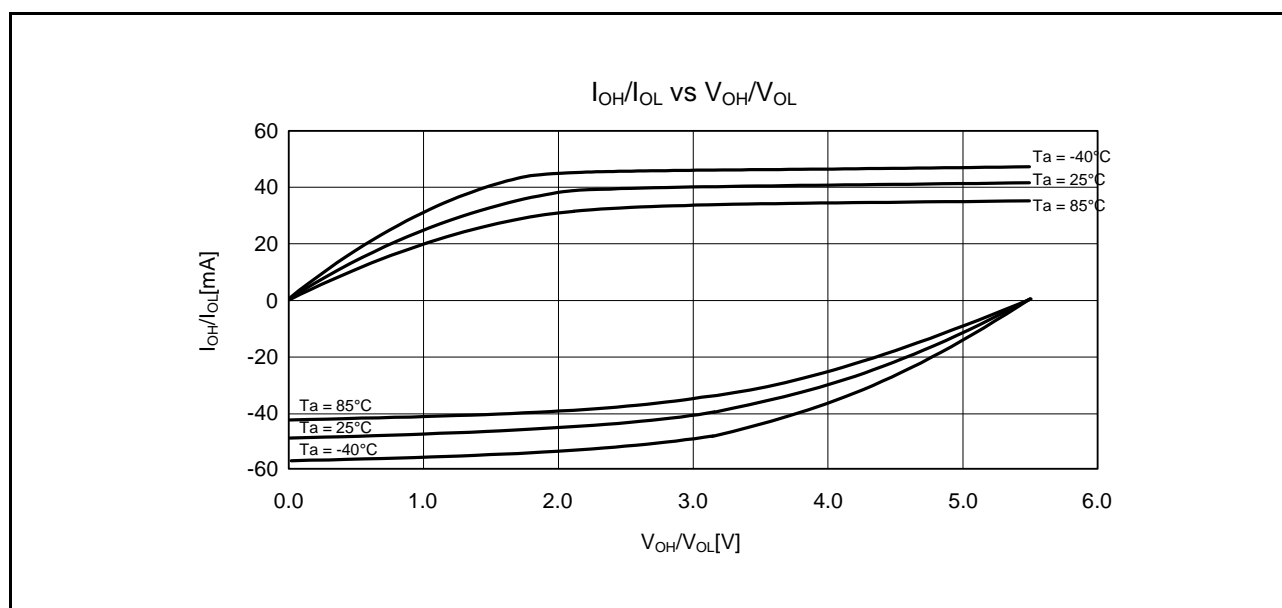
Figure 35.7 V_{OH}/V_{OL} and I_{OH}/I_{OL} Temperature Characteristics at V_{CC} = 5.5 V when Normal Output is Selected (Reference Data)
