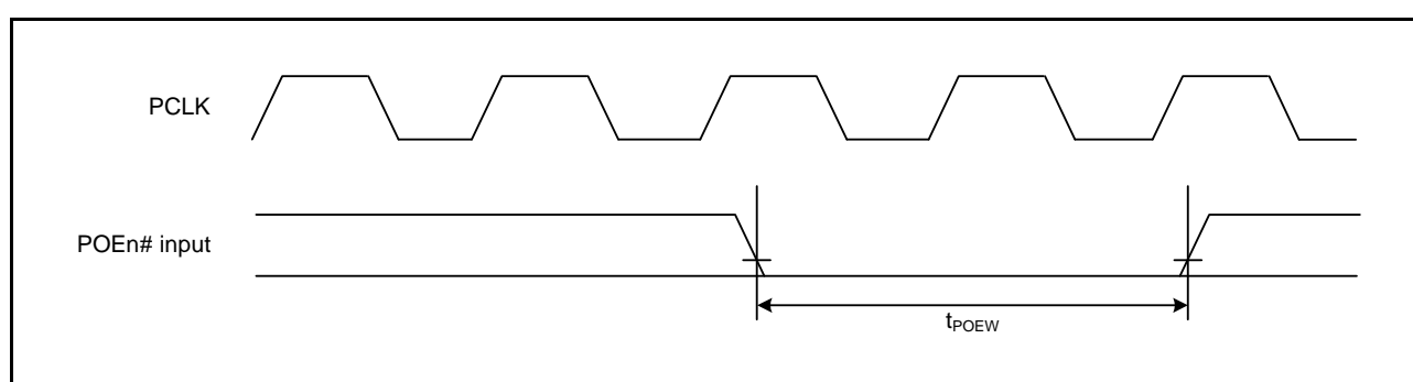
Figure 35.35 POE# Input Timing
