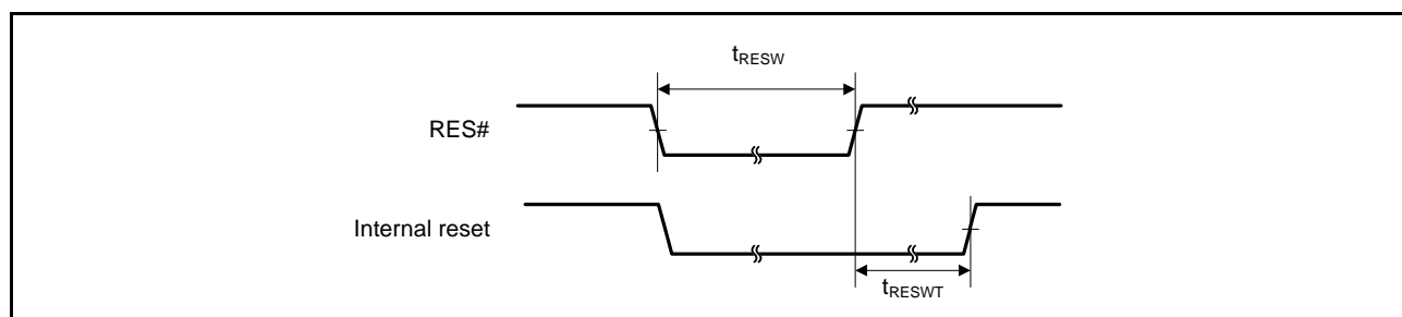
Figure 35.26 Reset Input Timing (1)
