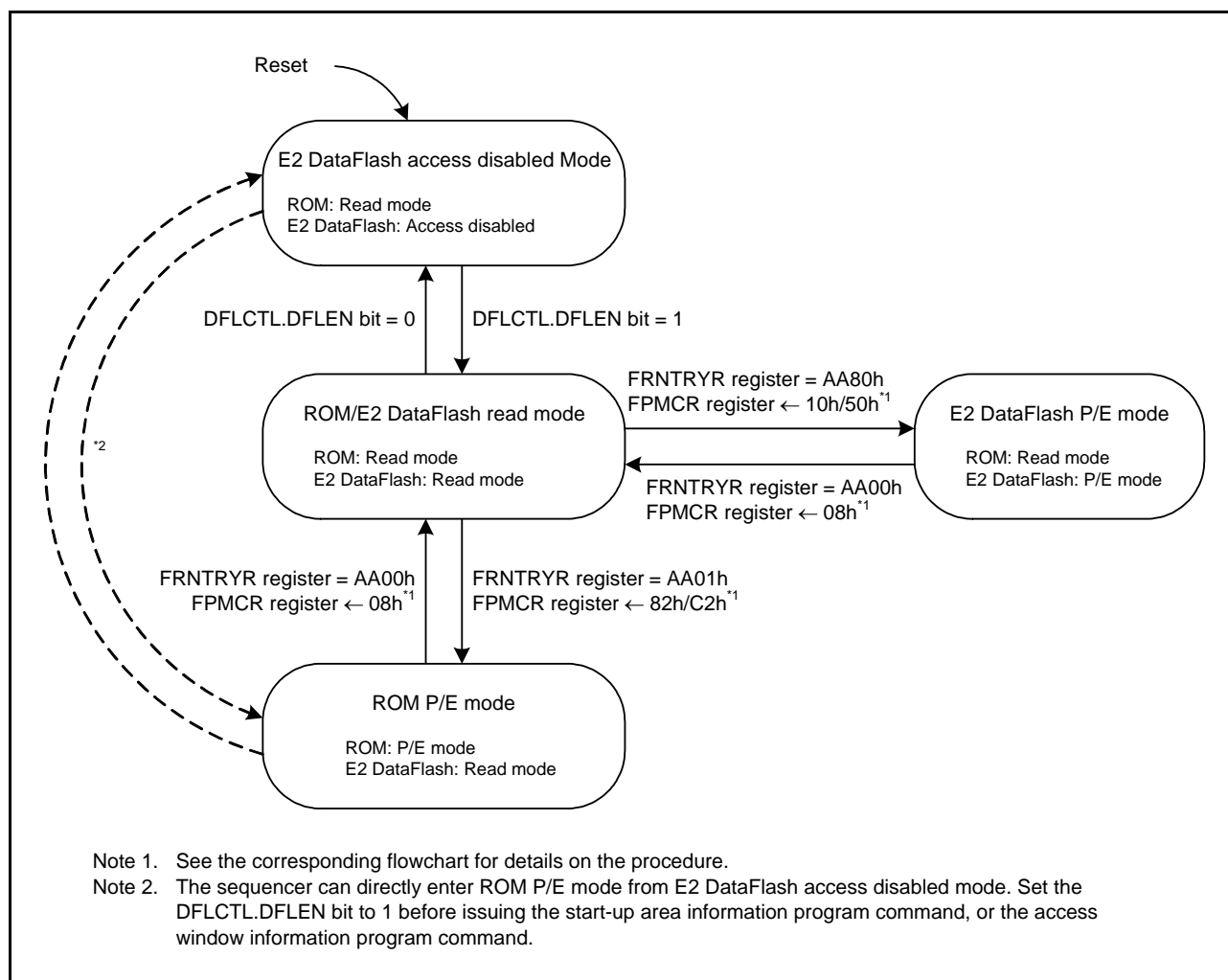
Figure 34.6 Mode Transitions of the Flash Memory
