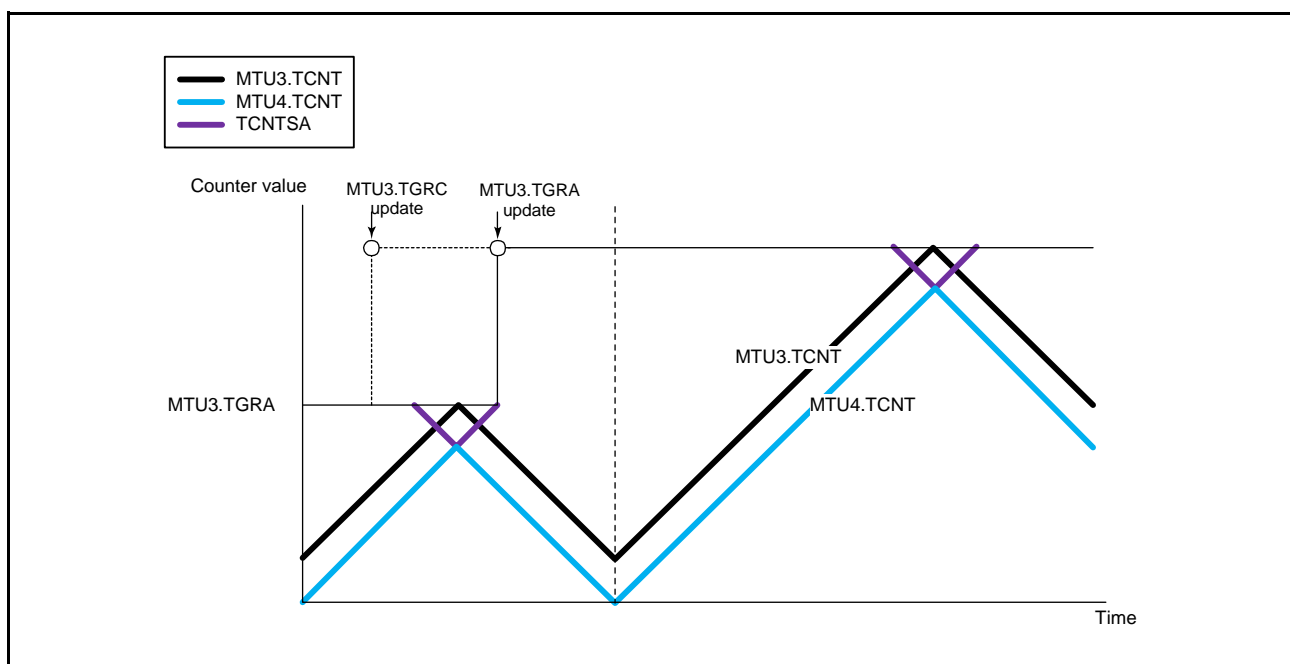
Figure 20.51 Example of PWM Cycle Updating (MTU3 and MTU4)
