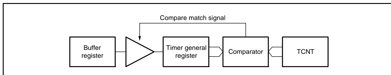
Figure 20.15 Compare Match Buffer Operation
