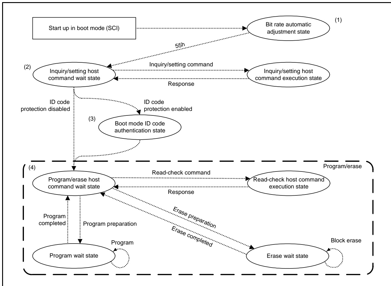
Figure 34.29 Boot Mode (SCI) State Transition
