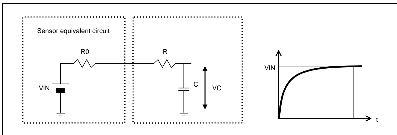
Figure 29.35 Equivalent Circuit of Analog Input Pin and External Sensor
