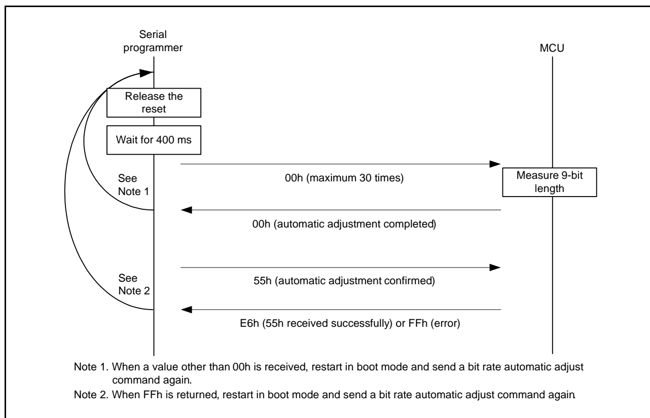
Figure 34.31 Bit Rate Automatic Adjustment Procedure
