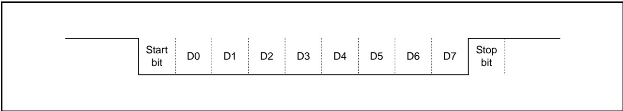
Figure 34.23 Communication Format
