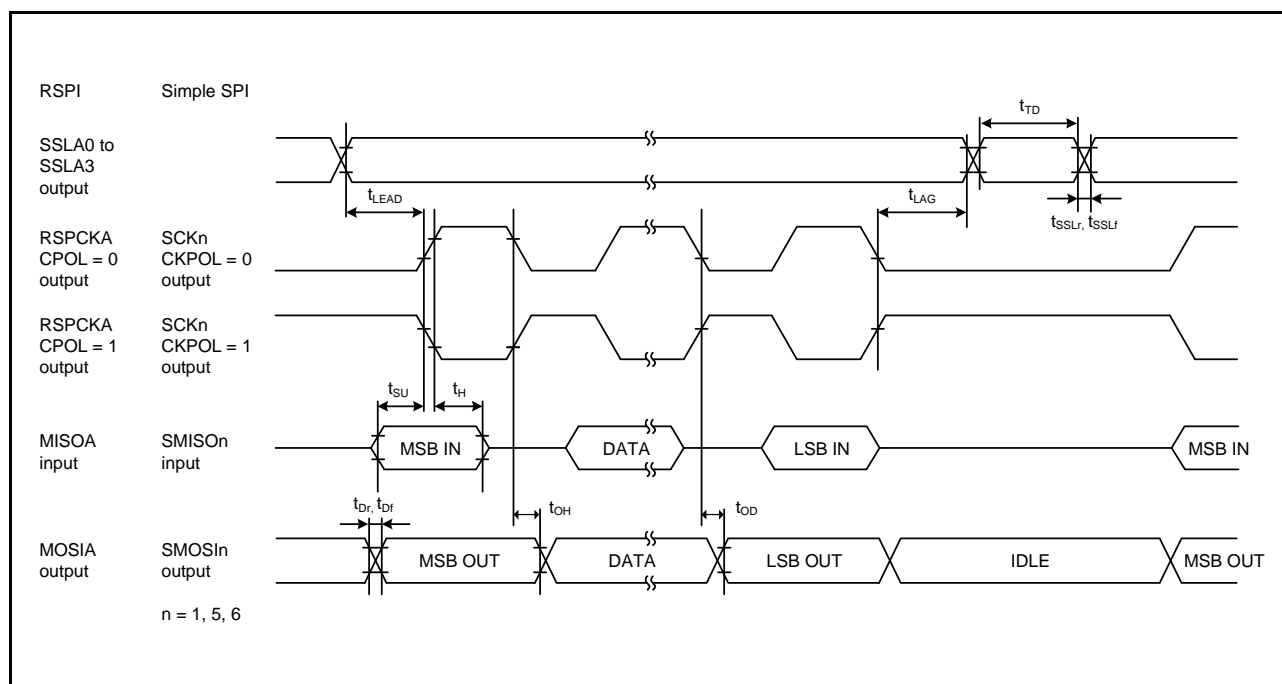
Figure 35.41 RSPI Timing (Master, CPHA = 0) and Simple SPI Clock Timing (Master, CKPH = 1)
