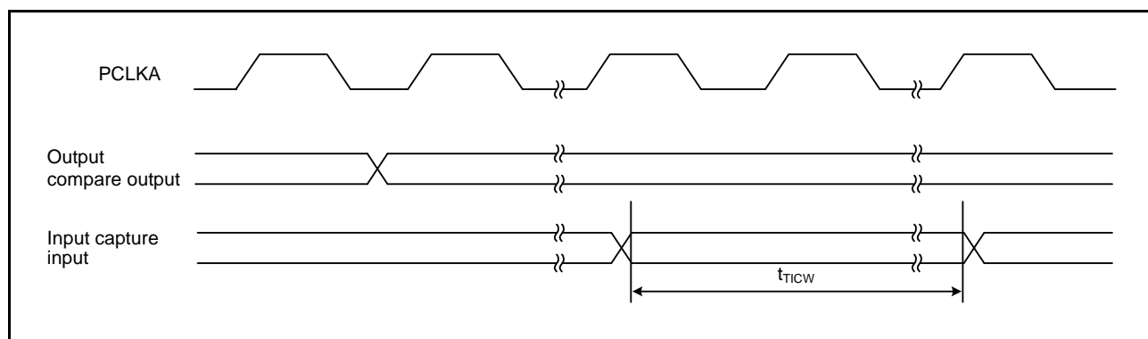
Figure 35.33 MTU3 Input/Output Timing
