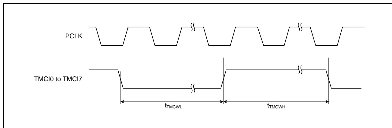
Figure 35.36 TMR Clock Input Timing
