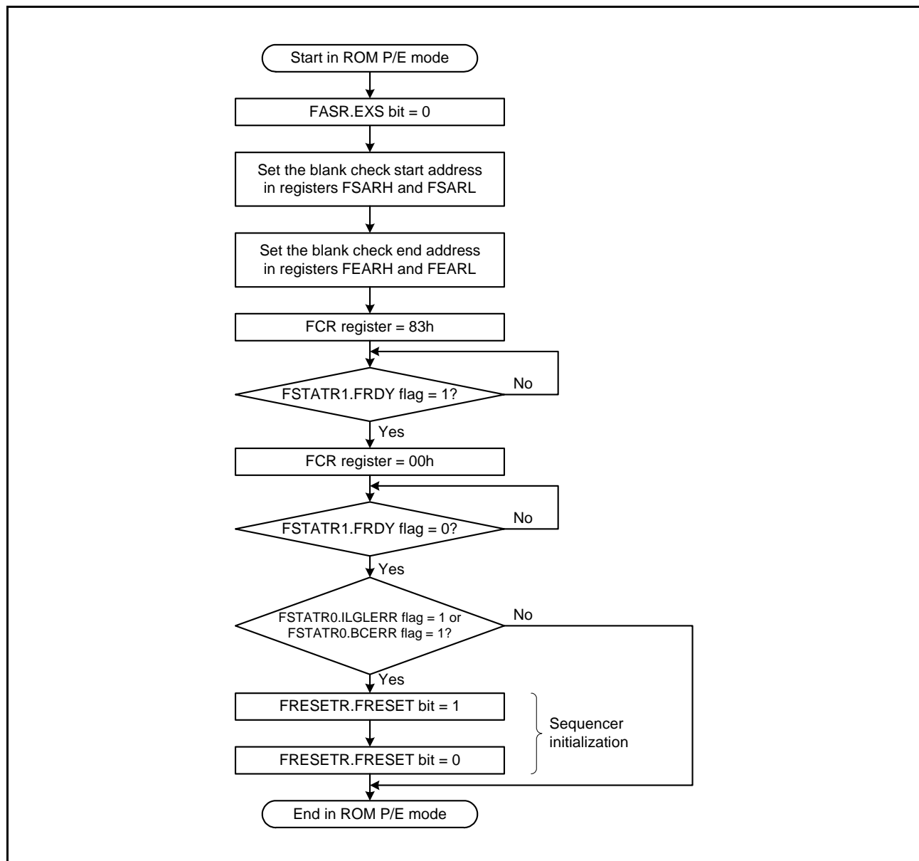
Figure 34.18 Procedure to Issue the Blank Check Command for the ROM
