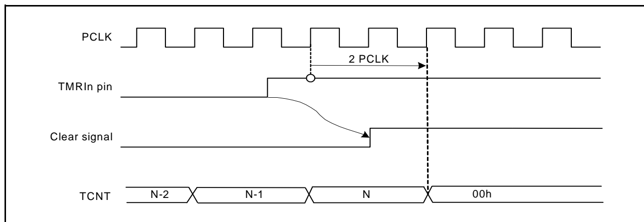
Figure 22.13 Clear Timing by External Counter Reset Signal (High Level)
