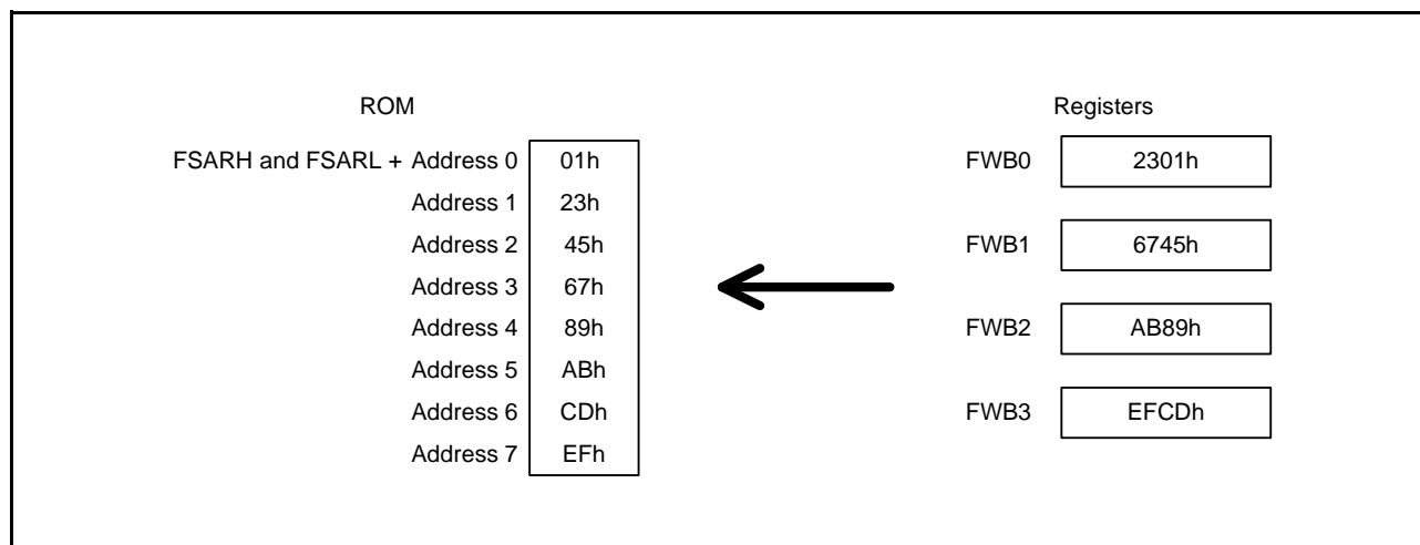
Figure 34.3 FWBn Register Setting Values and Data Allocation in the ROM
