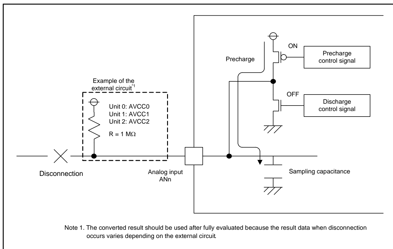
Figure 29.32 Example of Disconnection Detection When Precharge is Selected
