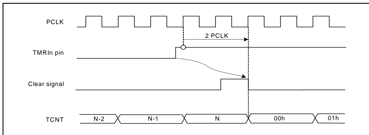
Figure 22.12 Clear Timing by External Counter Reset Signal (Rising Edge)
