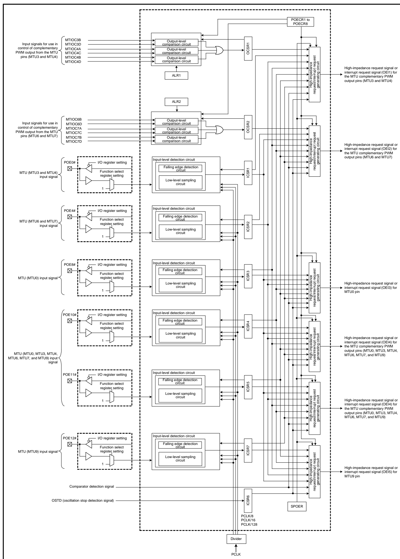
Figure 21.1 POE Block Diagram
