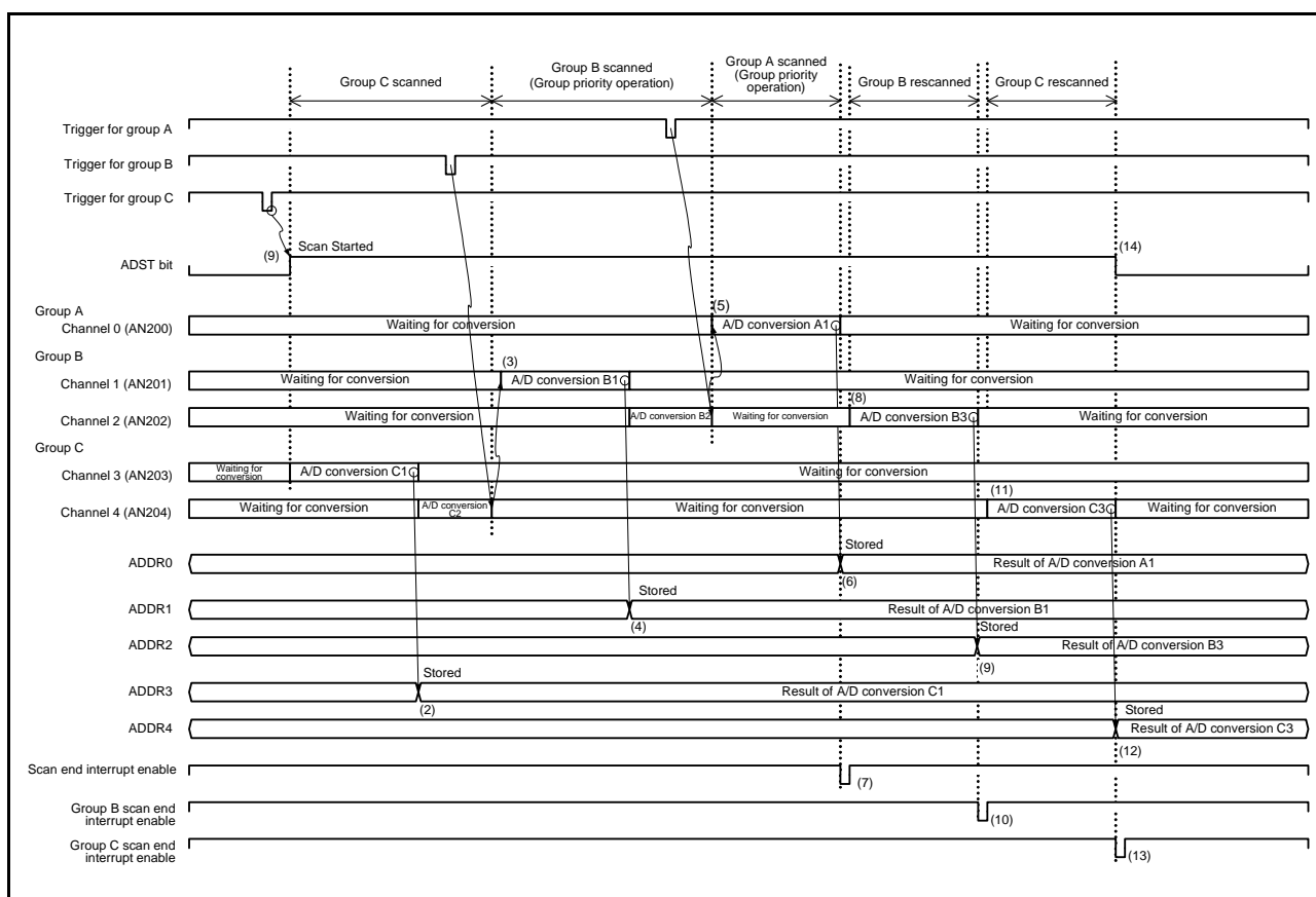
Figure 29.24 Example 1 of Group Priority Operation: Priority Group Trigger Input during Low-Priority Group Scan, With Rescan Setting (ADGSPCR.GBRSCN = 1, ADGSPCR.GBRP = 0, ADGSPCR.LGRRS = 1)
