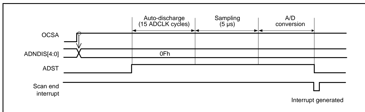
Figure 29.9 Example of Operation in Single Scan Mode (Internal Reference Voltage Selected: S12AD2 only)
