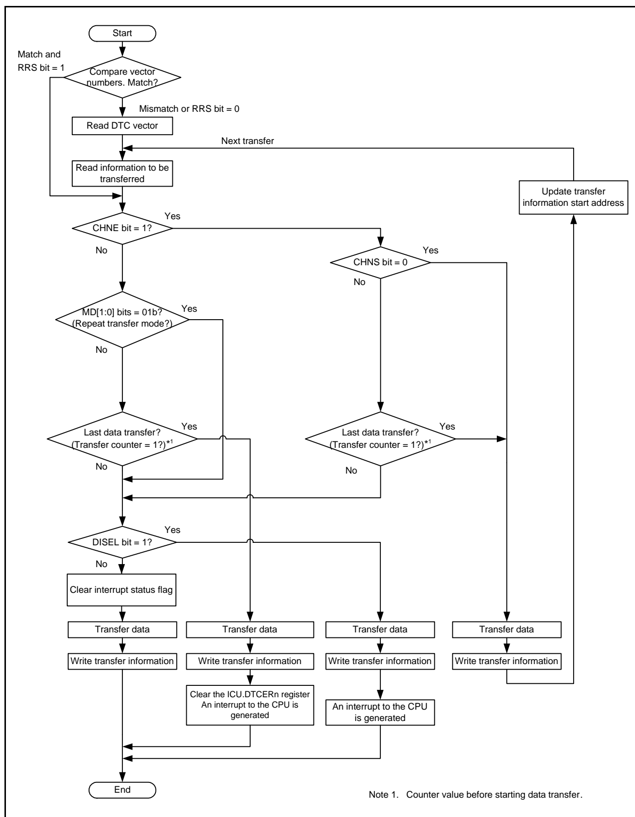
Figure 17.4 Operation Flowchart of the DTC
