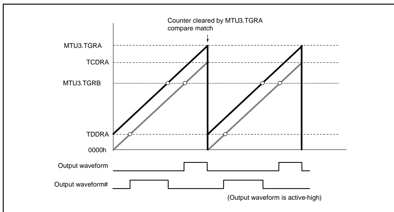
Figure 20.77 Example of Counter Clearing Operation by MTU3.TGRA Compare Match
