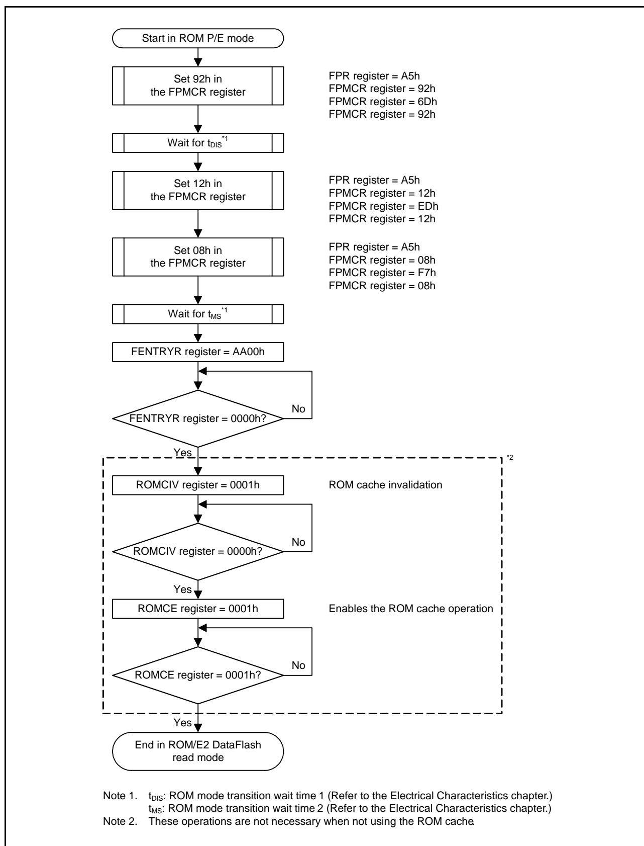
Figure 34.10 Procedure for Transition from ROM P/E Mode to ROM/E2 DataFlash Read Mode
