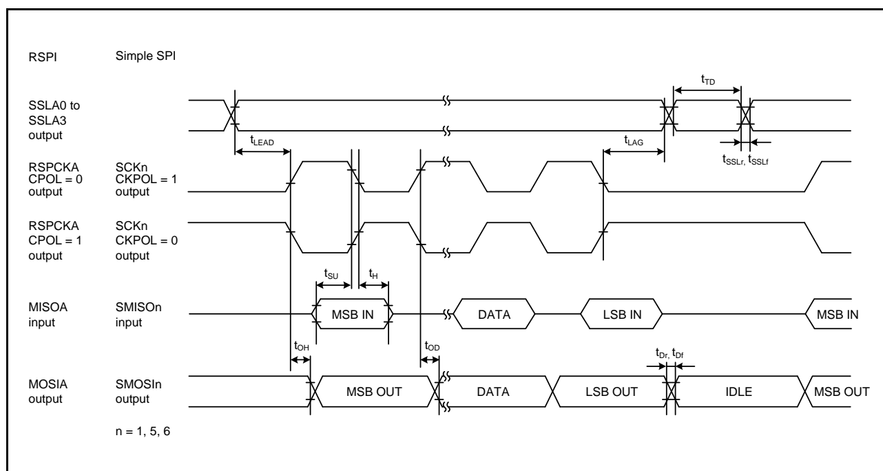
Figure 35.42 RSPI Timing (Master, CPHA = 1) and Simple SPI Clock Timing (Master, CKPH = 0)
