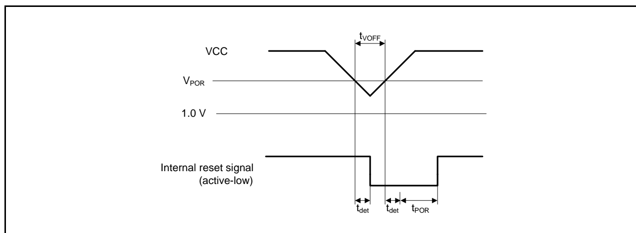
Figure 35.48 Voltage Detection Reset Timing
