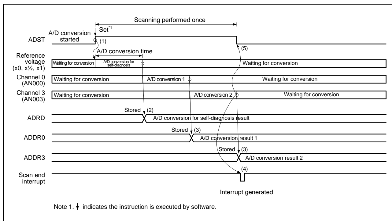
Figure 29.7 Example of Operation in Single Scan Mode (Basic Operation: AN000, AN003 Selected + Self-Diagnosis)
