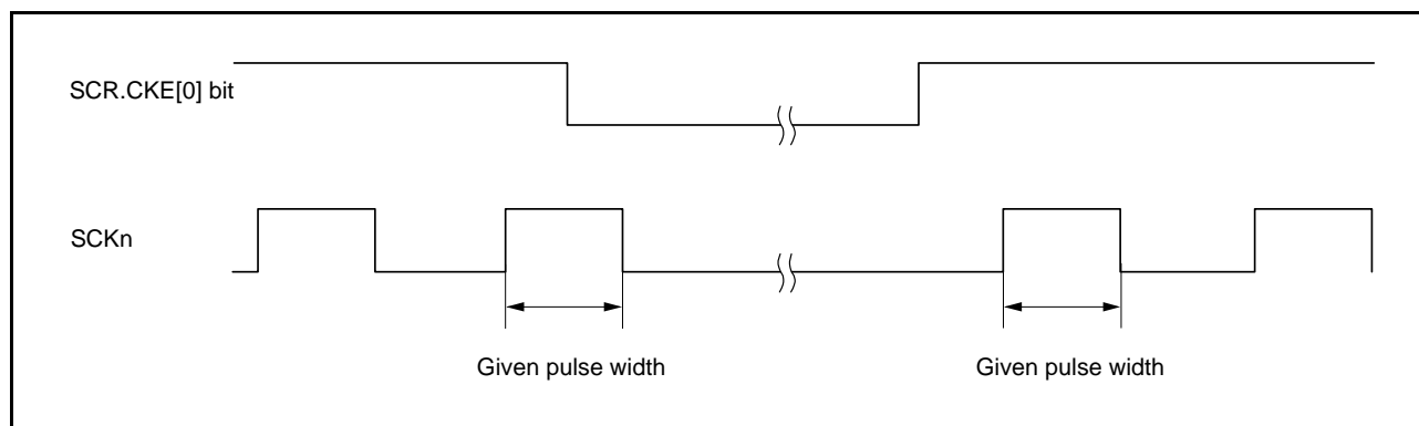
Figure 25.42 Clock Output Fixing Timing
