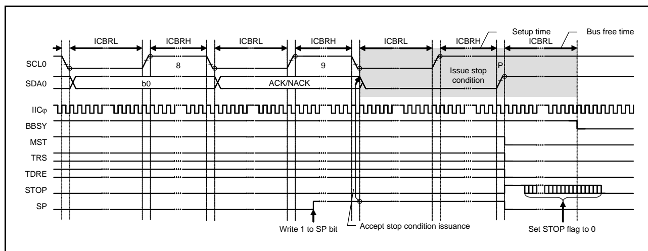
Figure 26.38 Stop Condition Issue Timing (SP Bit)
