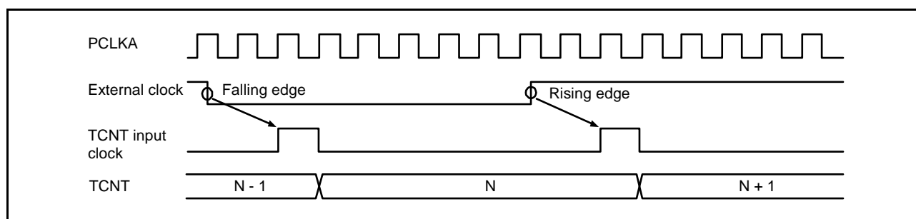
Figure 20.113 Count Timing in External Clock Operation (MTU0 to MTU4, MTU9)
