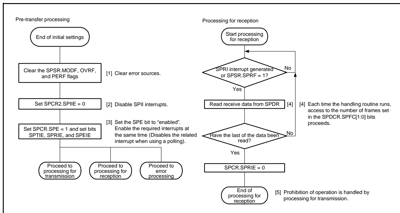
Figure 27.37 Flowchart in Master Mode (Reception)
