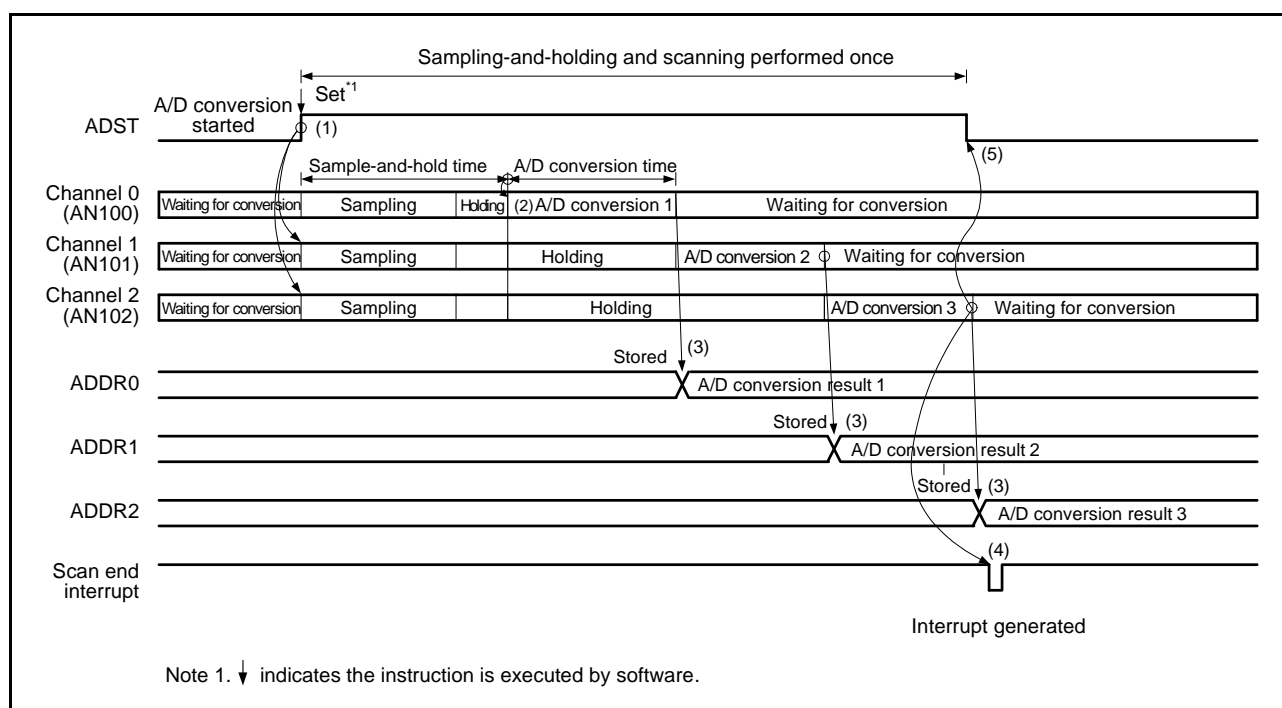
Figure 29.6 Example of Operation in Single Scan Mode (Channel-Dedicated Sample-and-Hold Circuits Used; AN100, AN101, AN102 Selected)
