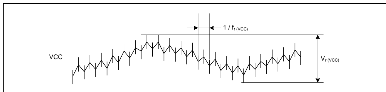
Figure 35.3 Ripple Waveform
