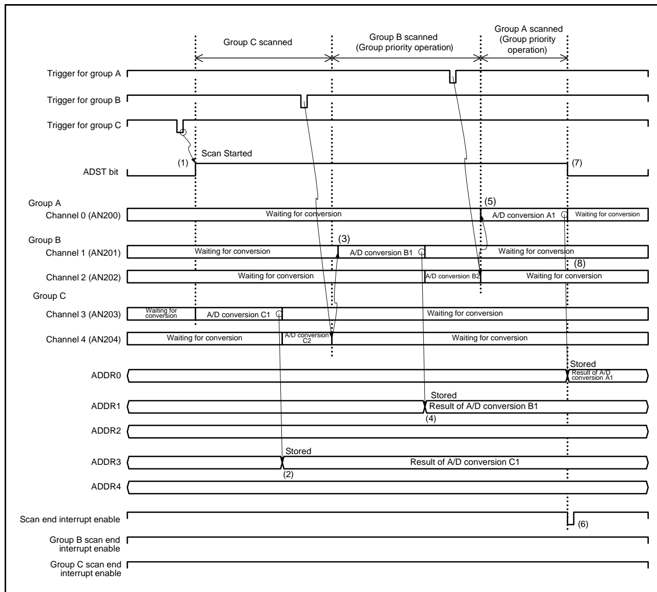
Figure 29.27 Example 4 of Group Priority Operation: Priority Group Trigger Input during Low-Priority Group Scan, Without Rescan Setting (ADGSPCR.GBRSCN = 0, ADGSPCR.GBRP = 0, ADGSPCR.LGRRS = 1)
