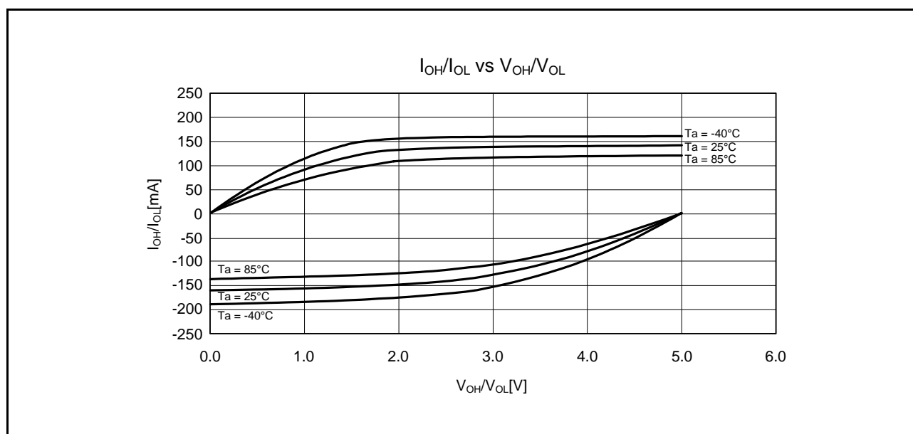
Figure 35.14 V_{OH}/V_{OL} and I_{OH}/I_{OL} Temperature Characteristics of Large Current Ports at V_{CC} = 5.0 V (Reference Data)
