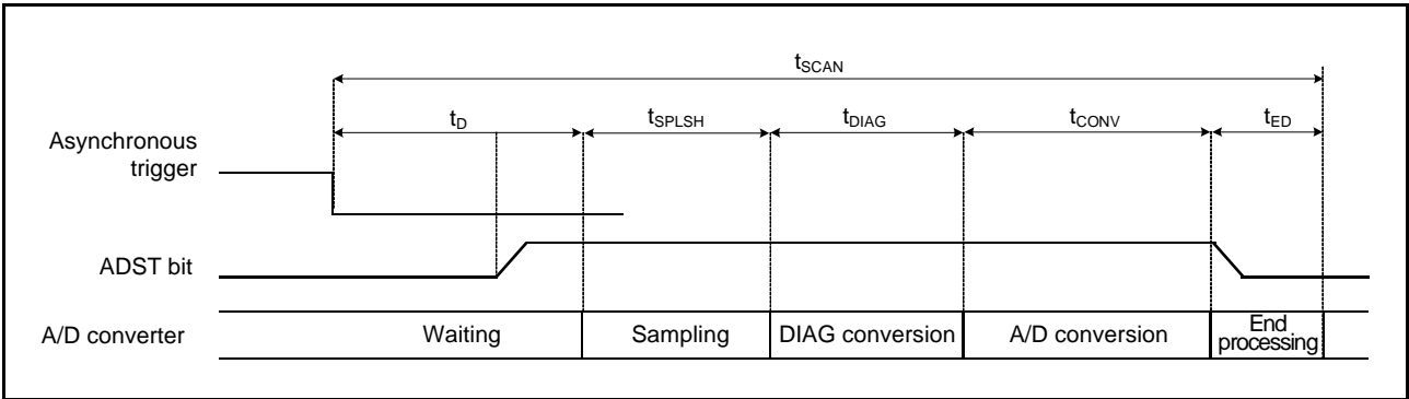
Figure 29.30 Scan Conversion Timing (Activated by Asynchronous Trigger)
