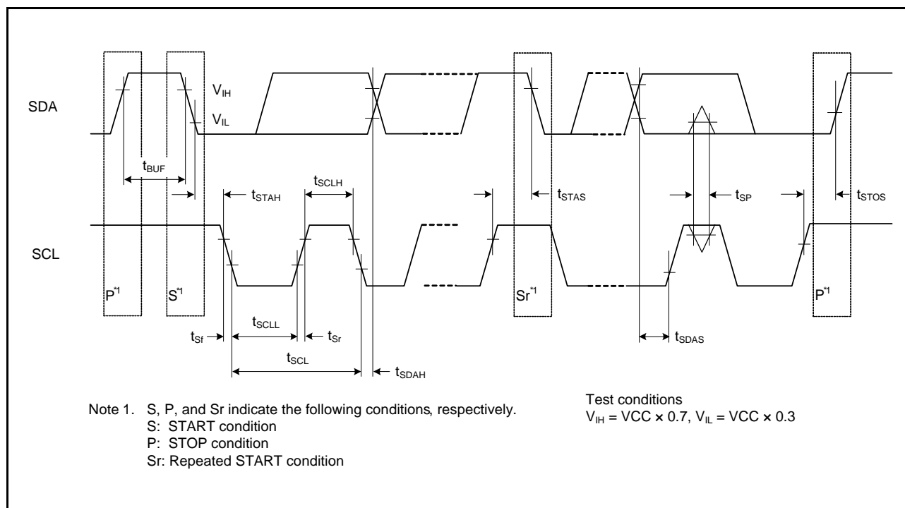
Figure 35.45 RIIC Bus Interface Input/Output Timing and Simple I 2 C Bus Interface Input/Output Timing
