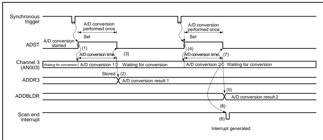
Figure 29.10 Example of Operation in Single Scan Mode (Double Trigger Mode Selected; AN003 Duplicated)
