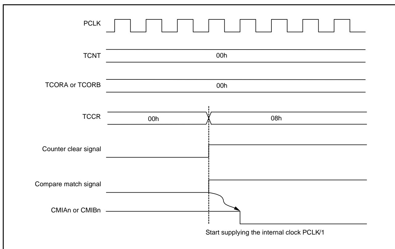
Figure 22.18 Continuous Output of Compare Match Interrupt Signal (n = 0 to 7)
