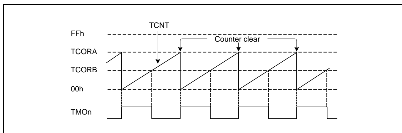
Figure 22.5 Example of Pulse Output (n = 0 to 7)
