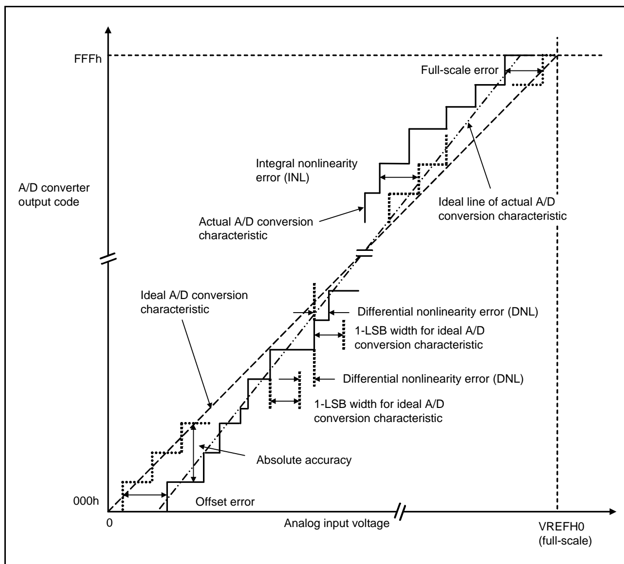
Figure 35.46 Illustration of A/D Converter Characteristic Terms
