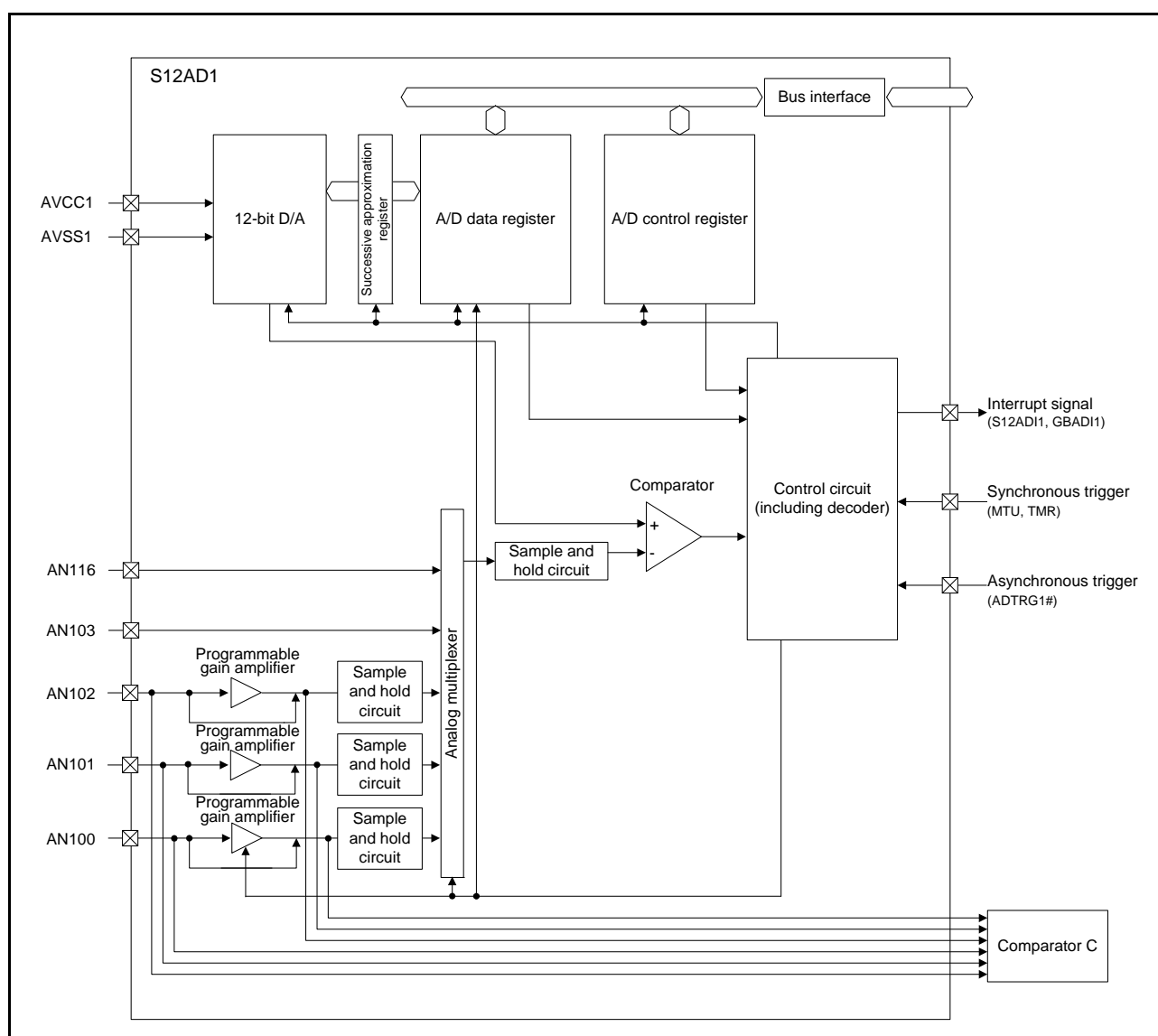
Figure 29.2 Block Diagram of 12-Bit A/D Converter (Unit 1)
