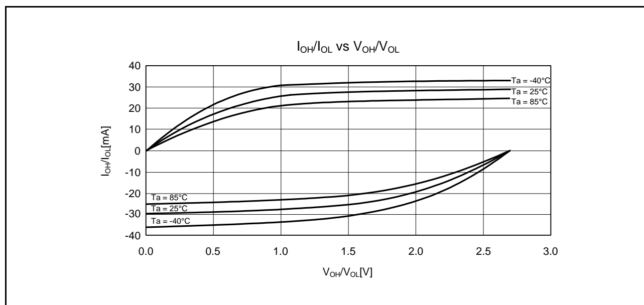
Figure 35.9 V_{OH}/V_{OL} and I_{OH}/I_{OL} Temperature Characteristics at V_{CC} = 2.7 V when Normal Output is Selected (Reference Data)
