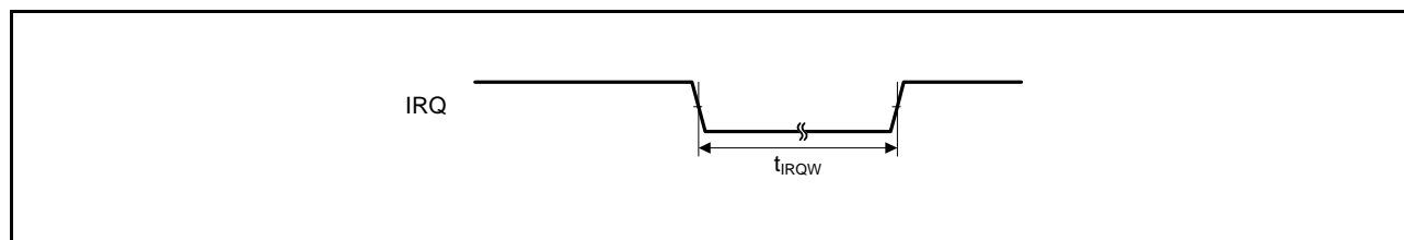
Figure 35.31 IRQ Interrupt Input Timing
