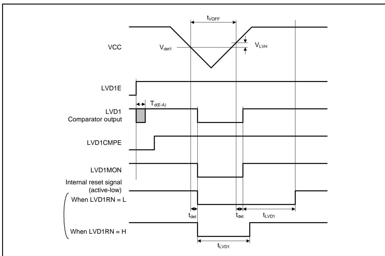
Figure 35.51 Voltage Detection Circuit Timing ( V_{det1} )
