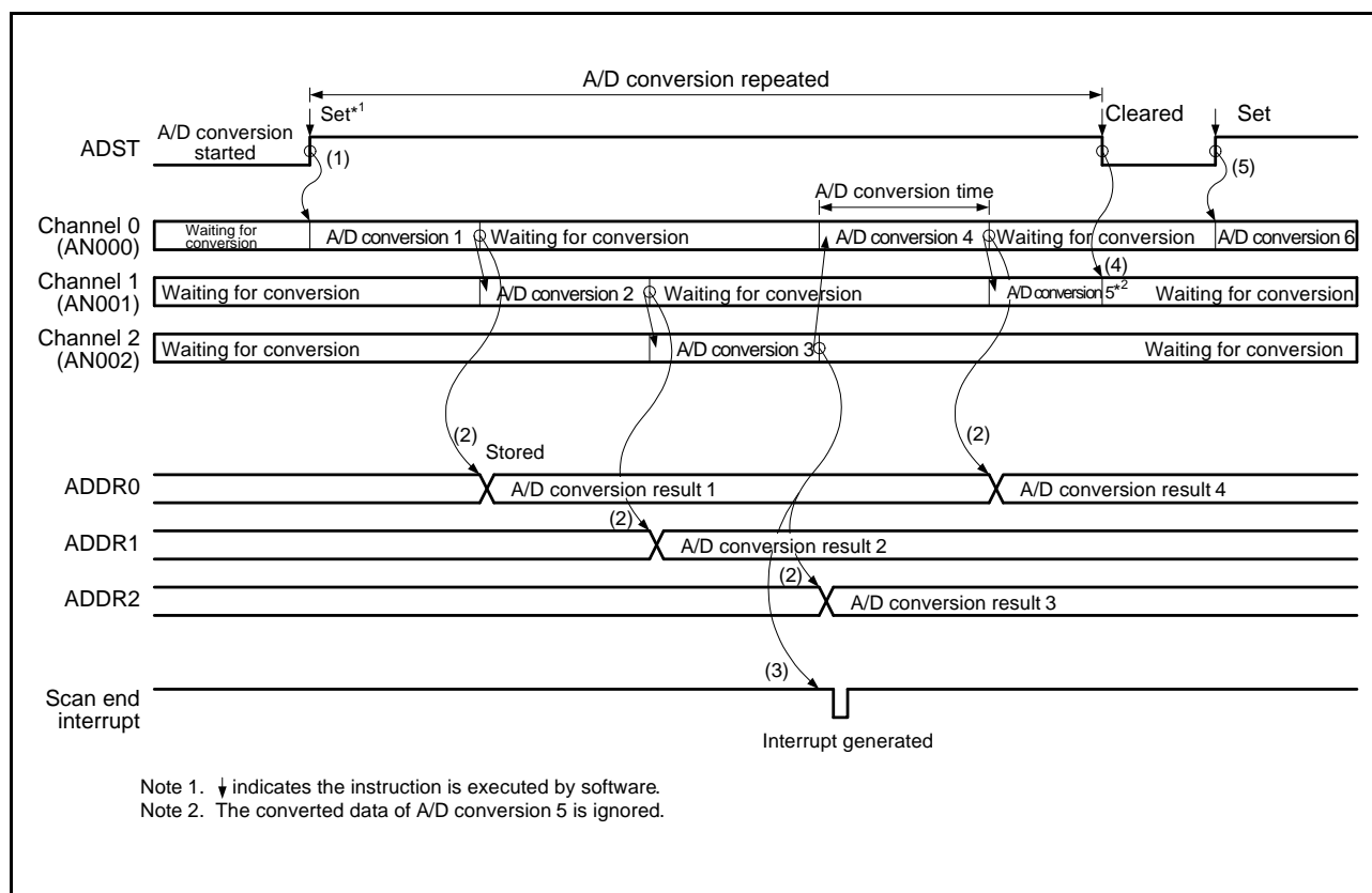
Figure 29.12 Example of Operation in Continuous Scan Mode (Basic Operation: AN000 to AN002 Selected)
