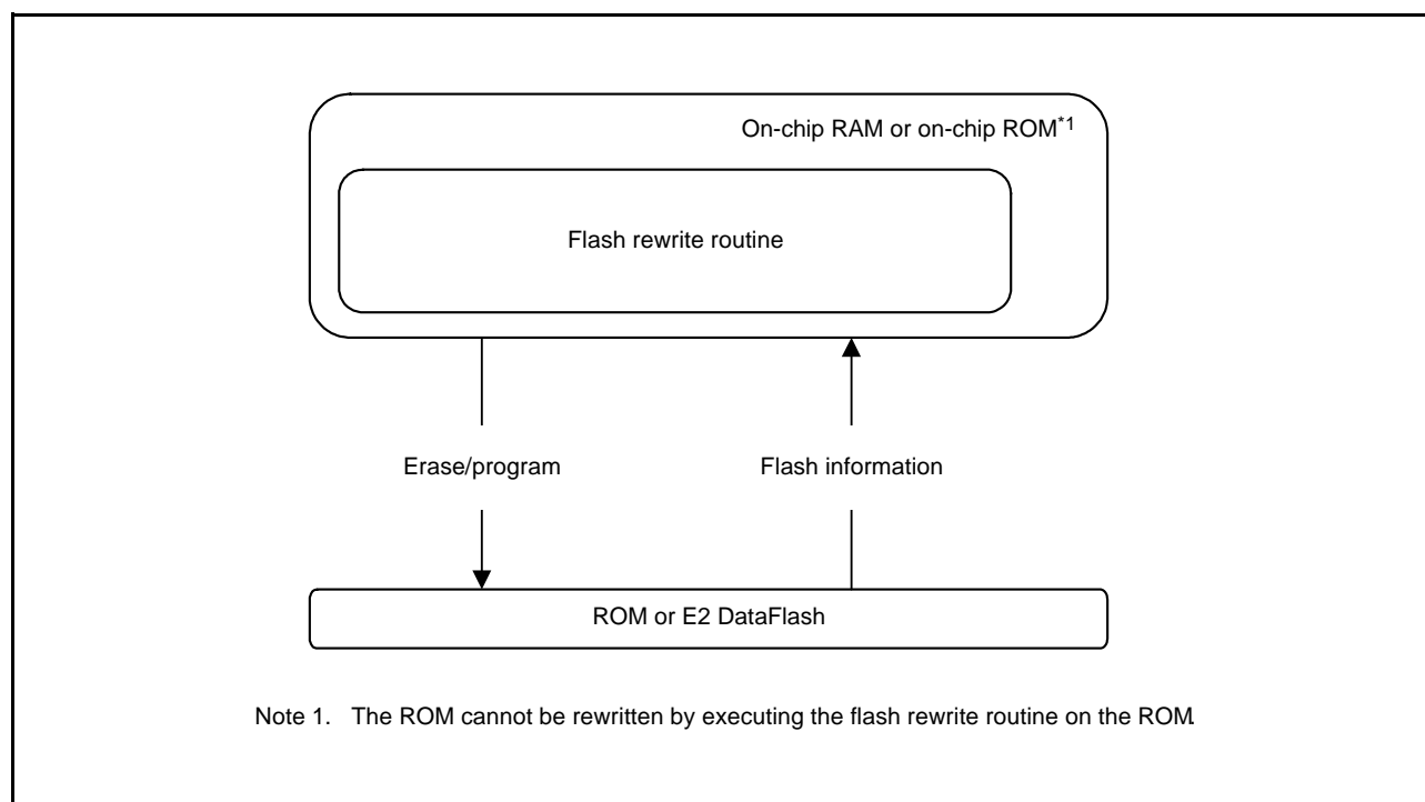
Figure 34.41 Self-Programming Overview
