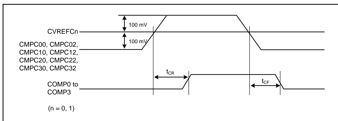
Figure 35.47 Comparator Response Time
