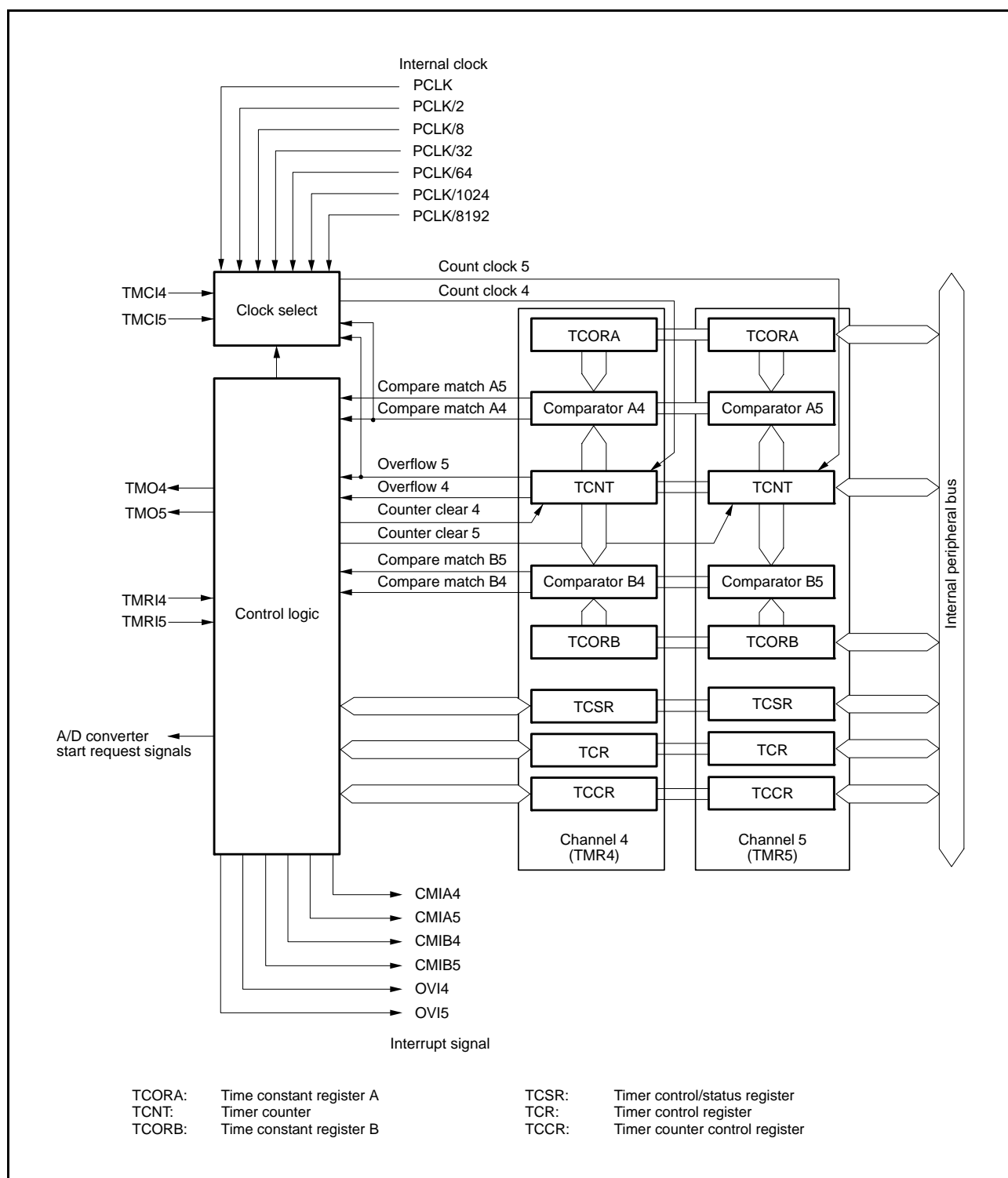
Figure 22.3 Block Diagram of TMR (Unit 2)
