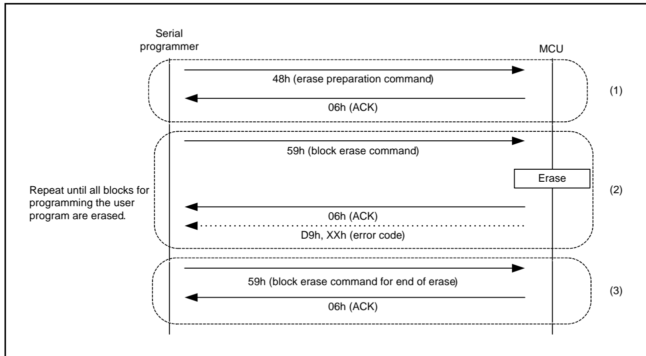
Figure 34.36 Procedure to Erase the User Area and Data Area
