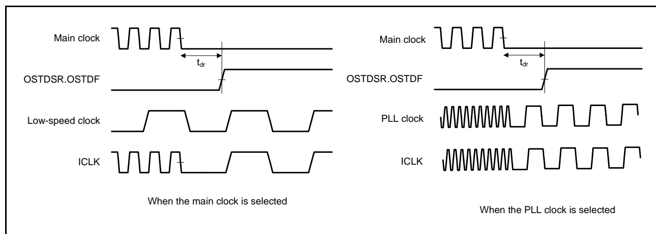
Figure 35.53 Oscillation Stop Detection Timing
