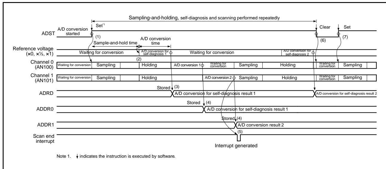
Figure 29.15 Example of Operation in Continuous Scan Mode (Channel-Dedicated Sample-and-Hold Circuits Used: AN100 and AN101 Selected + Self-Diagnosis)
