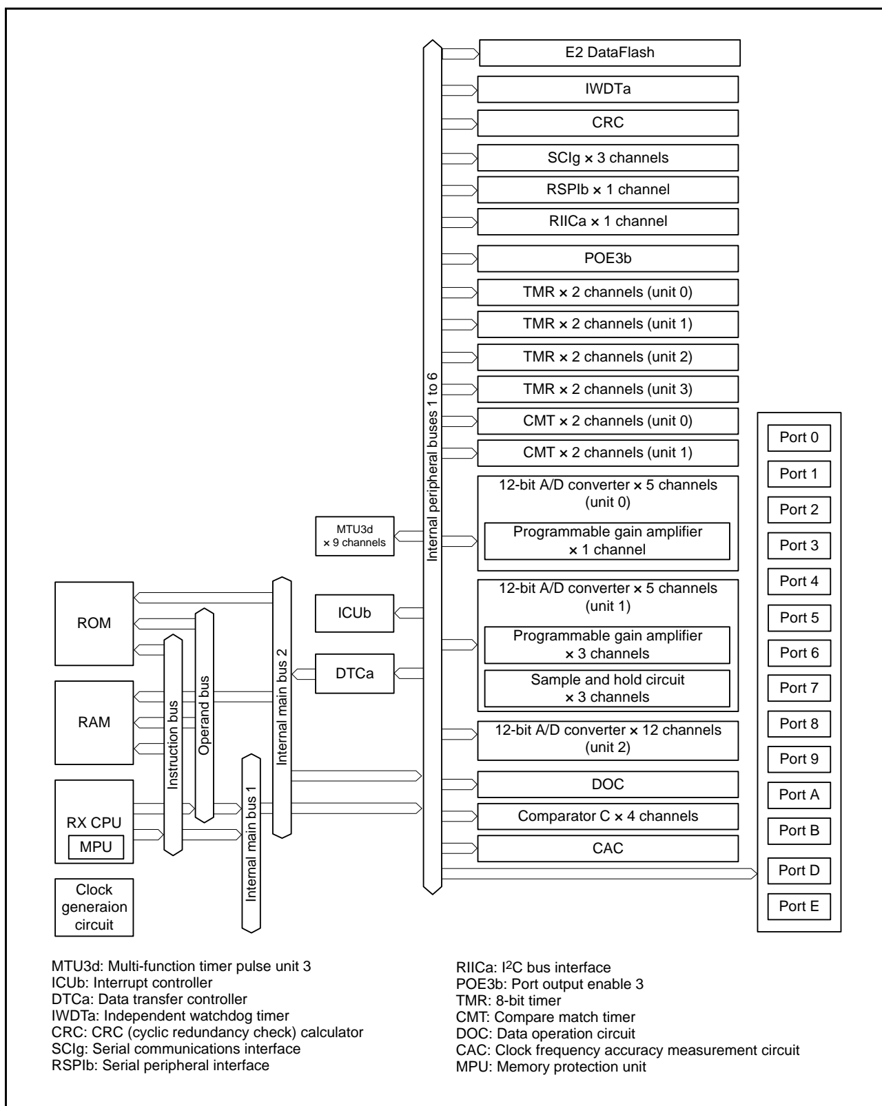
Figure 1.2 Block Diagram
