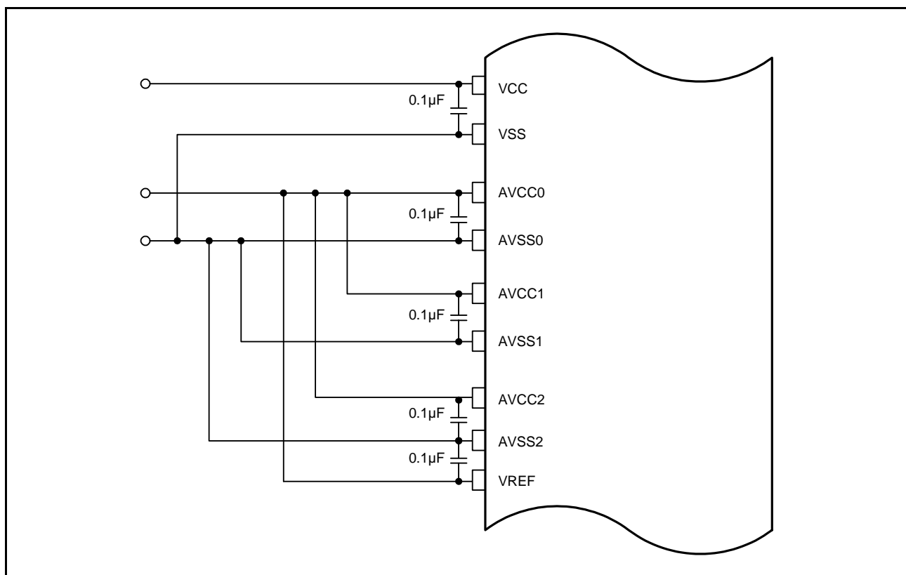
Figure 29.37 Power Supply Pin Connection Example
