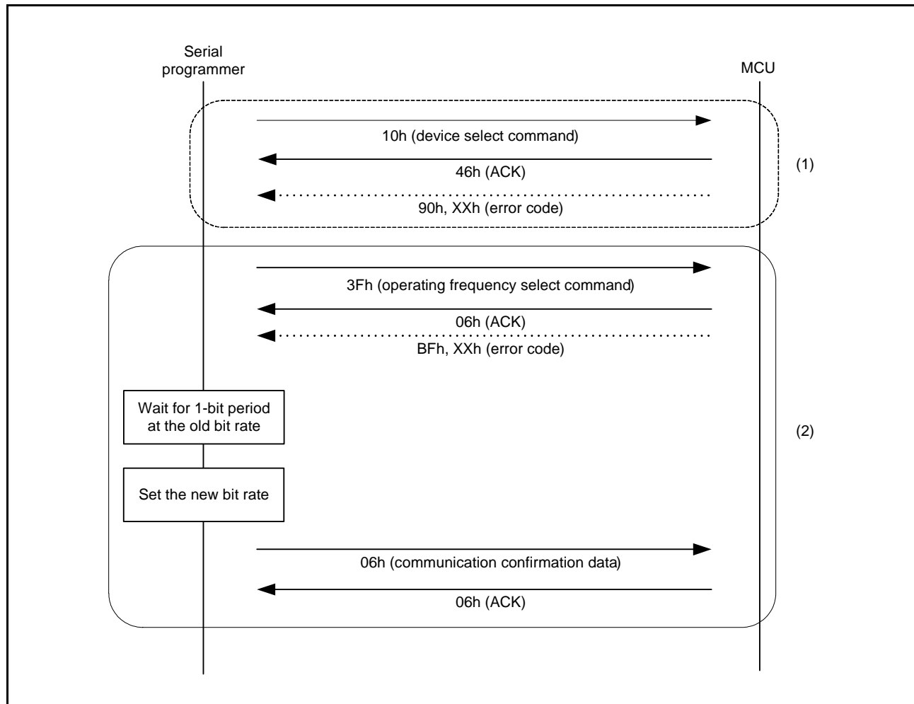
Figure 34.33 Procedure to Select the Device and Change the Bit Rate
