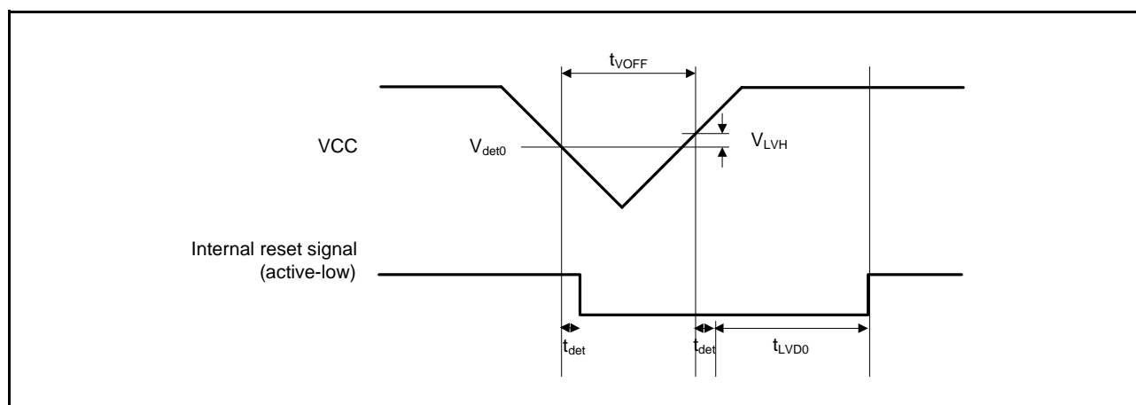
Figure 35.50 Voltage Detection Circuit Timing (Vdet0)
