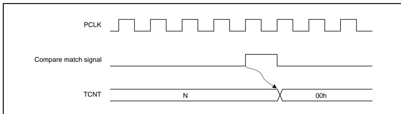
Figure 22.11 Timing of Counter Clear by Compare Match
