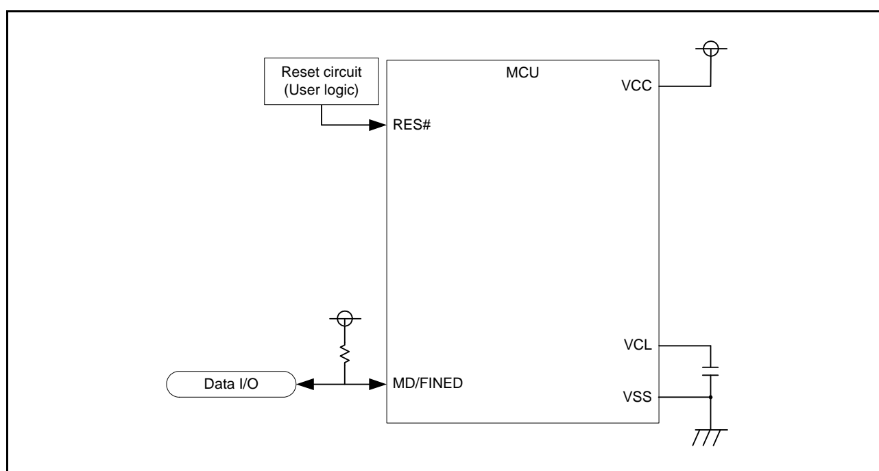
Figure 34.25 Example of Pin Connections in Boot Mode (FINE Interface)
