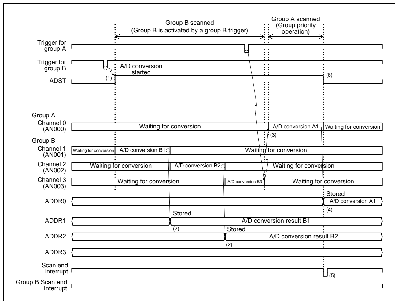
Figure 29.22 Example 4 of Group Priority Operation: Group A Trigger Input during Group B Scan, Without Rescan Setting (ADGSPCR.GBRSCN = 0, ADGSPCR.GBRP = 0, ADGSPCR.LGRRS = 0)
