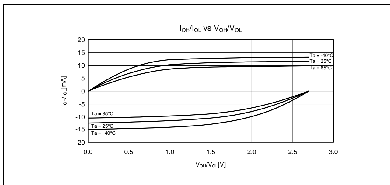
Figure 35.5 V_{OH}/V_{OL} and I_{OH}/I_{OL} Temperature Characteristics at V_{CC} = 2.7 V when Normal Output is Selected (Reference Data)
