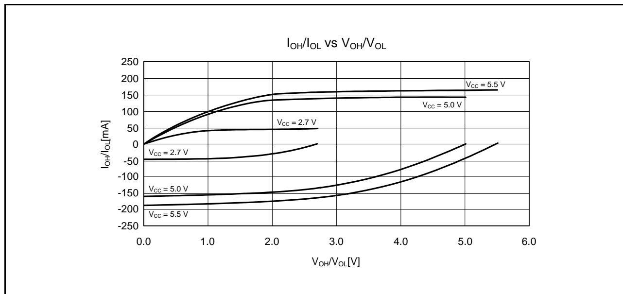
Figure 35.12 V_{OH}/V_{OL} and I_{OH}/I_{OL} Voltage Characteristics of Large Current Ports at T_a = 25^\circ\text{C} (Reference Data)
