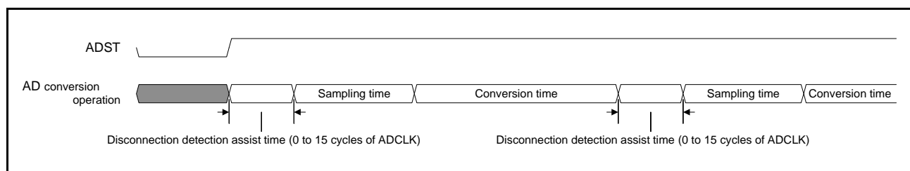
Figure 29.31 Operation of A/D Conversion When the Disconnection Detection Assist Function is Used
