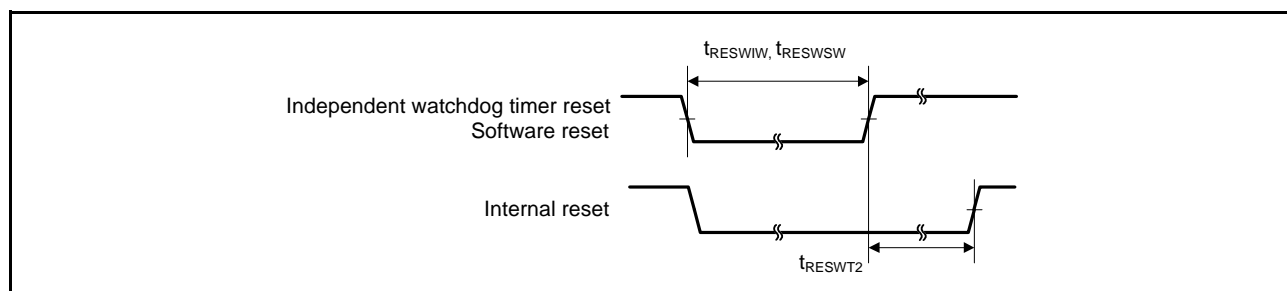
Figure 35.27 Reset Input Timing (2)
