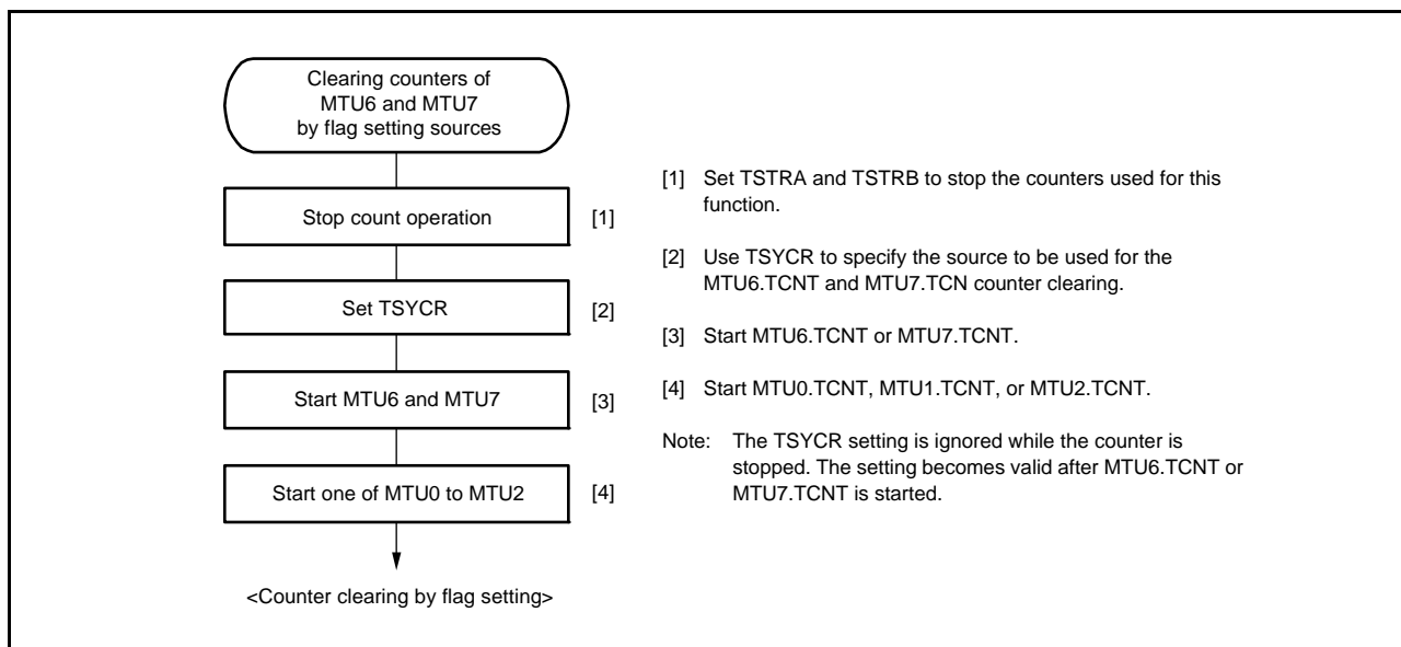
Figure 20.100 Example of Procedure for Specifying Synchronous Counter Clearing for MTU6 and MTU7
