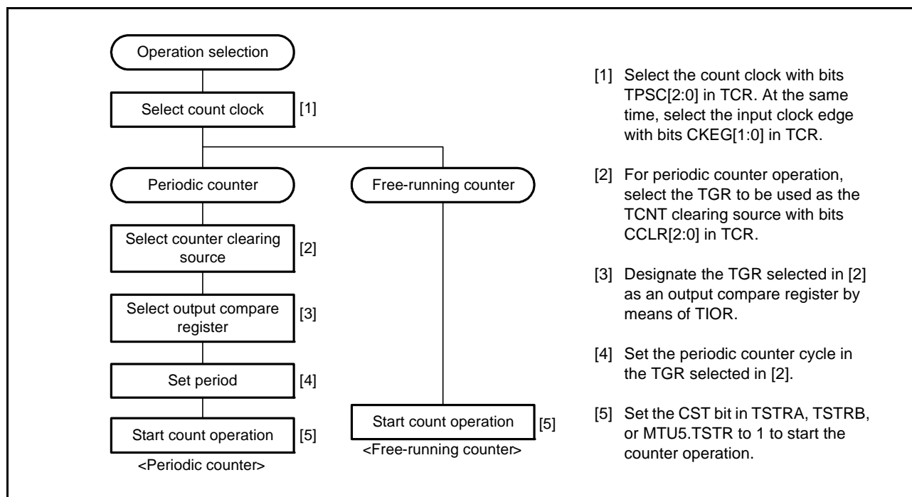
Figure 20.5 Example of Counter Operation Setting Procedure
