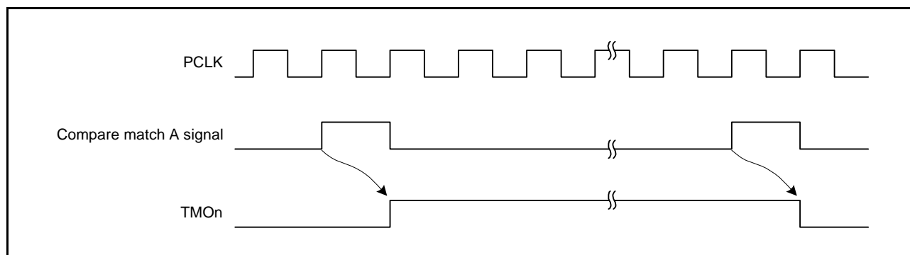
Figure 22.10 Timing of Timer Output Signal at Compare Match A Signal ( n = 0 to 7)
