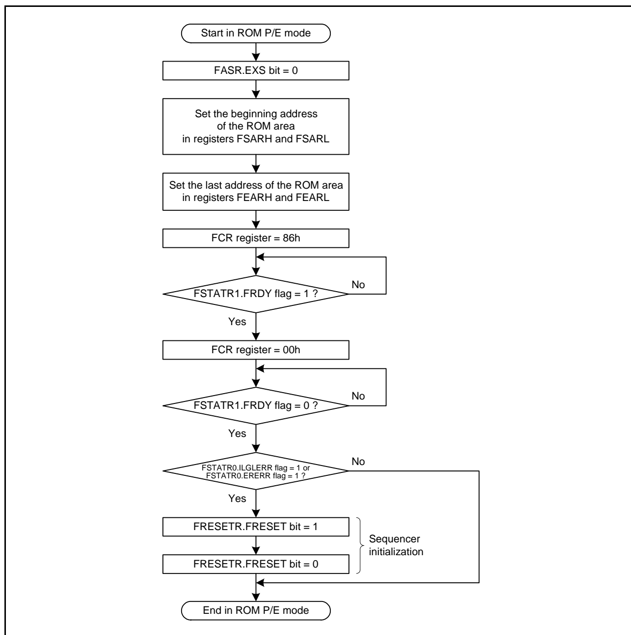
Figure 34.16 Procedure to Issue the All-Block Erase Command for the ROM
