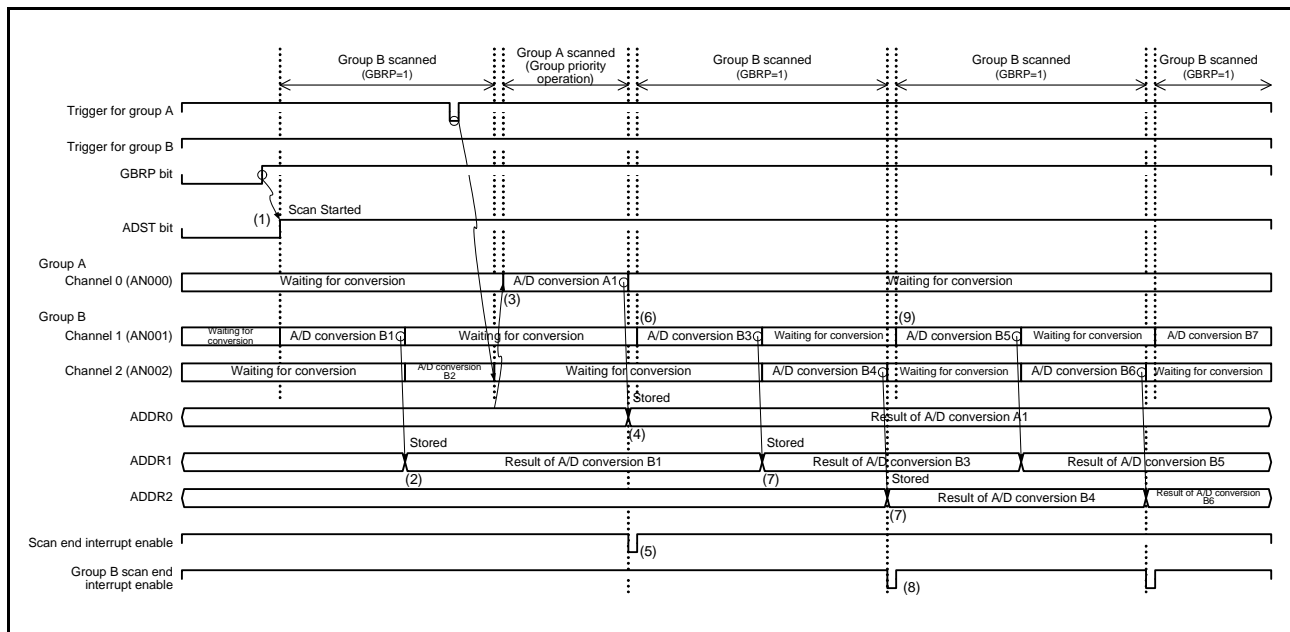
Figure 29.23 Example 5 for Group Priority Operation: Continuous Single Scan Operation on Group B (ADGSPCR.GBRP = 1, ADGSPCR.LGRRS = 1, ADGCTRGR.GRCE = 0)
