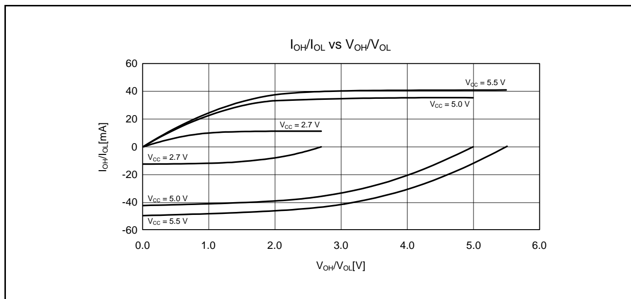
Figure 35.4 V_{OH}/V_{OL} and I_{OH}/I_{OL} Voltage Characteristics at T_a = 25^\circ\text{C} When Normal Output is Selected (Reference Data)
