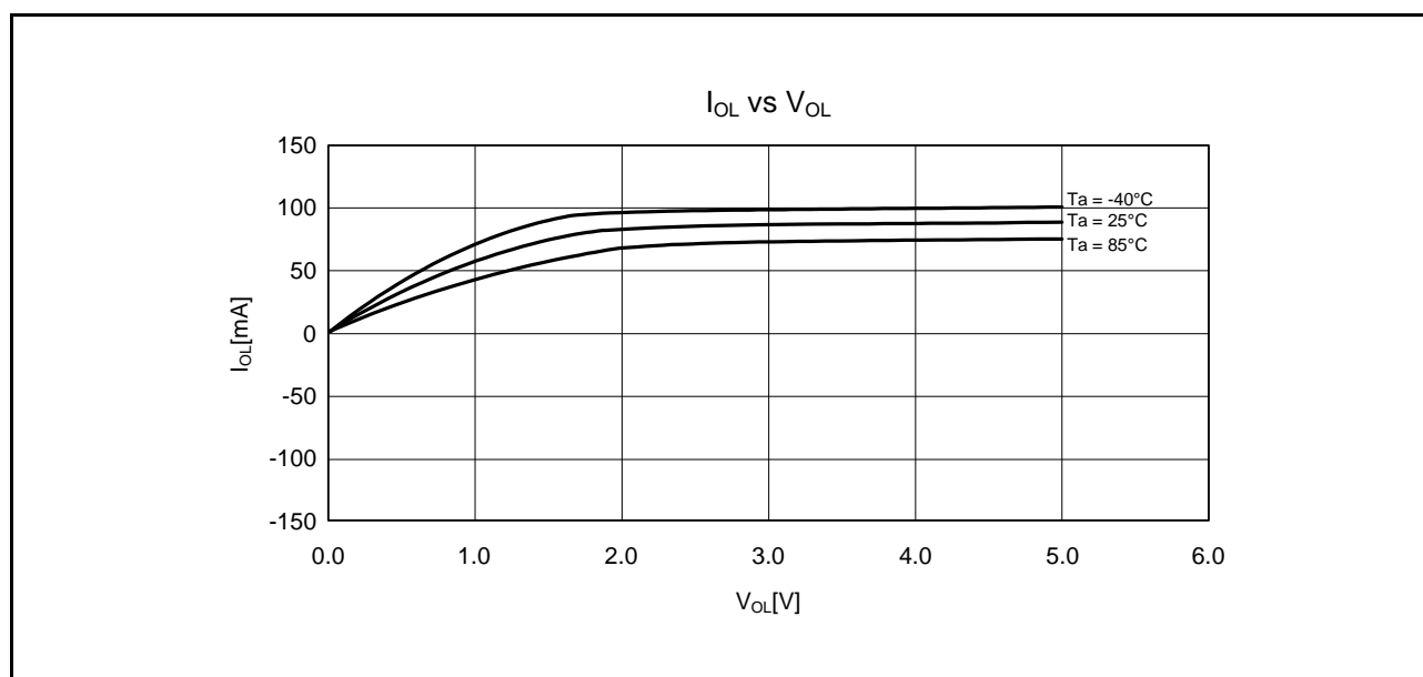
Figure 35.18 V_{OL} and I_{OL} Temperature Characteristics of RIIC Output Pin at V_{CC} = 5.0 V (Reference Data)
