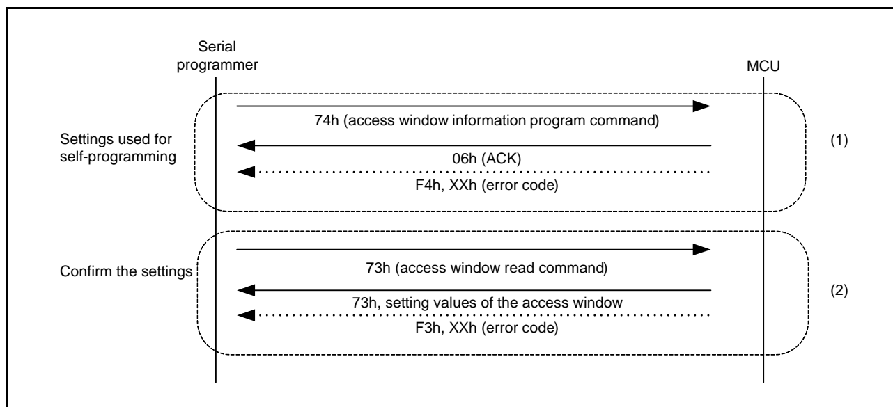
Figure 34.40 Procedure to Set the Access Window in the User Area
