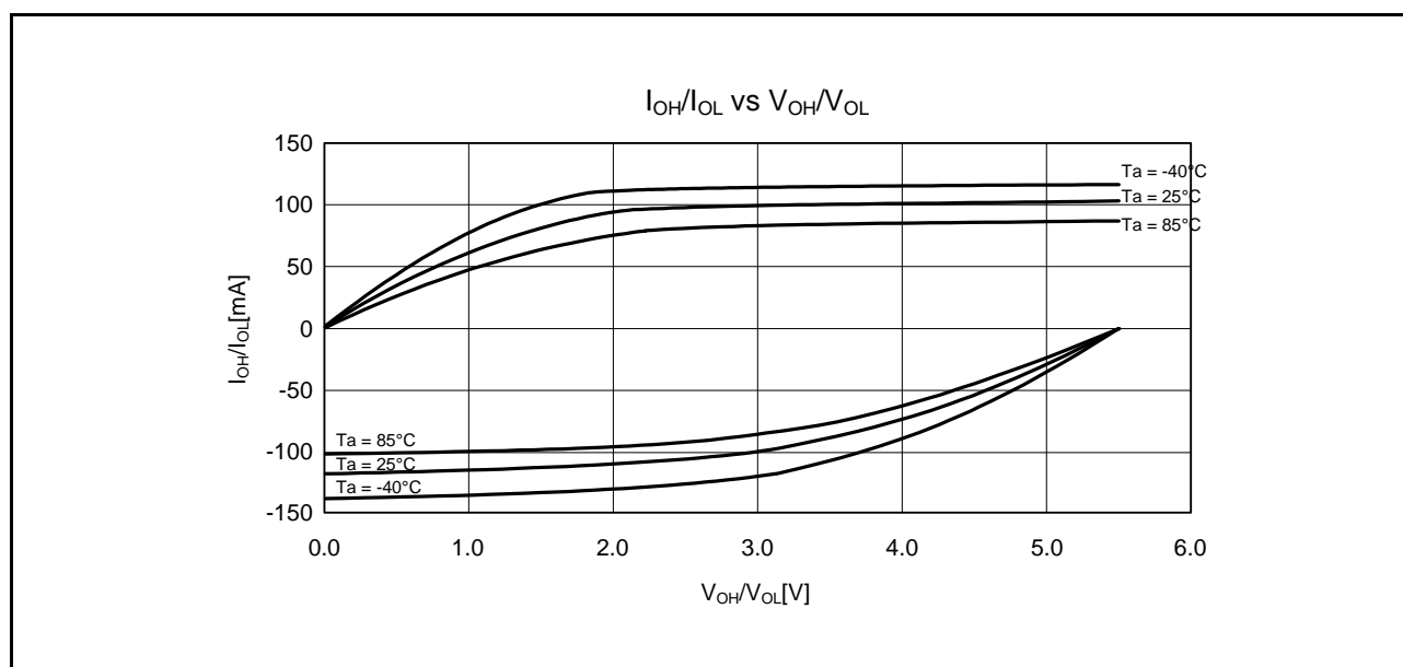
Figure 35.11 V_{OH}/V_{OL} and I_{OH}/I_{OL} Temperature Characteristics at V_{CC} = 5.5 V when Normal Output is Selected (Reference Data)
