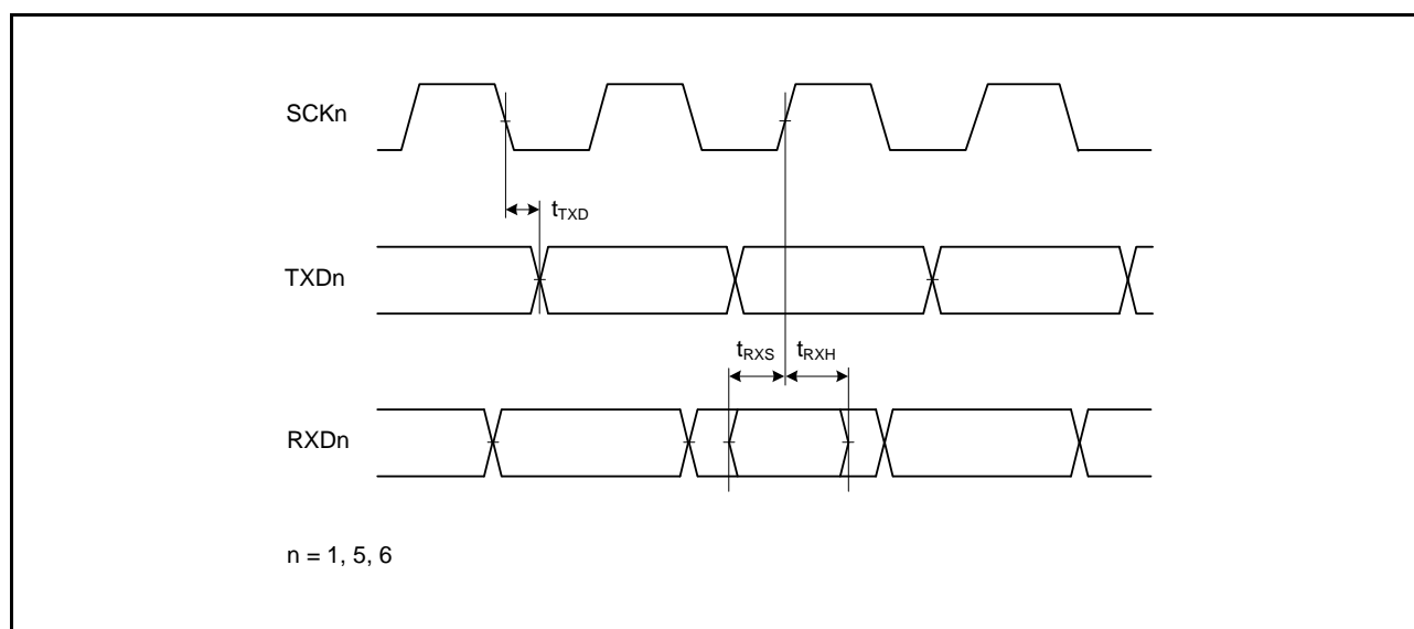
Figure 35.38 SCI Input/Output Timing: Clock Synchronous Mode
