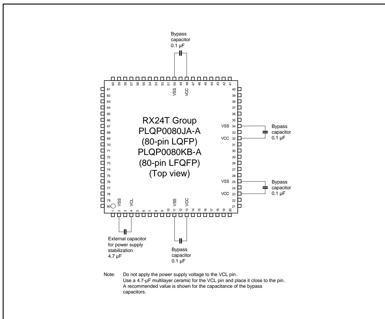
Figure 35.55 Connecting Capacitors (80 Pins)
