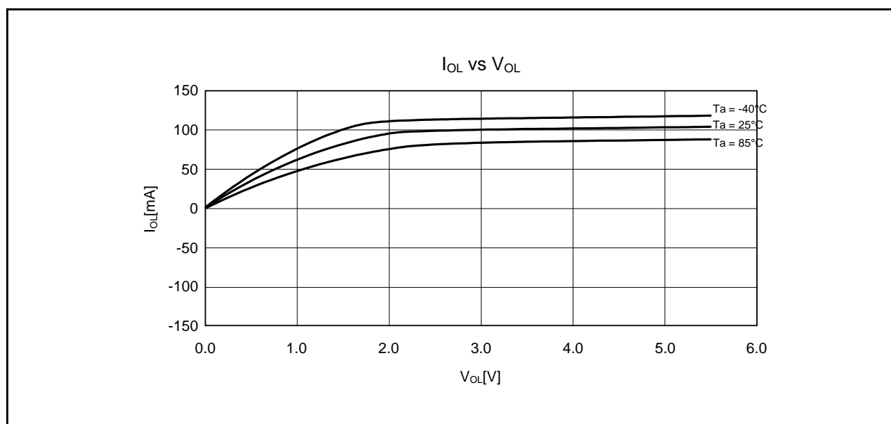
Figure 35.19 V_{OL} and I_{OL} Temperature Characteristics of RIIC Output Pin at V_{CC} = 5.5 V (Reference Data)
