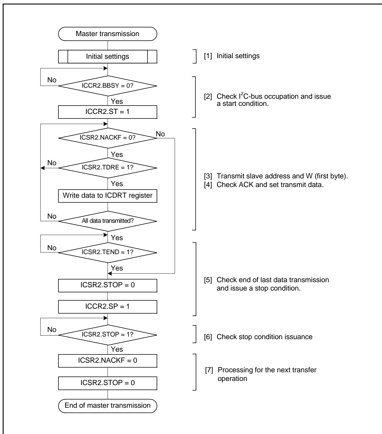
Figure 26.6 Example of Master Transmission Flowchart
