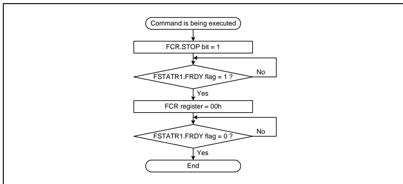
Figure 34.21 Procedure for Forced Stop of Software Commands
