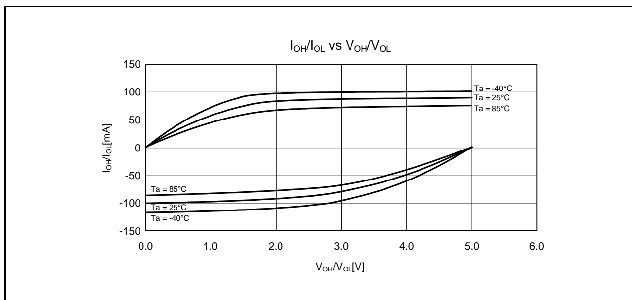
Figure 35.10 V_{OH}/V_{OL} and I_{OH}/I_{OL} Temperature Characteristics at V_{CC} = 5.0 V when Normal Output is Selected (Reference Data)
