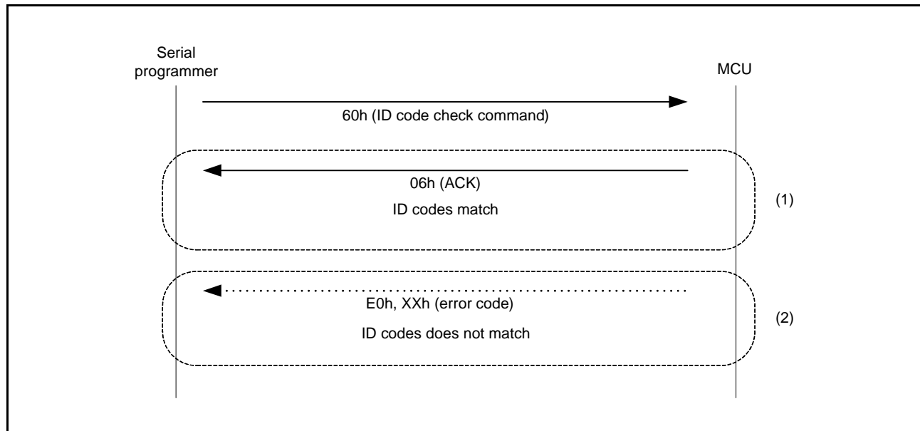
Figure 34.35 Procedure to Unlock ID Code Protection
