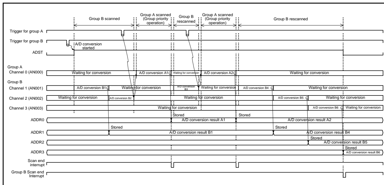
Figure 29.20 Example 2 of Group Priority Operation: Group A Trigger Input during Group B Rescan, With Rescan Setting (ADGSPCR.GBRSCN = 1, ADGSPCR.GBRP = 0, ADGSPCR.LGRRS = 0)
