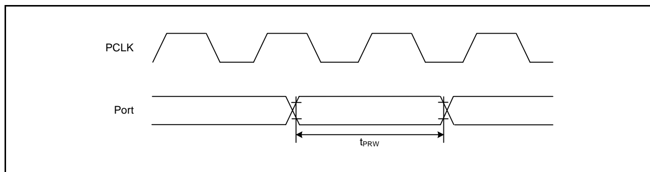
Figure 35.32 I/O Port Input Timing
