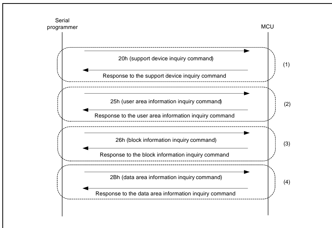
Figure 34.32 Procedure to Receive the MCU Information
