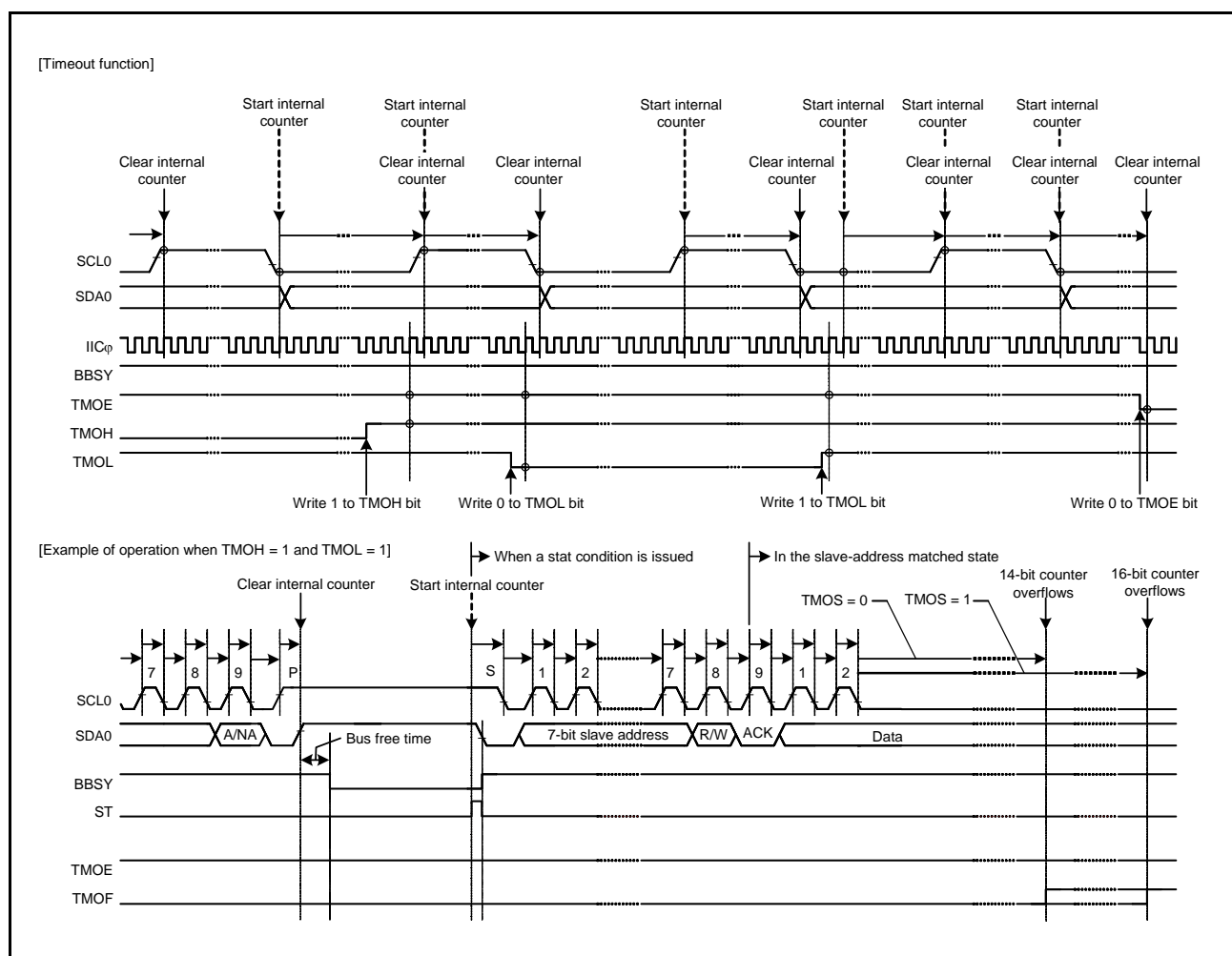
Figure 26.39 Timeout Function
