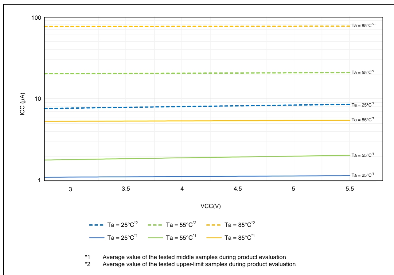
Figure 35.1 Voltage Dependency in Software Standby Mode (Reference Data)
