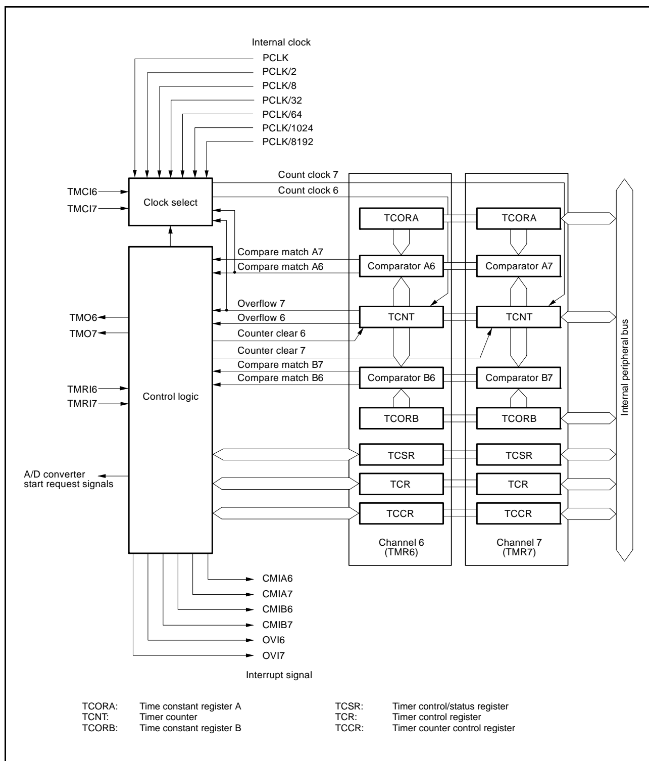
Figure 22.4 Block Diagram of TMR (Unit 3)
