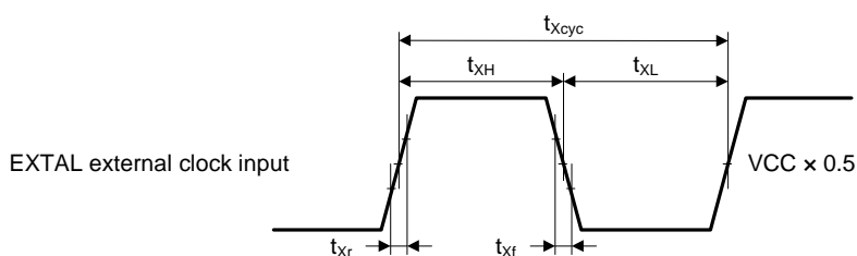
Figure 35.20 EXTAL External Clock Input Timing
