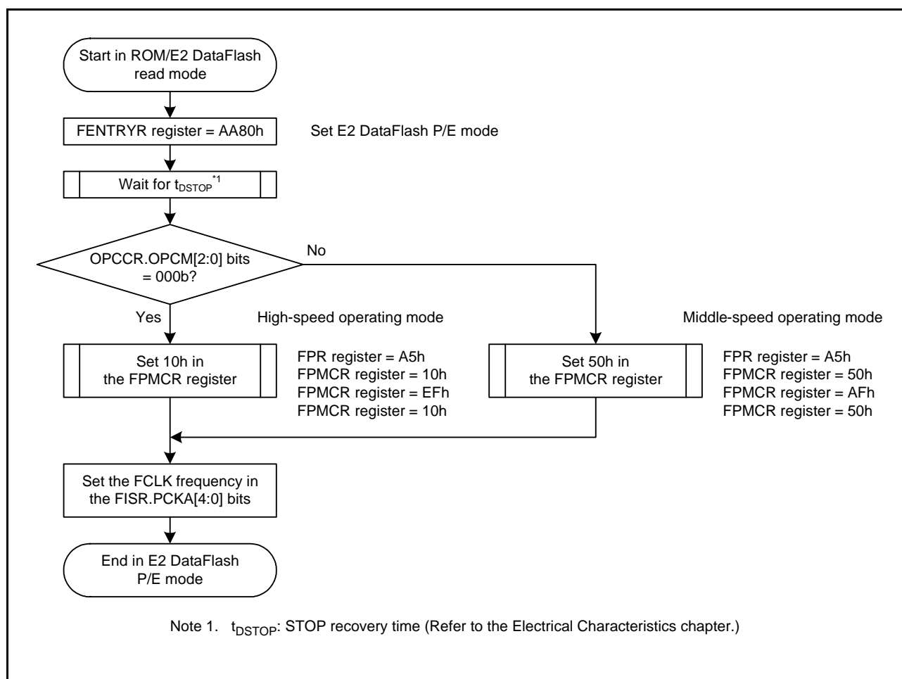
Figure 34.9 Procedure for Transition from ROM/E2 DataFlash Read Mode to E2 DataFlash P/E Mode
