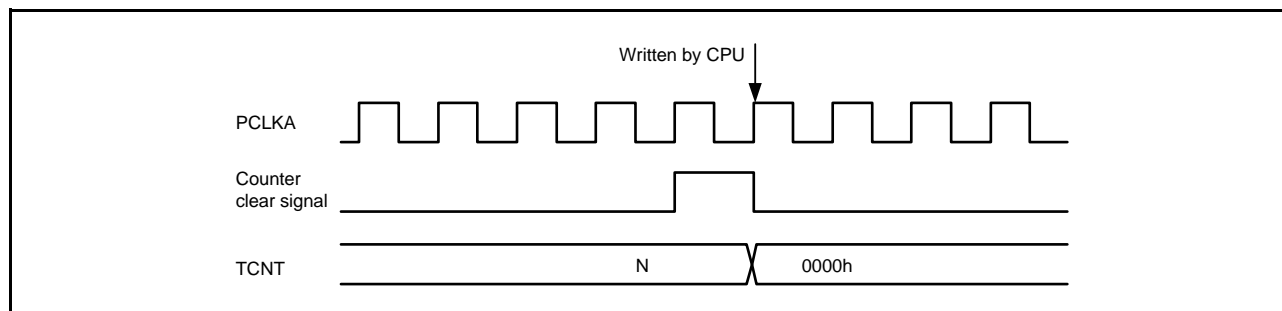
Figure 20.134 Contention between TCNT Write and Clear Operations
