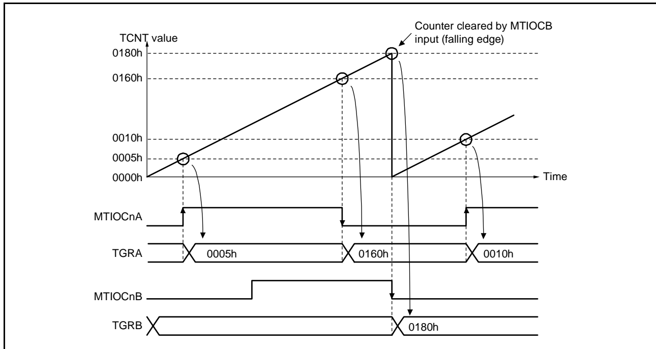
Figure 20.12 Example of Input Capture Operation (n = 0 to 4, 6, 7, 9)
