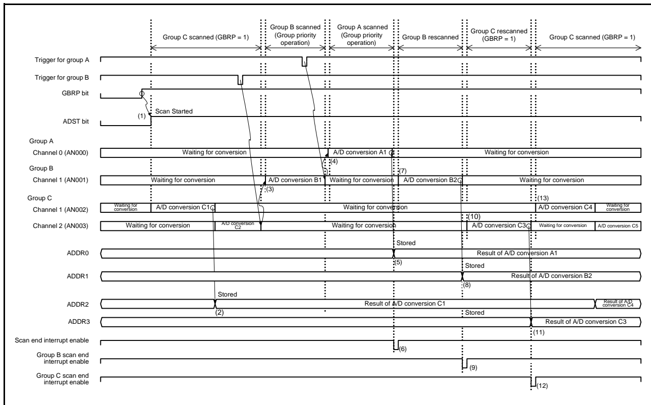
Figure 29.28 Example 5 for Group Priority Operation: Continuous Single Scan Operation on Group C (ADGSPCR.GBRP = 1, ADGSPCR.LGRRS = 1)
