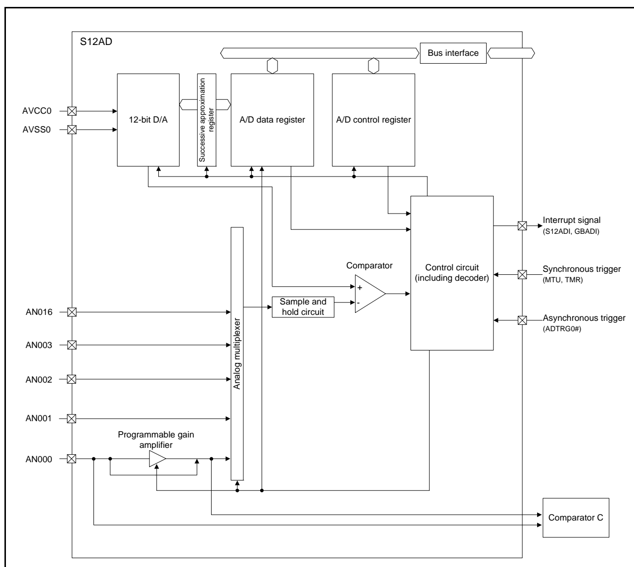
Figure 29.1 Block Diagram of 12-Bit A/D Converter (Unit 0)
