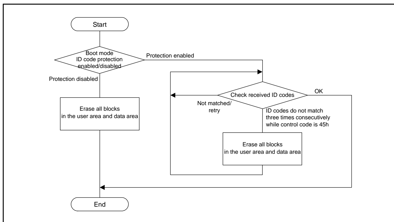
Figure 34.27 Authentication for Boot Mode ID Code Protection
