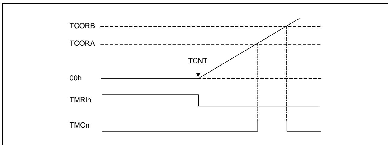
Figure 22.6 Example of External Counter Reset Signal Input (n = 0 to 7)
