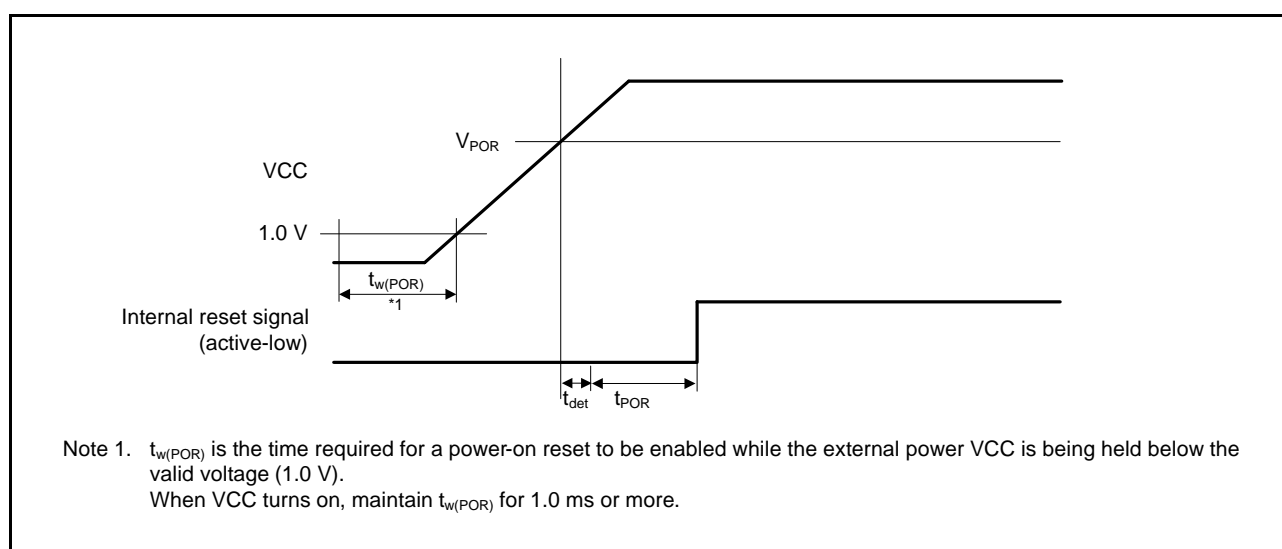
Figure 35.49 Power-On Reset Timing
