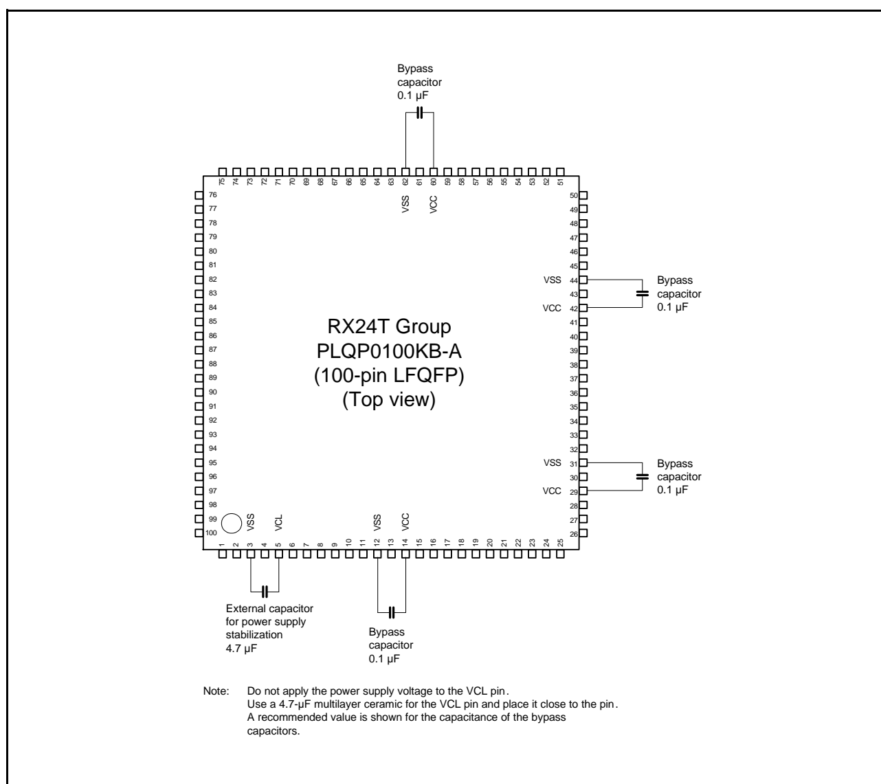
Figure 35.54 Connecting Capacitors (100 Pins)
