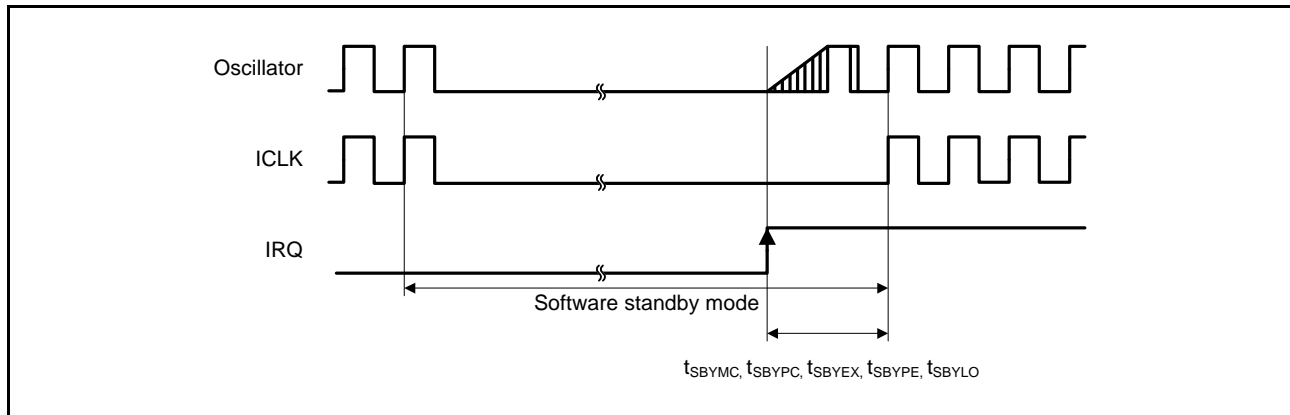
Figure 35.28 Software Standby Mode Recovery Timing
