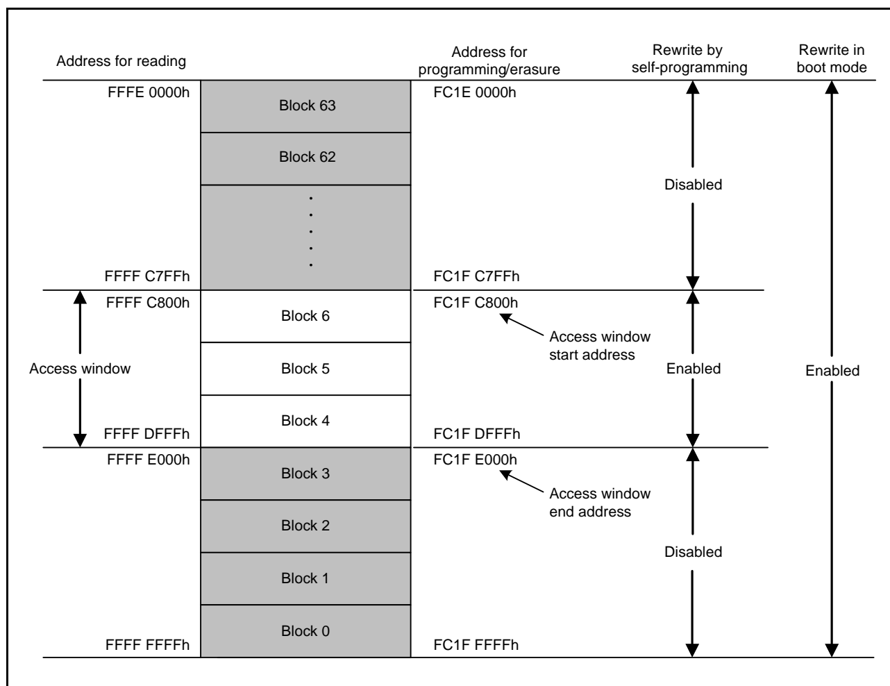
Figure 34.5 Area Protection Overview (When Blocks 4 to 6 are Set as the Access Window in Products with 128-Kbyte ROM)
