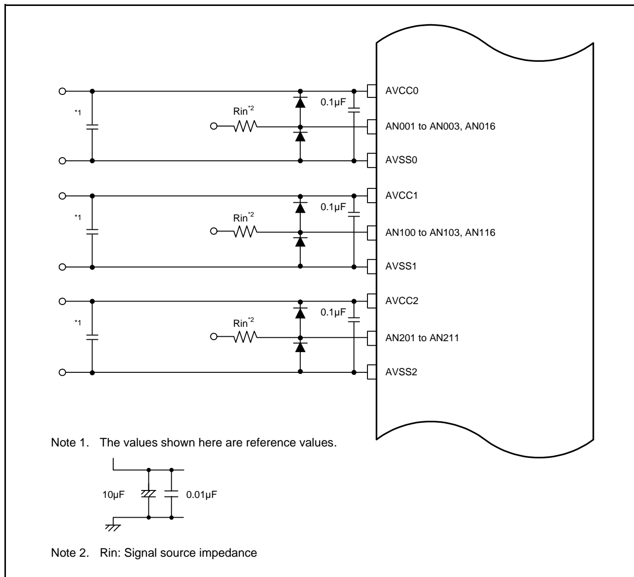
Figure 29.38 Sample Protection Circuit for Analog Inputs
