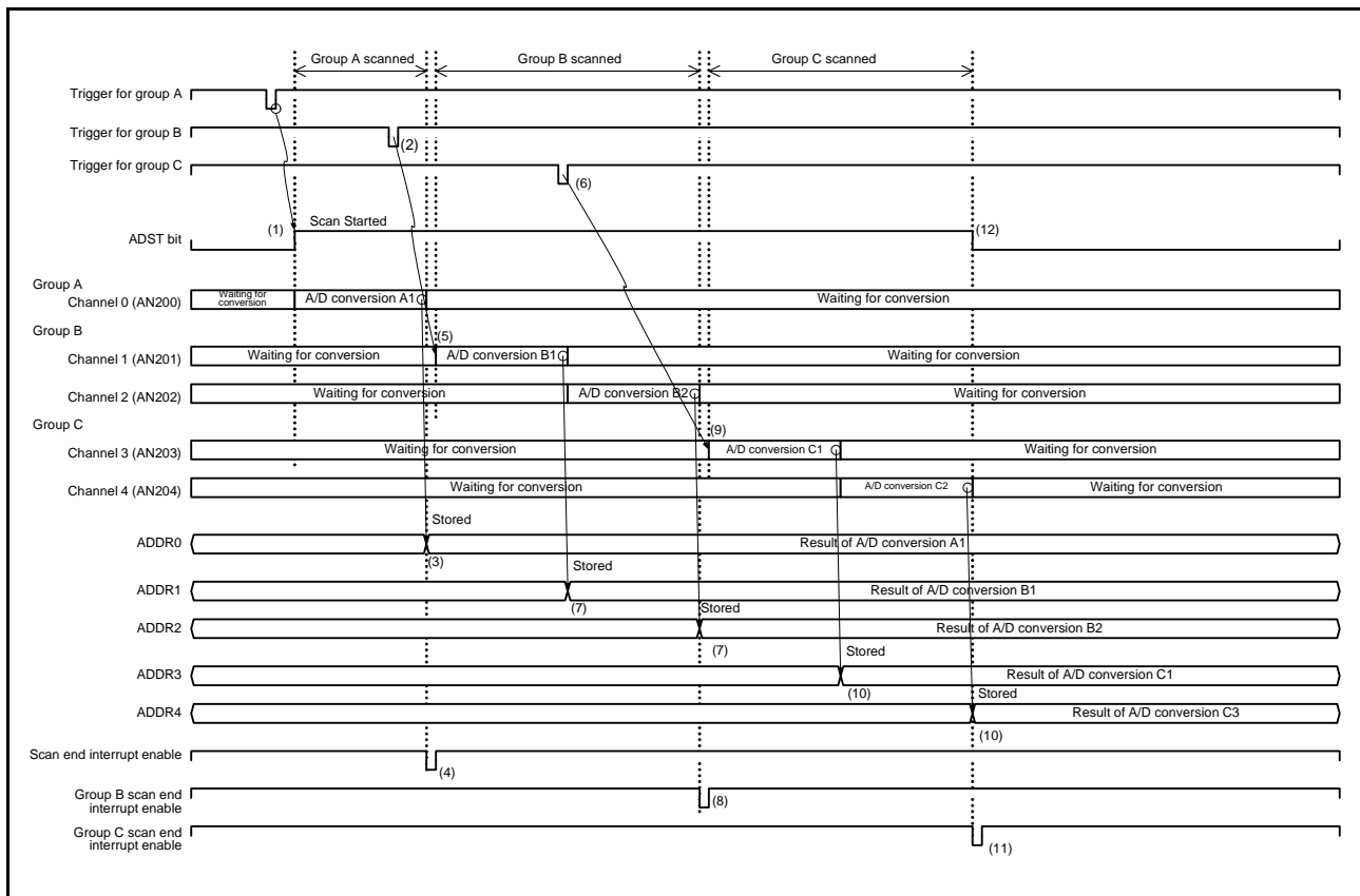
Figure 29.26 Example 3 of Group Priority Operation: Low-Priority Group Trigger Input during Priority Group Scan, With Rescan Setting (ADGSPCR.GBRSCN = 1, ADGSPCR.GBRP = 0, ADGSPCR.LGRRS = 1, ADGCTRGR.GRCE = 1)
