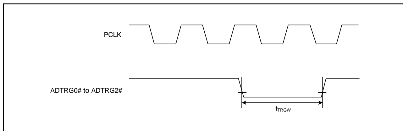
Figure 35.39 A/D Converter External Trigger Input Timing
