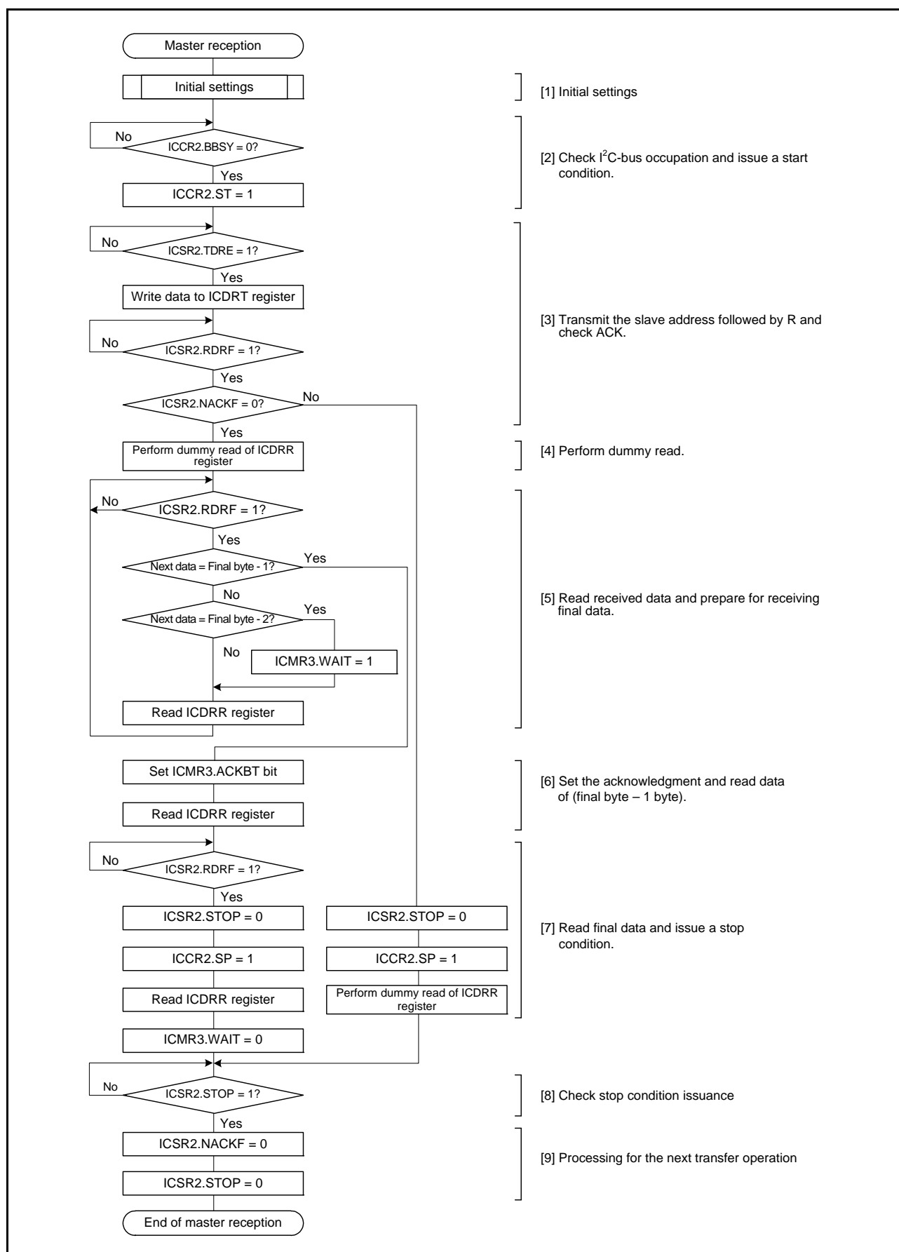
Figure 26.11 Example of Master Reception (7-Bit Address Format, 3 Bytes or More)
