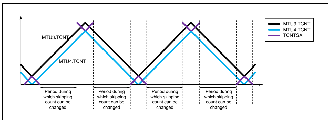
Figure 20.86 Periods during which Interrupt Skipping Count can be Changed
