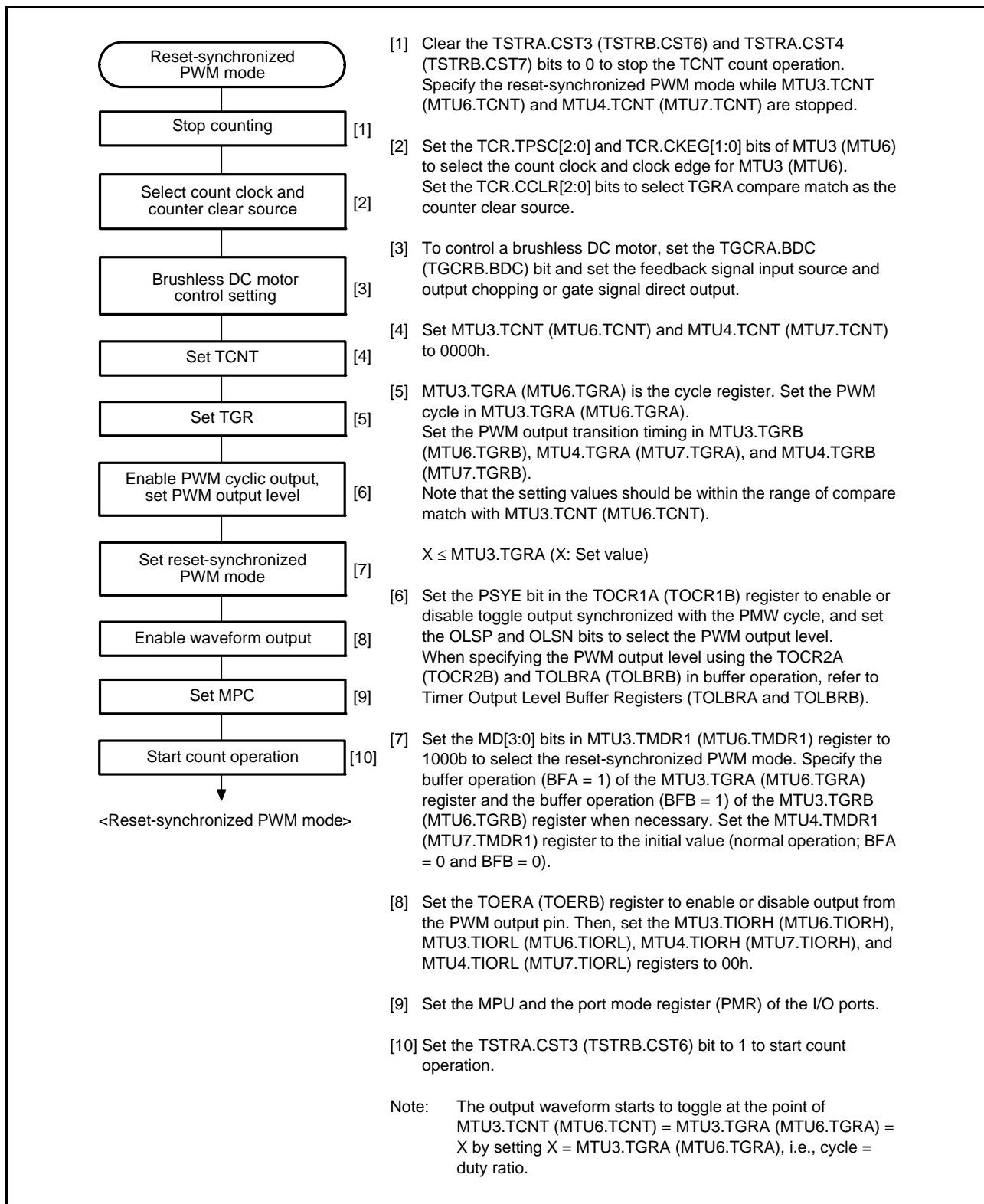
Figure 20.43 Procedure for Selecting Reset-Synchronized PWM Mode
