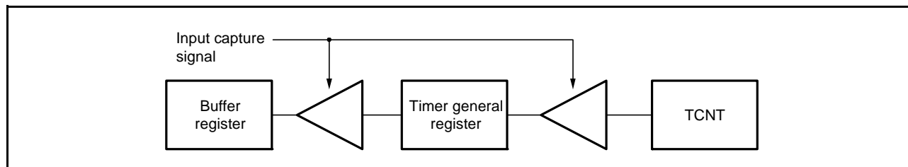
Figure 20.16 Input Capture Buffer Operation
