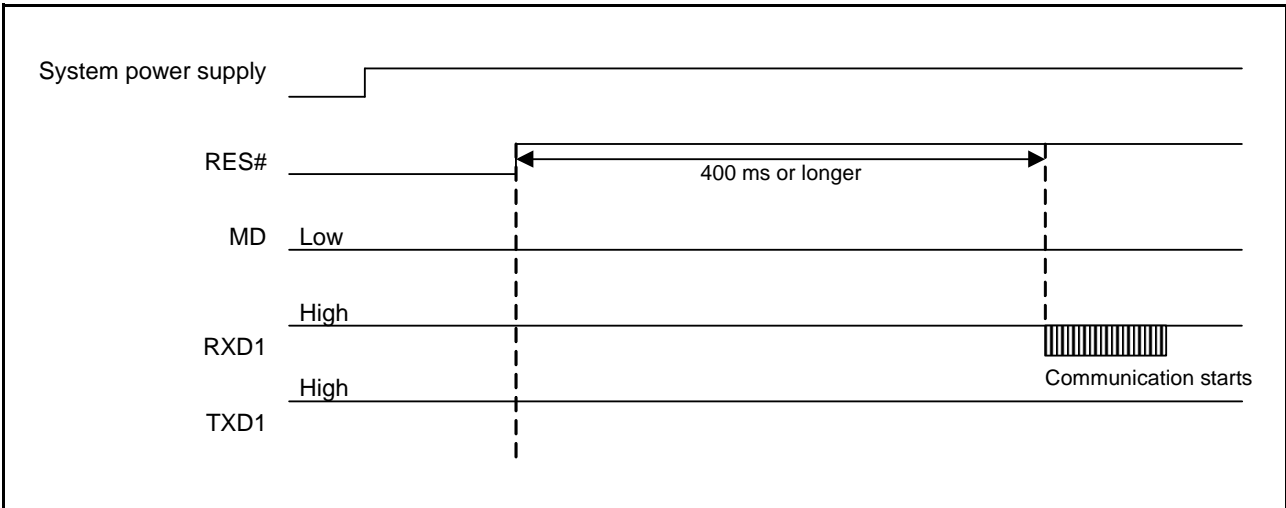
Figure 34.24 Wait Time until Communication Becomes Possible in Boot Mode (SCI)
