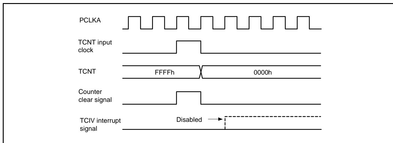
Figure 20.147 Contention between Overflow and Counter Clearing
