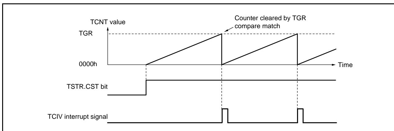
Figure 20.7 Periodic Counter Operation
