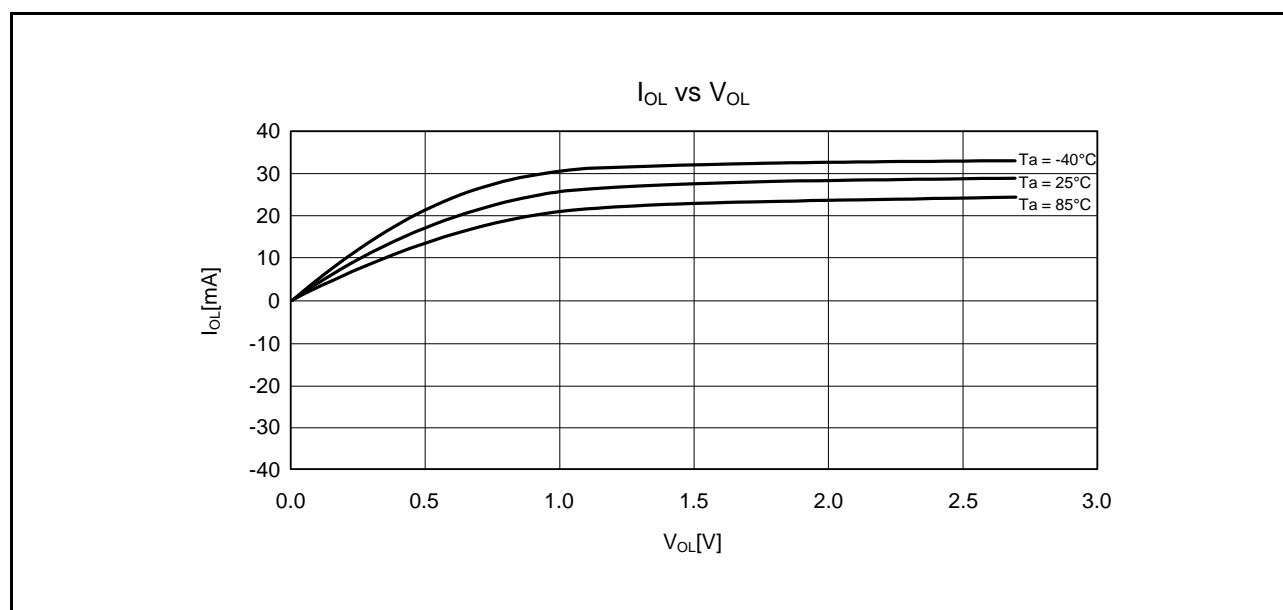
Figure 35.17 V OL and I OL Temperature Characteristics of RIIC Output Pin at V CC = 2.7 V (Reference Data)
