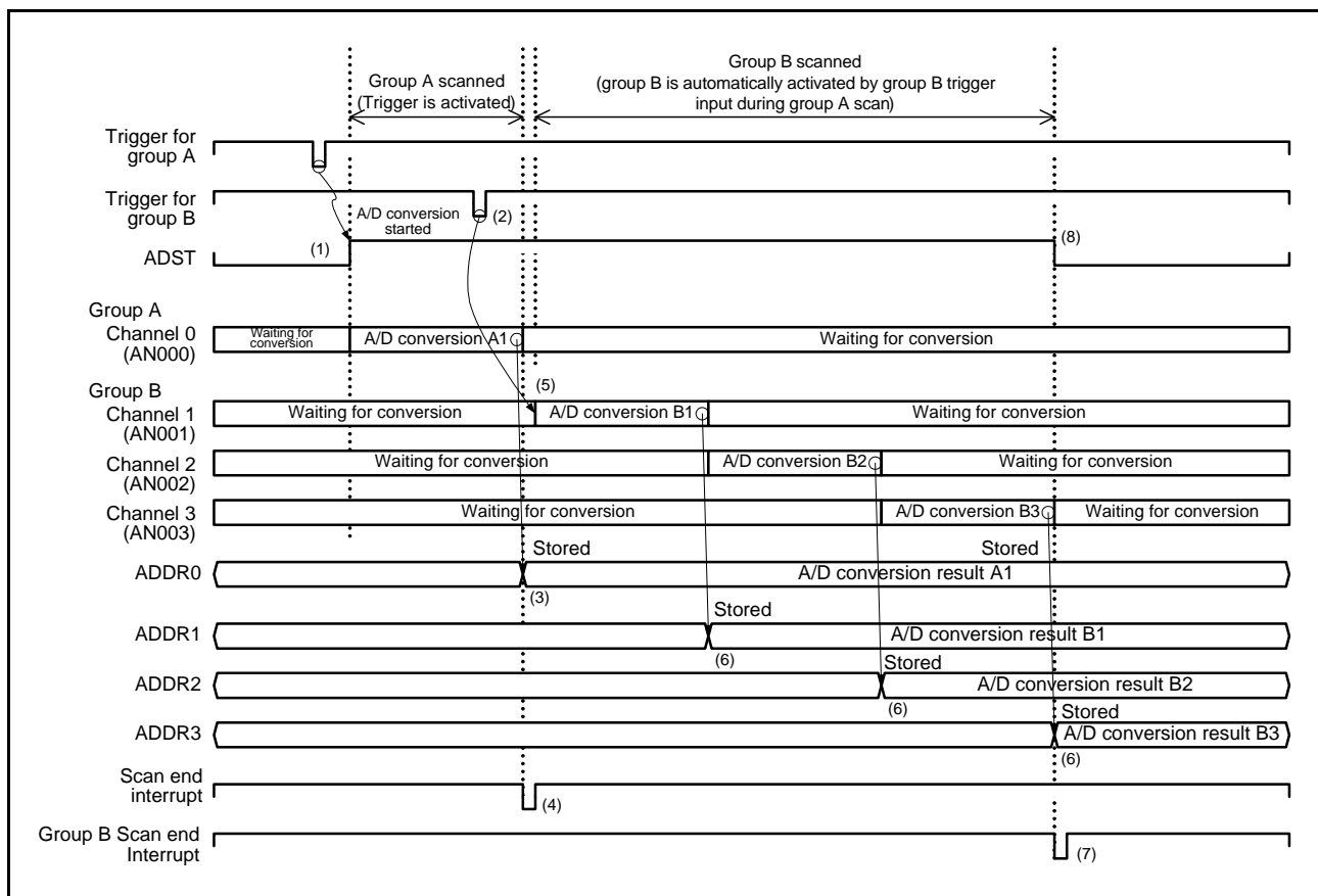
Figure 29.21 Example 3 of Group Priority Operation: Group B Trigger Input during Group A Scan, With Rescan Setting (ADGPSCR.GBRSCN = 1, ADGPSCR.GBRP = 0, ADGPSCR.LGRRS = 0)
