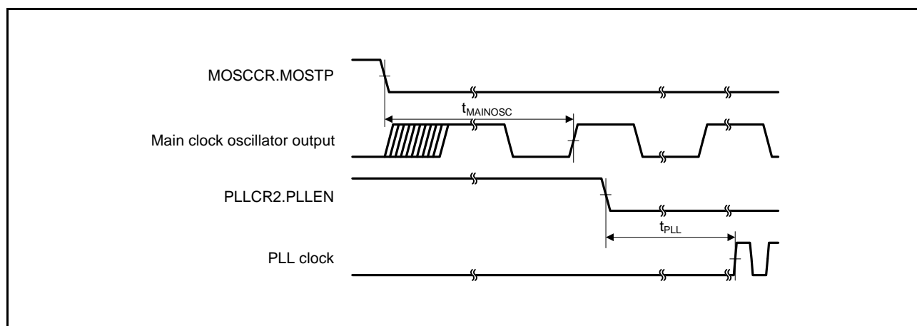
Figure 35.24 PLL Clock Oscillation Start Timing (PLL is Operated after Main Clock Oscillation Has Settled)
