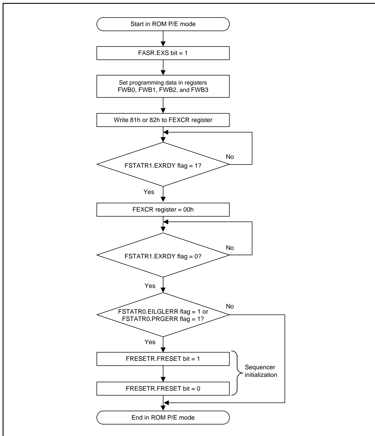
Figure 34.20 Procedure to Issue the Start-Up Area Information Program Command/Access Window Information Program Command
