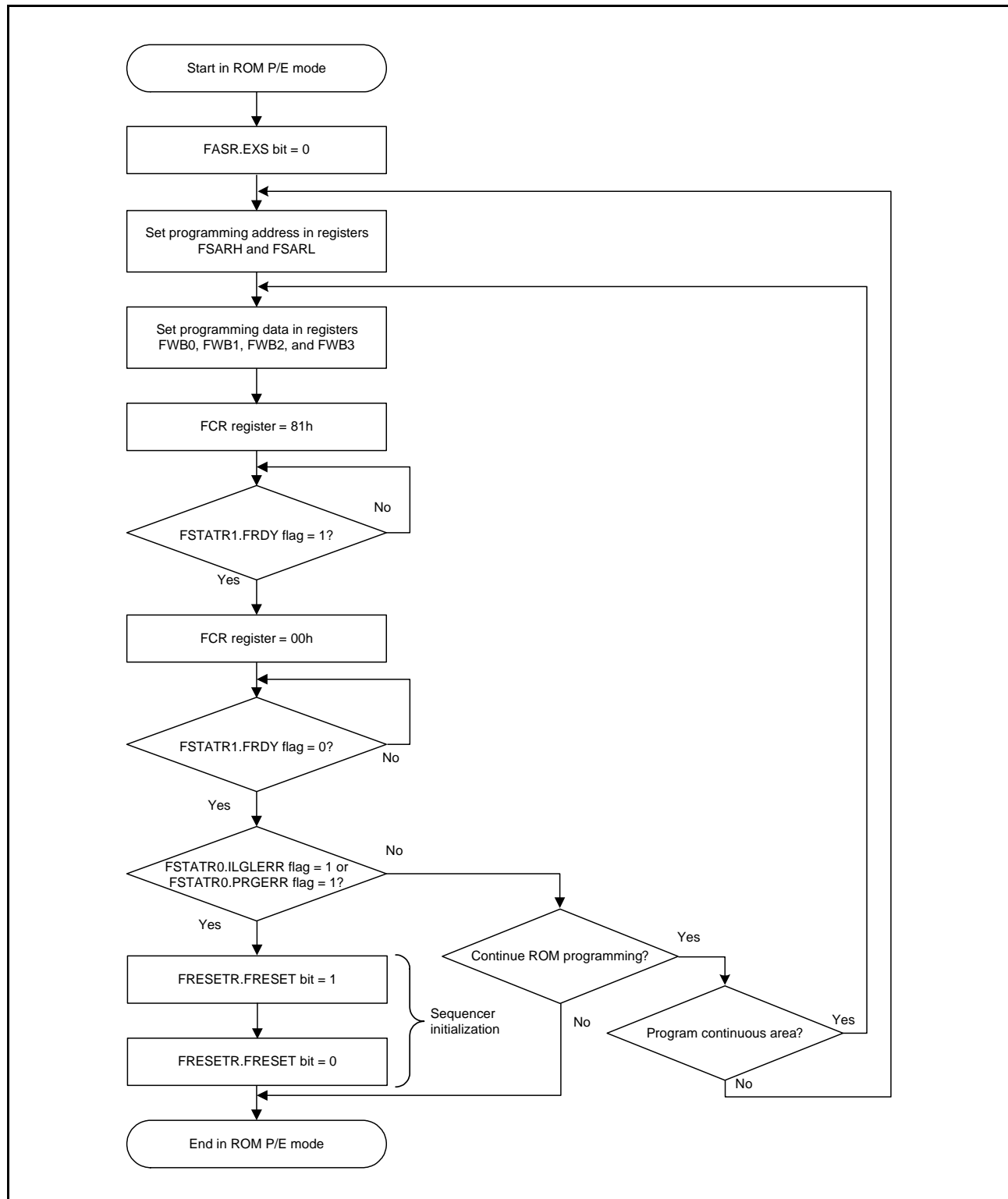
Figure 34.12 Procedure to Issue the Program Command for the ROM
