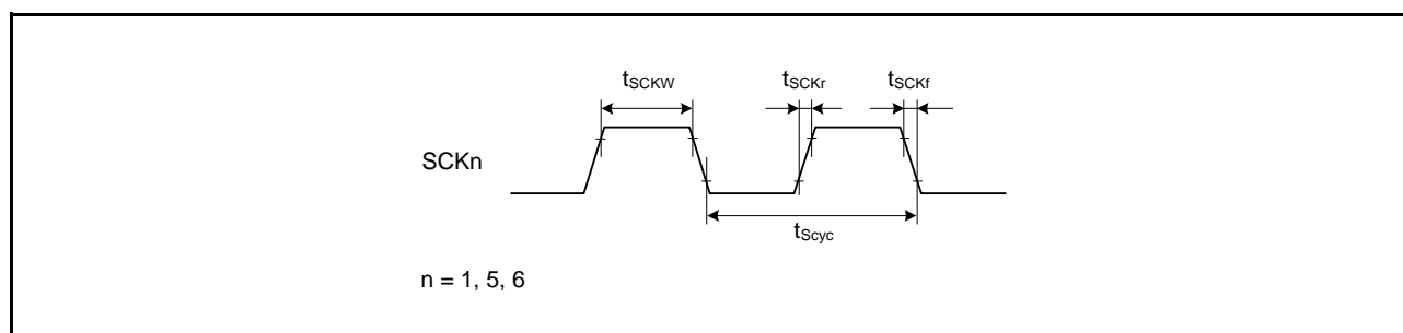
Figure 35.37 SCK Clock Input Timing
