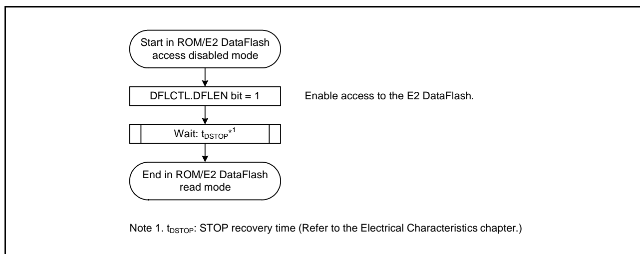
Figure 34.7 Procedure for Transition from E2 DataFlash Access Disabled Mode to ROM/E2 DataFlash Read Mode
