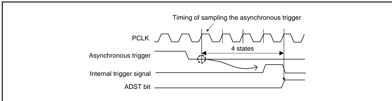
Figure 29.34 Timing of Sampling Asynchronous Trigger
