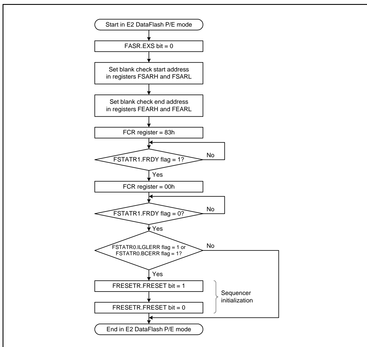
Figure 34.19 Procedure to Issue the Blank Check Command for the E2 DataFlash
