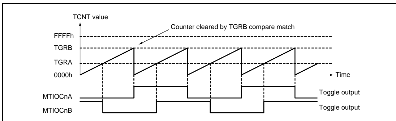
Figure 20.10 Example of Toggle Output Operation (n = 0 to 4, 6, 7, 9)
