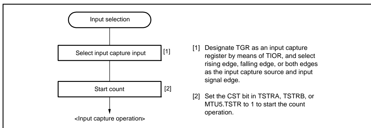
Figure 20.11 Example of Input Capture Operation Setting Procedure
