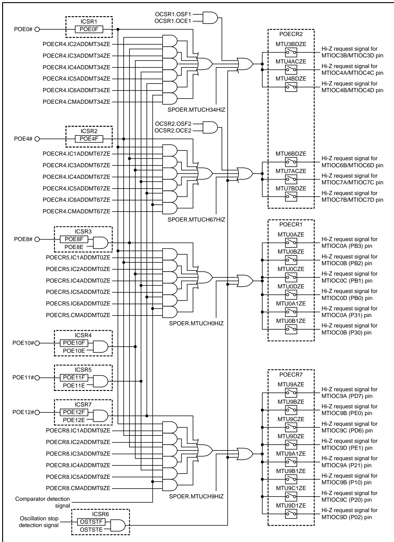
Figure 21.2 Target Pins and Conditions for High-Impedance Control
