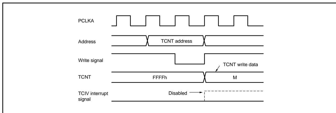
Figure 20.148 Contention between TCNT Write Operation and Overflow
