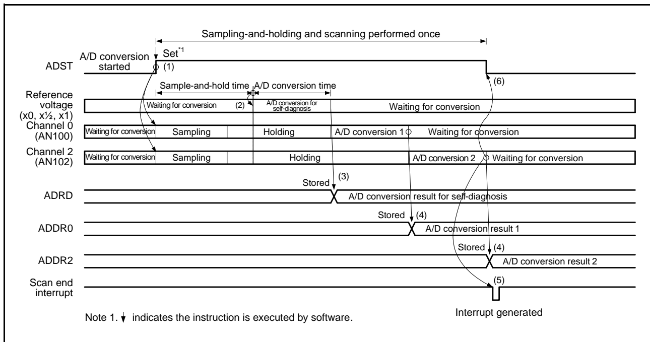
Figure 29.8 Example of Operation in Continuous Scan Mode (Channel-Dedicated Sample-and-Hold Circuits Used: AN100, AN102 Selected + Self-Diagnosis)
