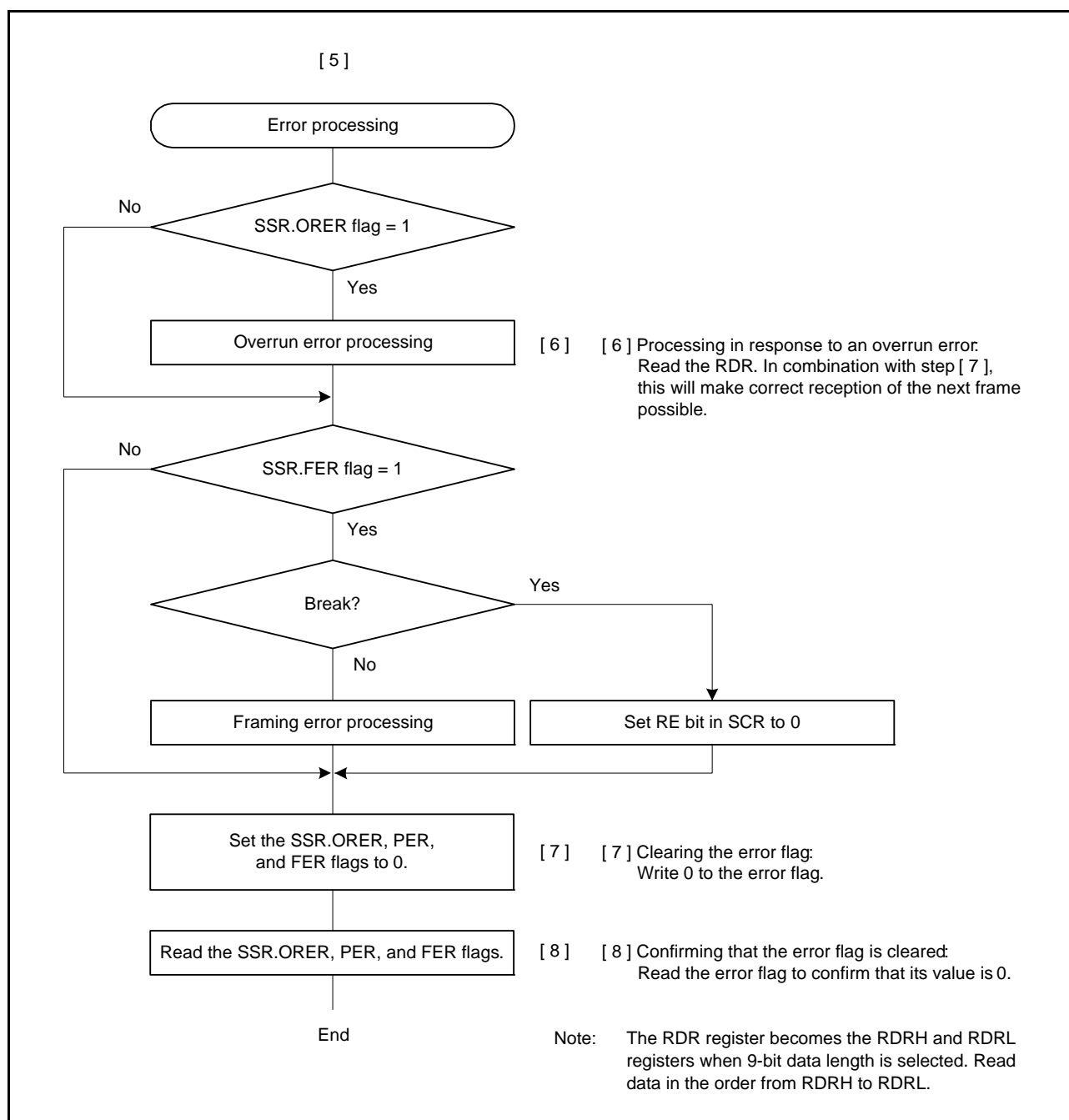
Figure 25.20 Example of Multi-Processor Serial Reception Flowchart (2)
