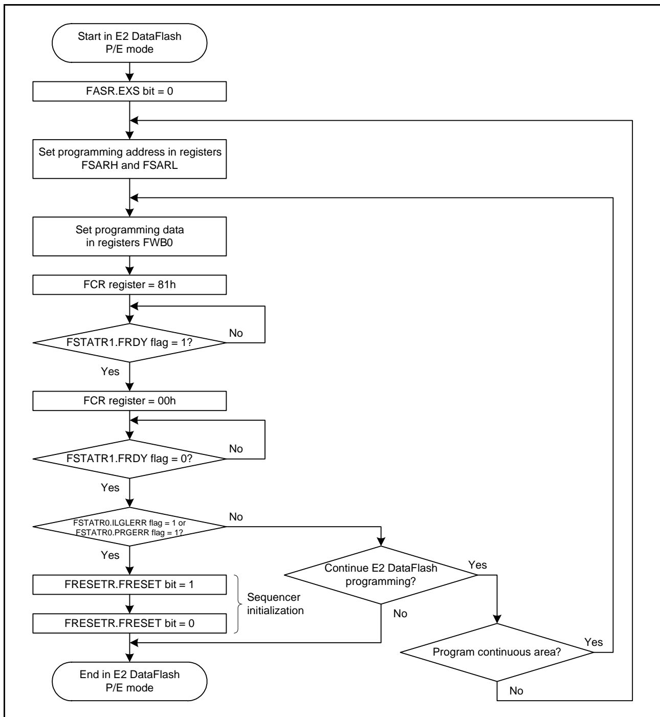
Figure 34.13 Procedure to Issue the Program Command for the E2 DataFlash
