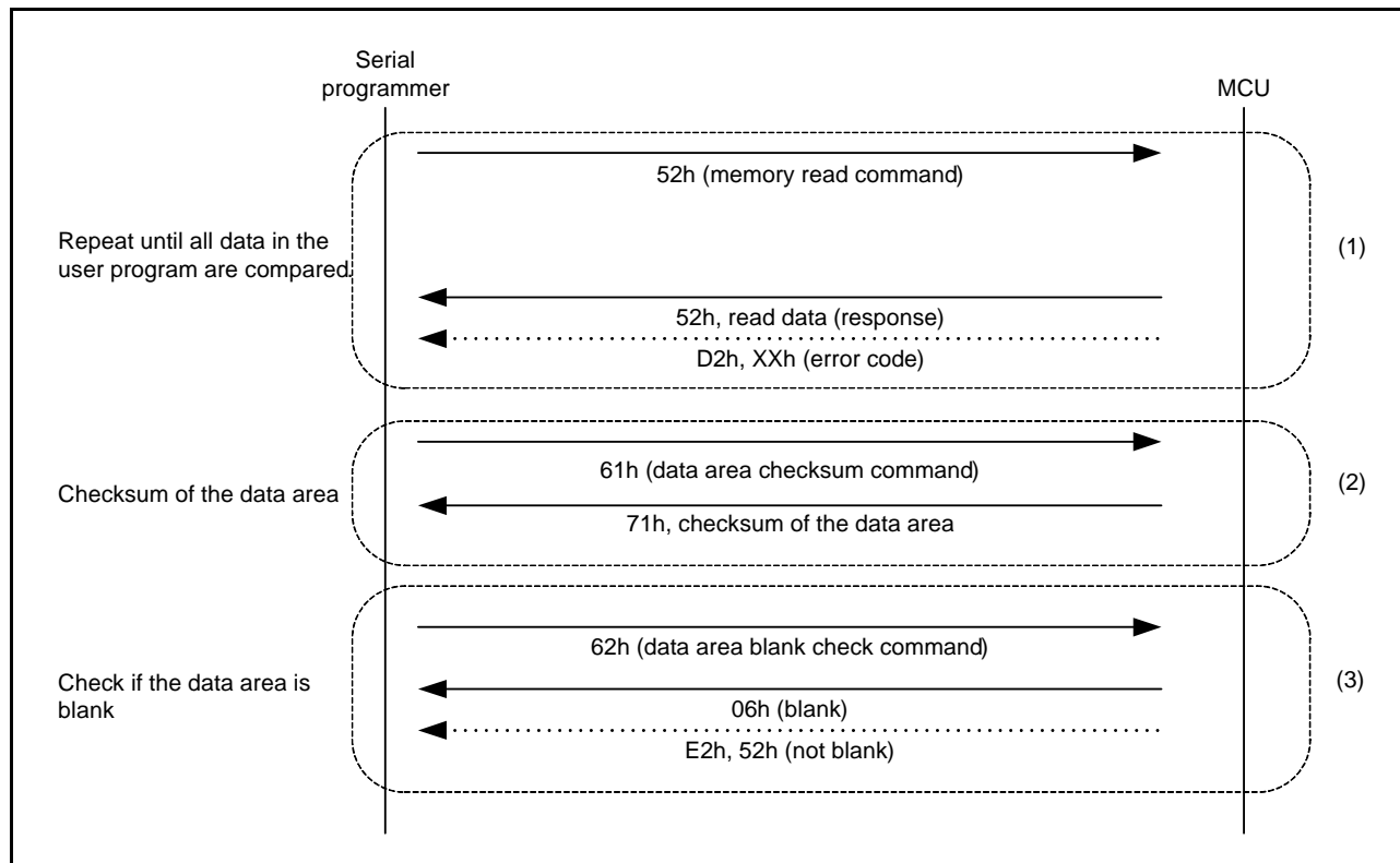
Figure 34.39 Procedure to Check Data in the Data Area
