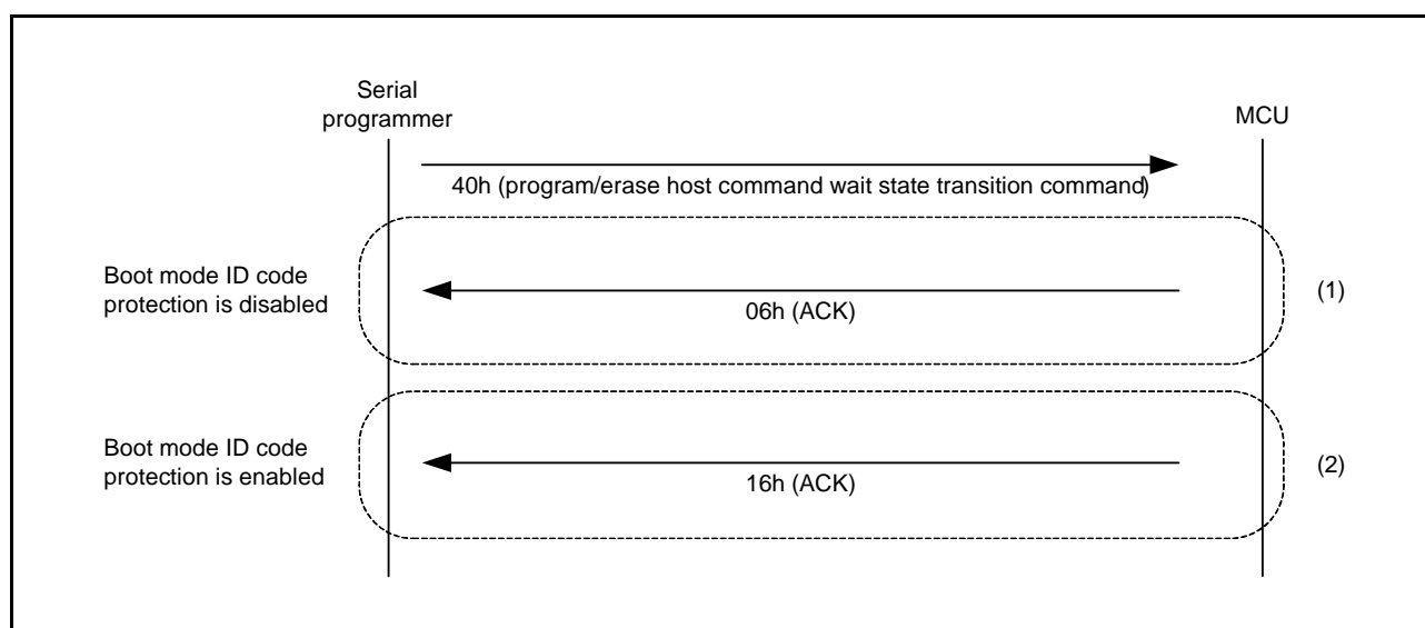
Figure 34.34 Procedure to Enter the Program/Erase Host Command Wait State
