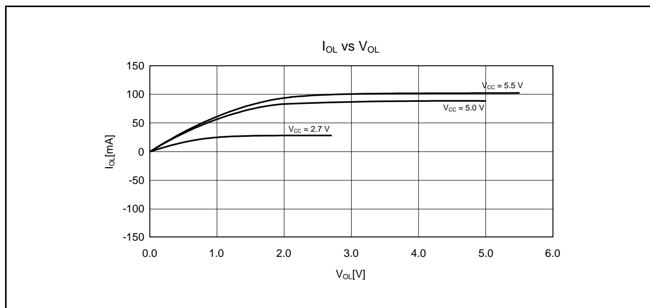
Figure 35.16 V OL and I OL Voltage Characteristics of RIIC Output Pin at T a = 25°C (Reference Data)
