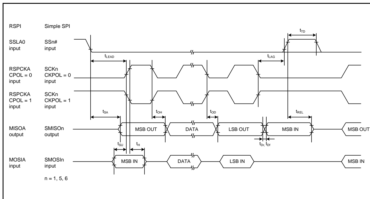
Figure 35.43 RSPI Timing (Slave, CPHA = 0) and Simple SPI Clock Timing (Slave, CKPH = 1)
