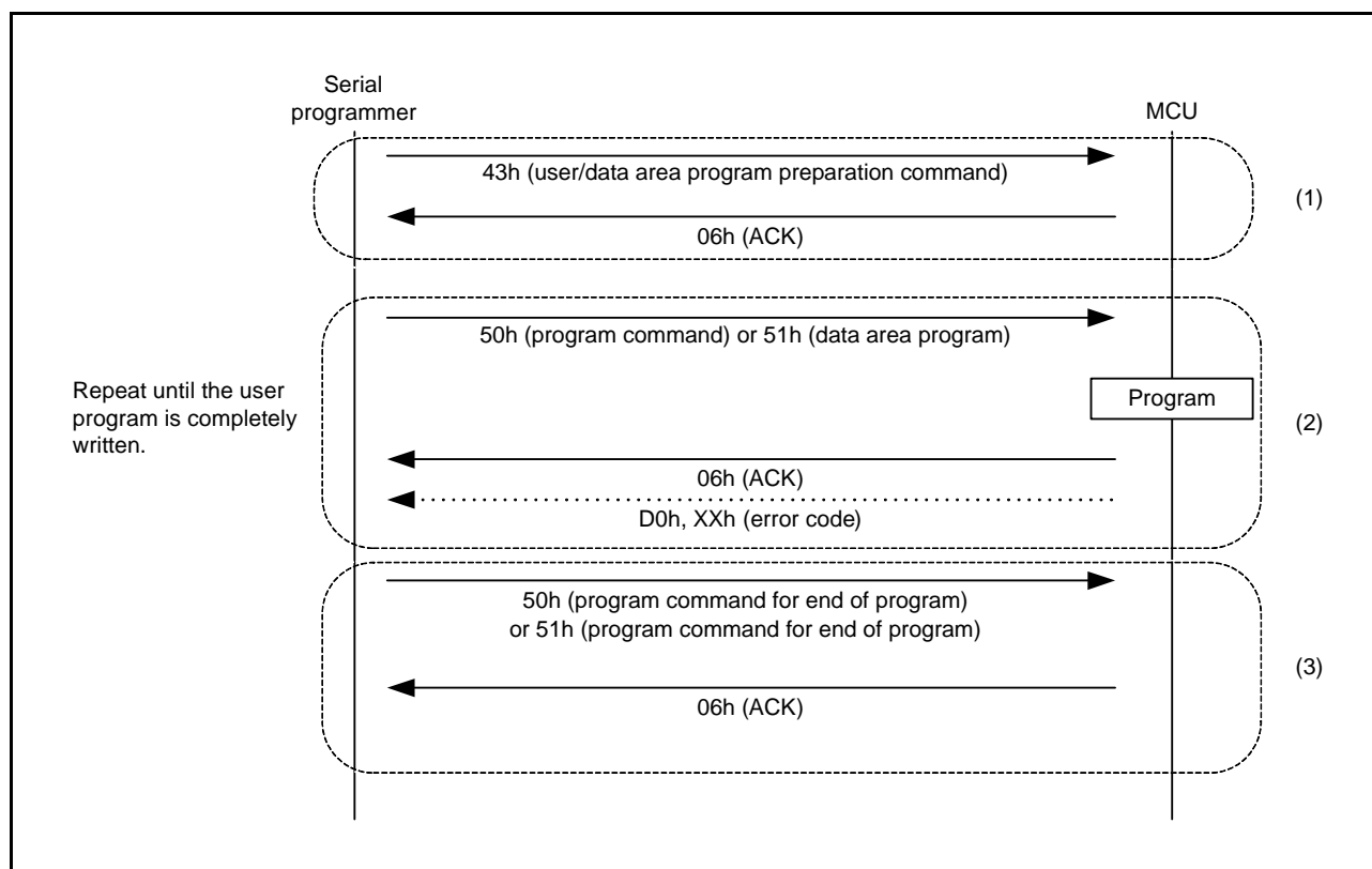
Figure 34.37 Procedure to Program the User Area and Data Area
