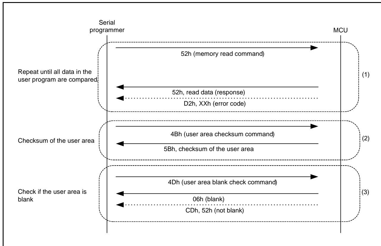
Figure 34.38 Procedure to Check Data in the User Area
