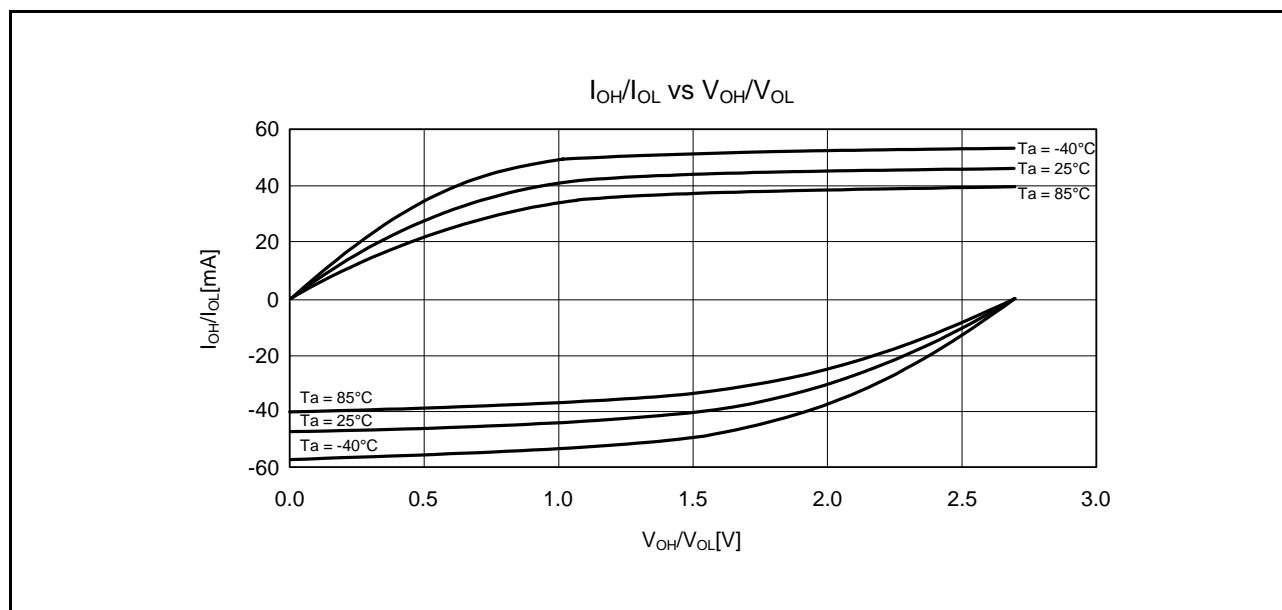
Figure 35.13 V_{OH}/V_{OL} and I_{OH}/I_{OL} Temperature Characteristics of Large Current Ports at V_{CC} = 2.7\text{ V} (Reference Data)
