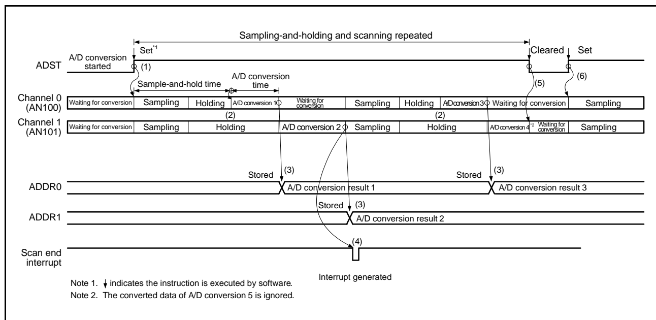
Figure 29.13 Example of Operation in Continuous Scan Mode (Channel-Dedicated Sample-and-Hold Circuits Used)
