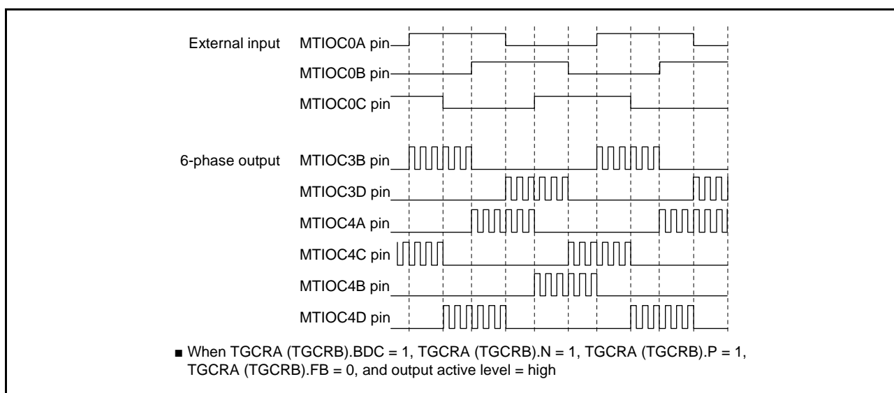
Figure 20.79 Example of Output Phase Switching by External Input (2)
