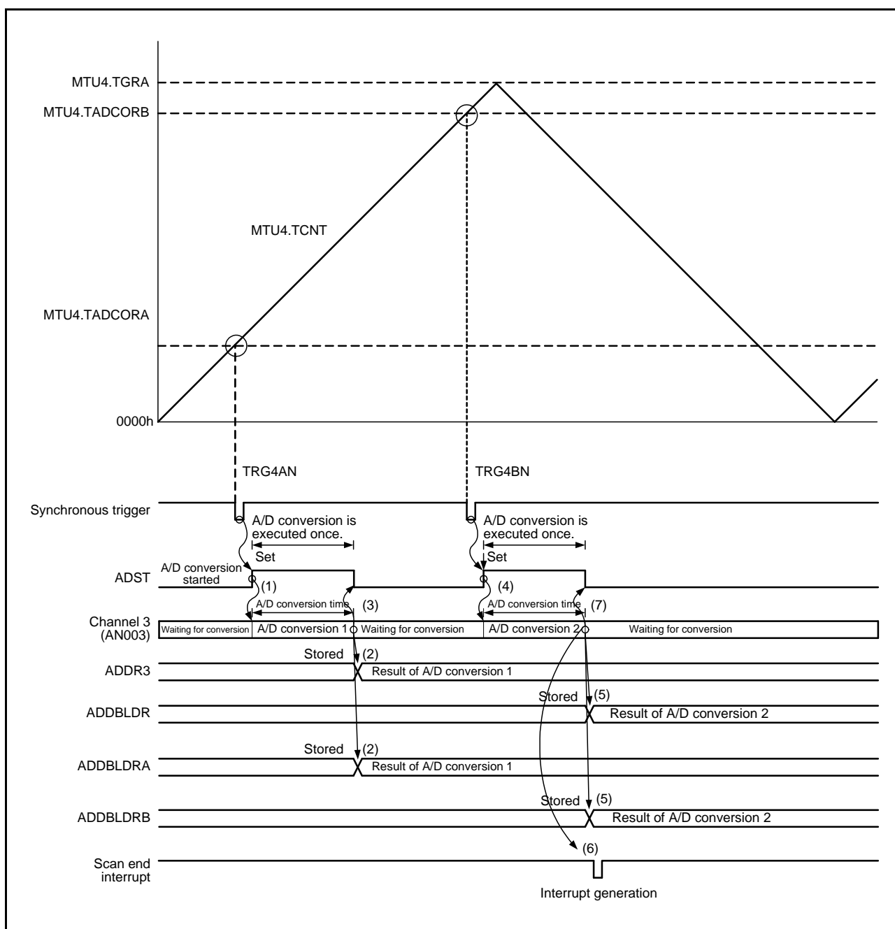
Figure 29.11 Example of Extended Operation in Double Trigger Mode (1) (Duplication Selected for AN003, TRG4AN or TRG4BN Selected, First Trigger is TRG4AN)
