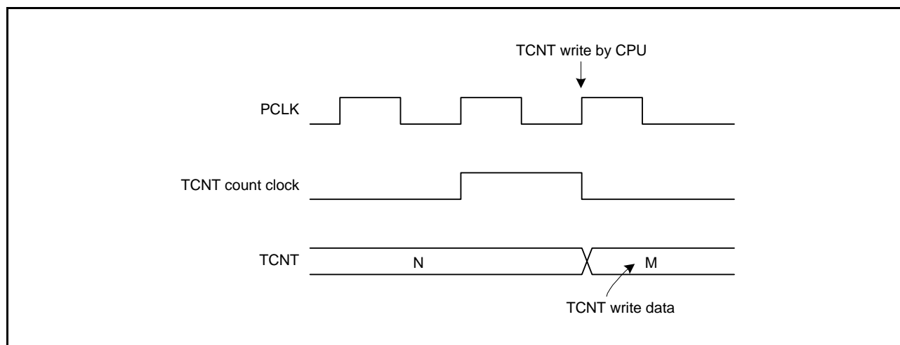
Figure 22.16 Conflict between TCNT Write and Increment
