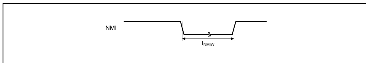
Figure 35.30 NMI Interrupt Input Timing
