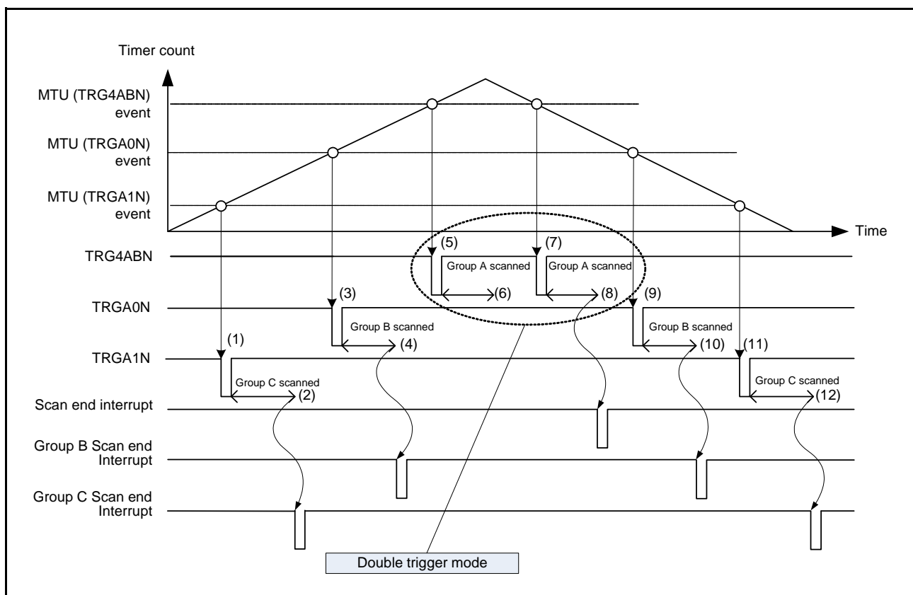
Figure 29.17 Example of Operation in Group Scan Mode with Double Trigger Mode (Basic Operation: Synchronous Triggers from MTU Used)
