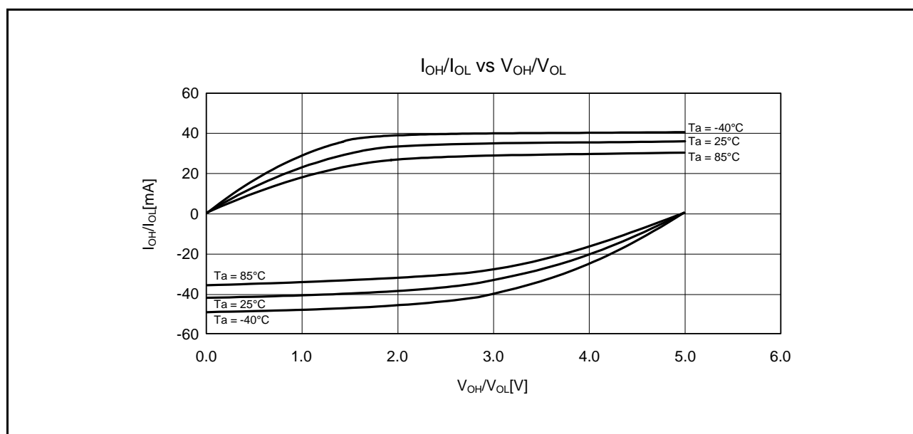
Figure 35.6 V_{OH}/V_{OL} and I_{OH}/I_{OL} Temperature Characteristics at V_{CC} = 5.0 V when Normal Output is Selected (Reference Data)
