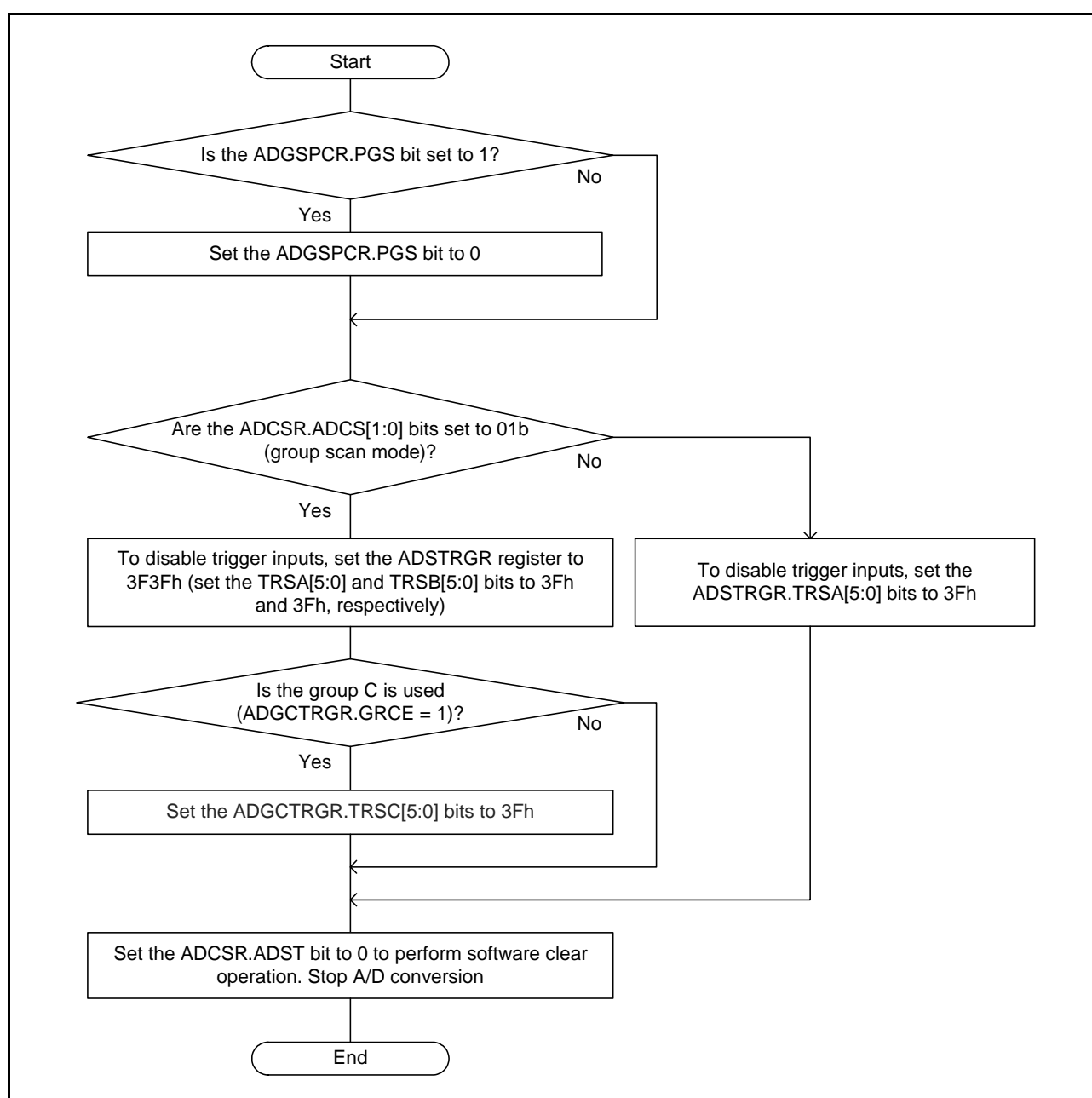
Figure 29.36 Procedure for Clear Operation by Software through the ADCSR.ADST Bit
