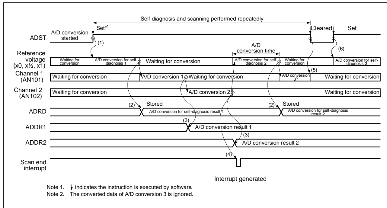
Figure 29.14 Example of Operation in Continuous Scan Mode (Basic Operation; AN101 and AN102 Selected + Self-Diagnosis)
