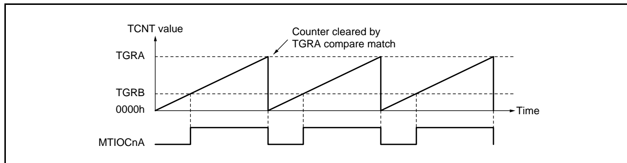
Figure 20.27 Example of PWM Mode 1 Operation (n = 0 to 4, 6, 7, 9)
