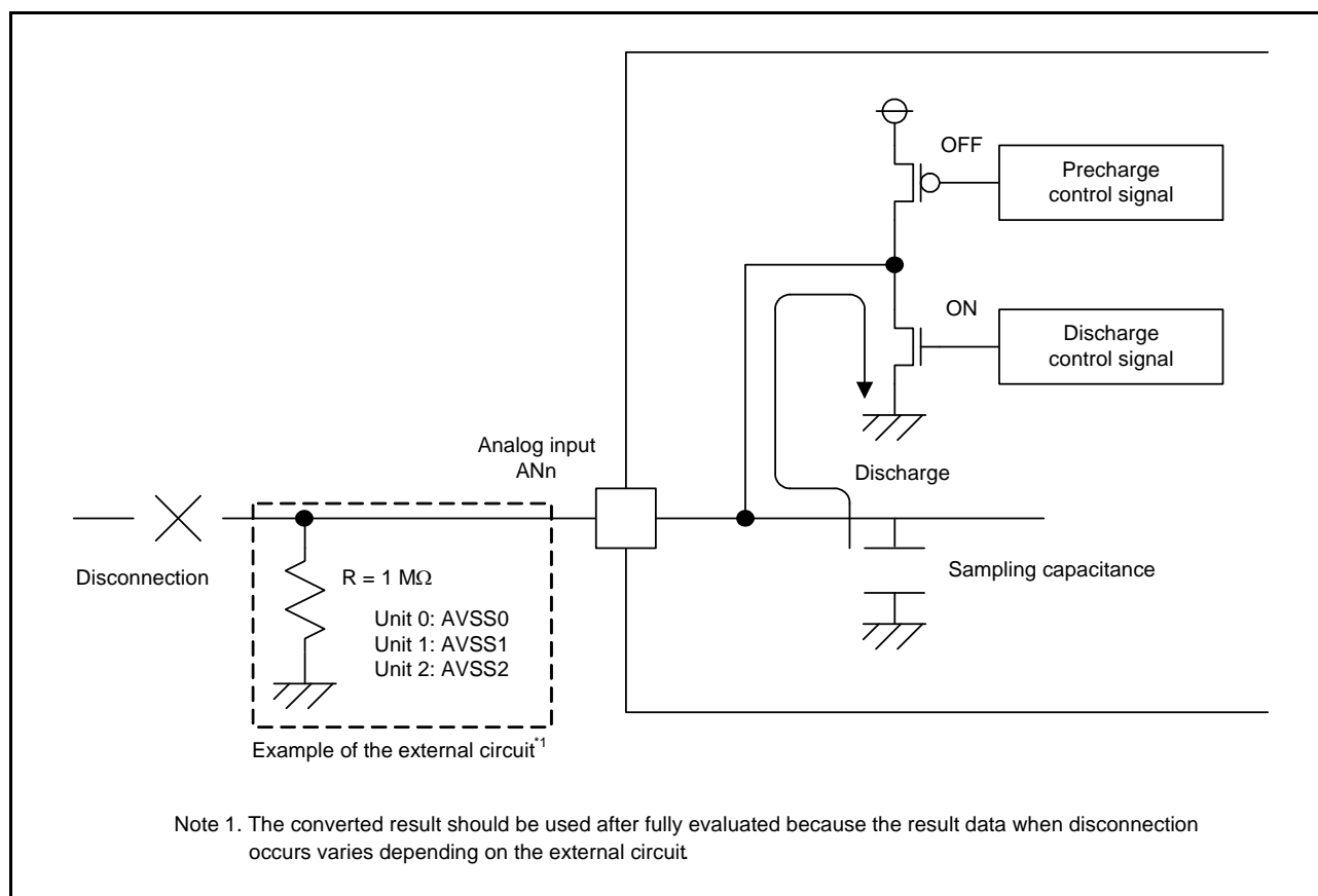
Figure 29.33 Example of Disconnection Detection When Discharge is Selected
