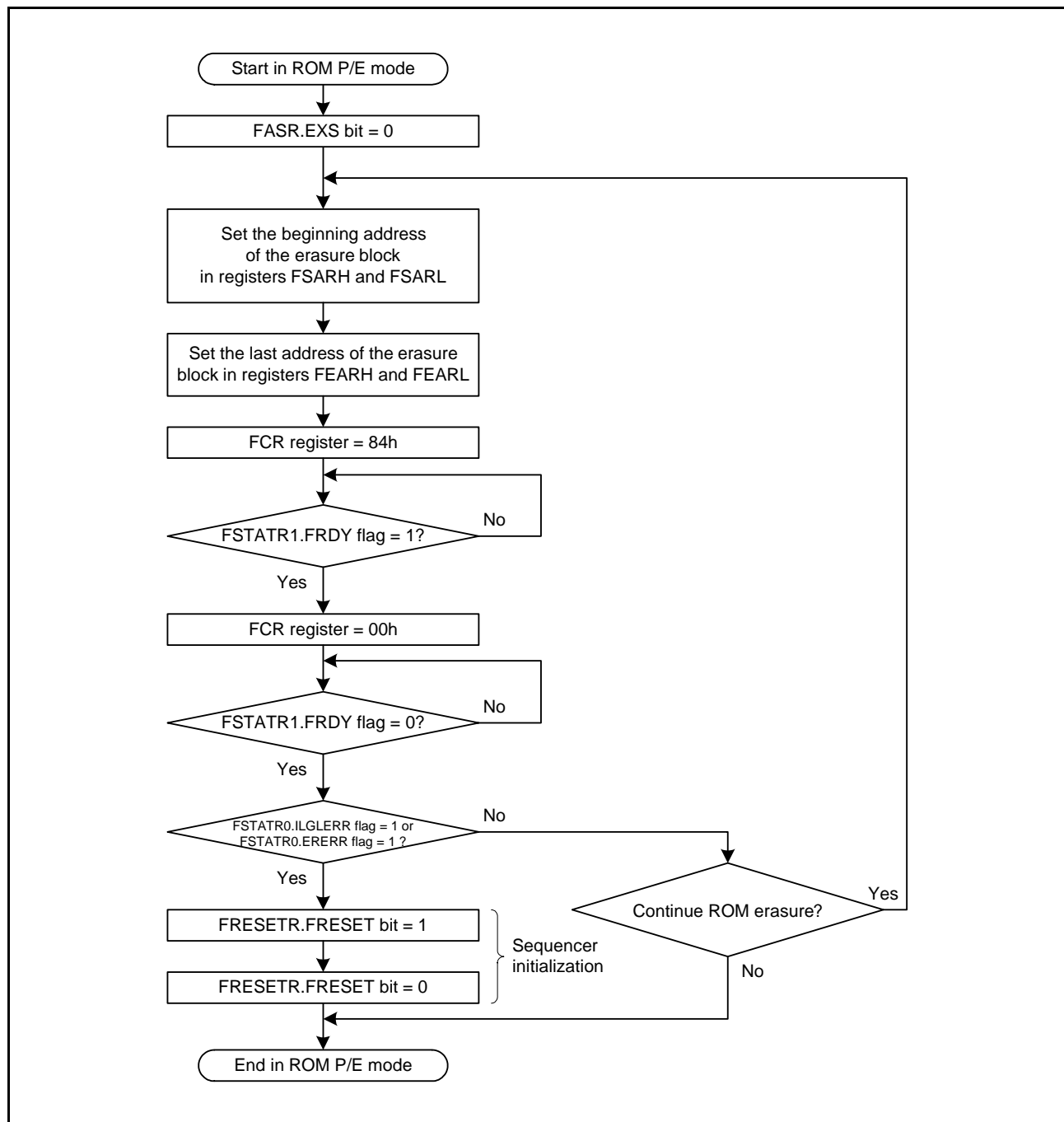
Figure 34.14 Procedure to Issue the Block Erase Command for the ROM
