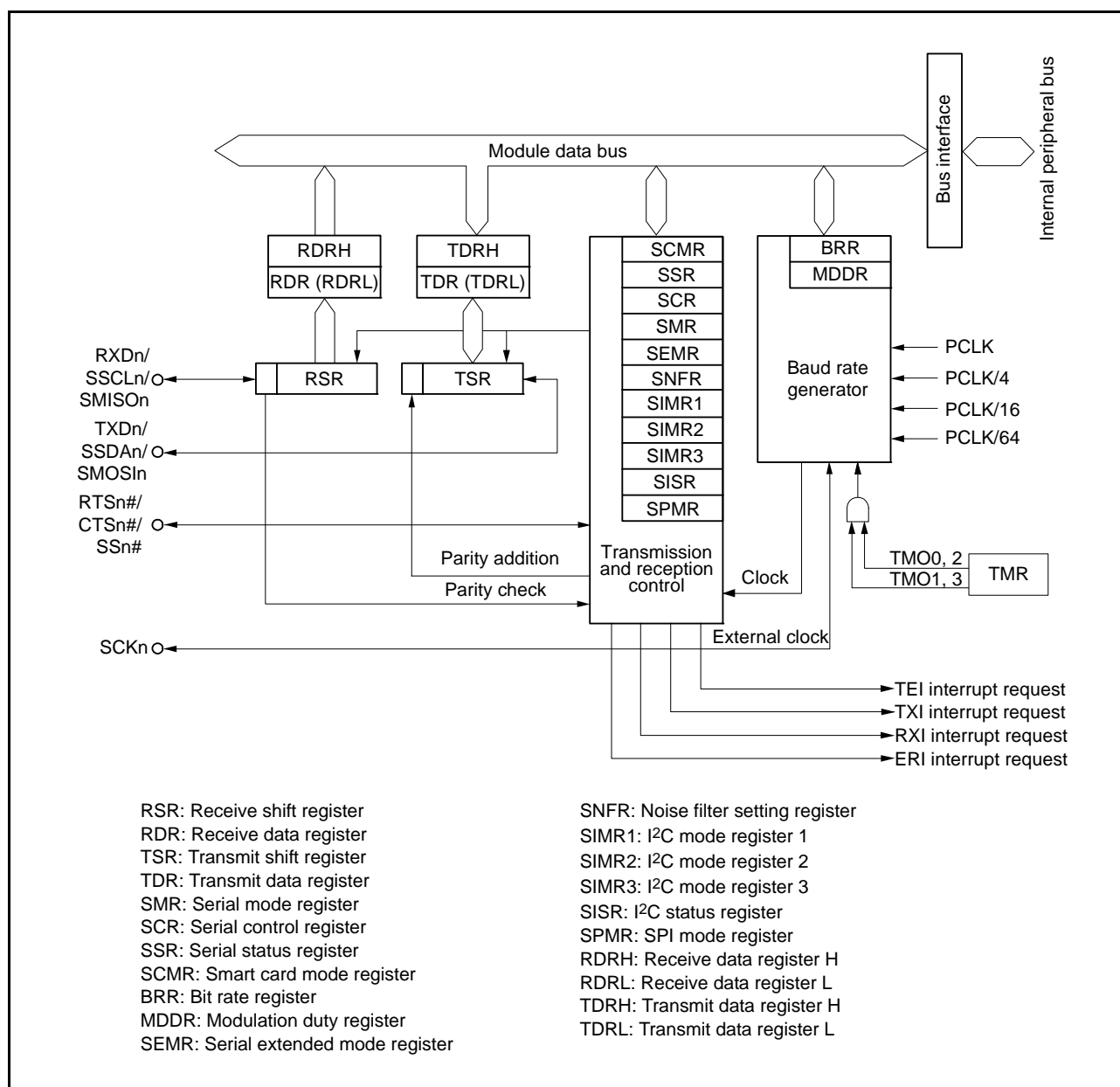
Figure 25.2 Block Diagram of SCIg (SCI5 and SCI6)
