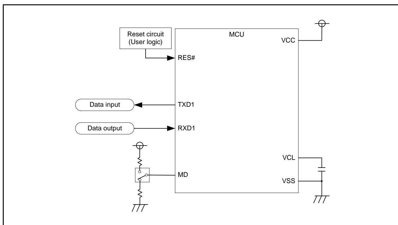
Figure 34.22 Example of Pin Connections in Boot Mode (SCI)
