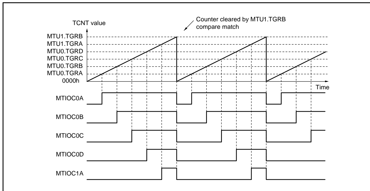
Figure 20.28 Example of PWM Mode 2 Operation
