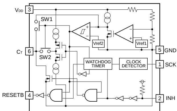
R5106Nxx1C (CMOS Output)
