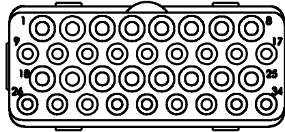
MATING FACE
