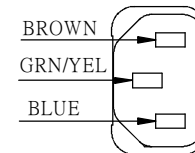
IEC-60320-C13
