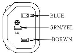
IEC-60320-C14
