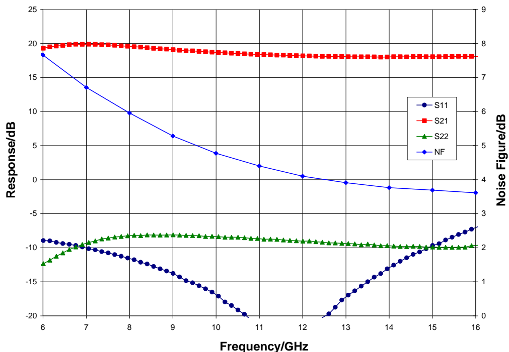
Narrow-band Performance, V_{dd} = 5.0\text{ V} , T_A = 25\text{ °C}
