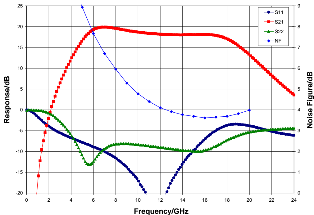
Broadband Performance, V_{dd} = 5.0\text{ V} , T_A = 25\text{ °C}
