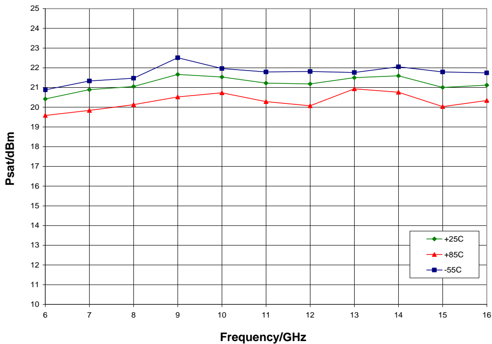
Psat vs. Temperature, V_{dd} = 5.0 V
