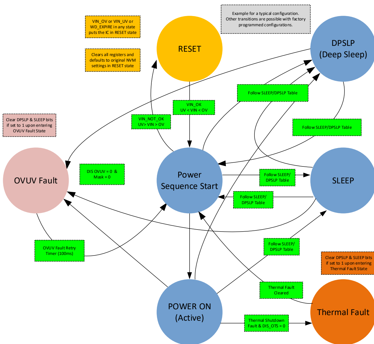
Figure 4: State Machine
