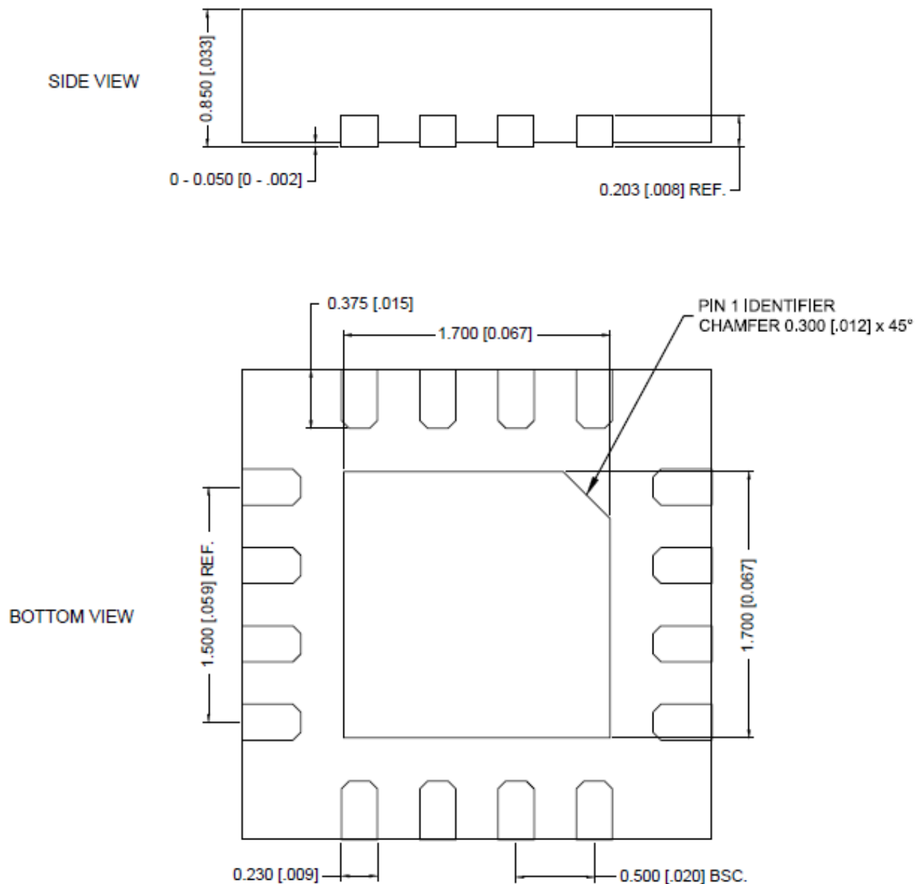
3 x 3 16-pin QFN
