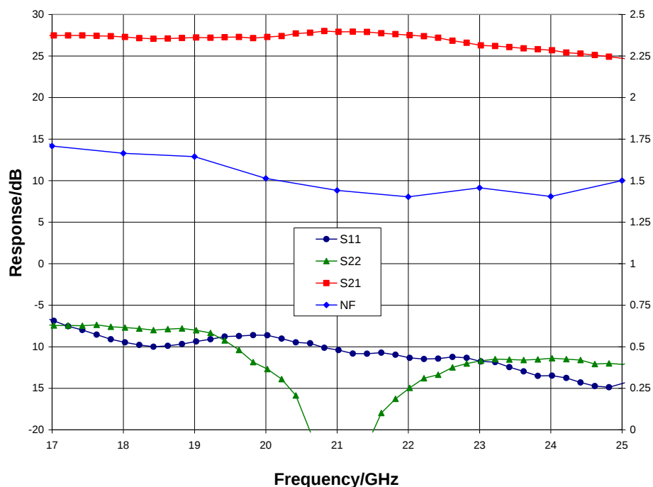
Narrow-band Performance, V_{dd} = 3.0 V, V_{gg} = 1.5 V, I_{dd} = 27 mA, T_A = 25^\circ C
