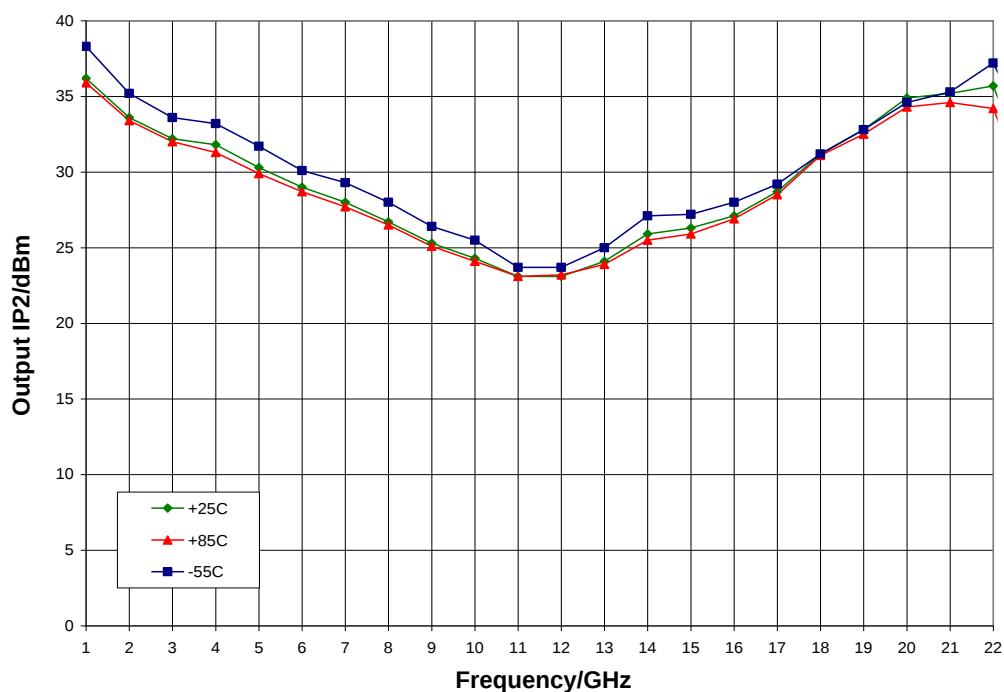
Output IP2 vs. Temperature, V_{dd} = 8.0\text{ V} , V_{gg} = 3.0\text{ V}
