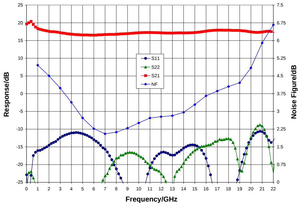
Narrow-band Performance, V_{dd} = 8.0 V, V_{gg} = 3.0 V, T_A = 25^\circ C
