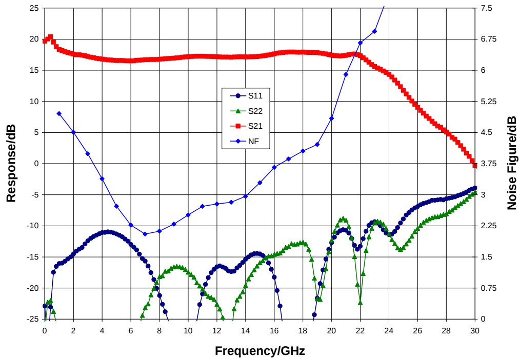
Broadband Performance, V_{dd} = 8.0 V, V_{gg} = 3.0 V, T_A = 25^\circ C
