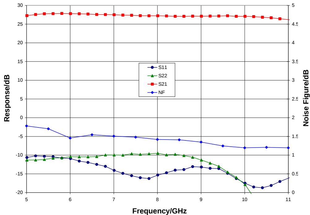
Narrow-band Performance, V_{dd} = 4.0 \text{ V} , T_A = 25^\circ \text{C}
