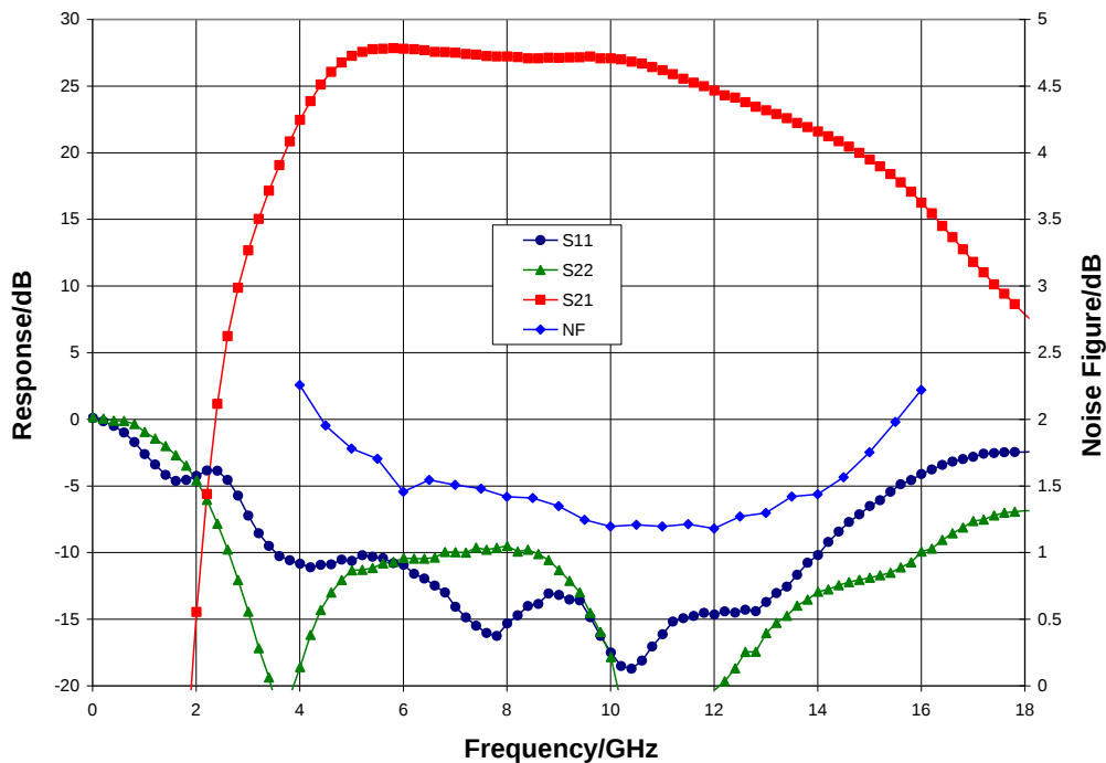
Broadband Performance, V_{dd} = 4.0 \text{ V} , T_A = 25^\circ \text{C}
