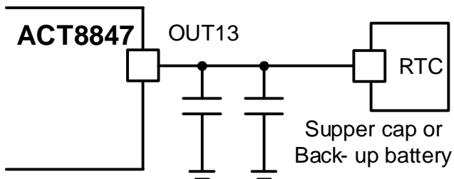
Figure 5: Typical Application of RTC LDO
