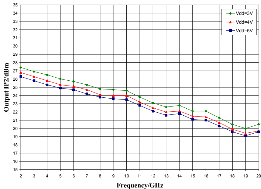
Output IP2 vs. V_{dd} , I_{dd} = 40\text{ mA} , T_A = 25^\circ\text{C}
