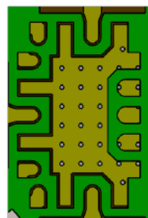
MOUNTING DETAIL
