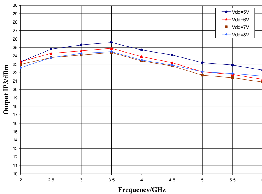
Output IP3 vs. Supply Voltage, T_A = 25^\circ\text{C}
