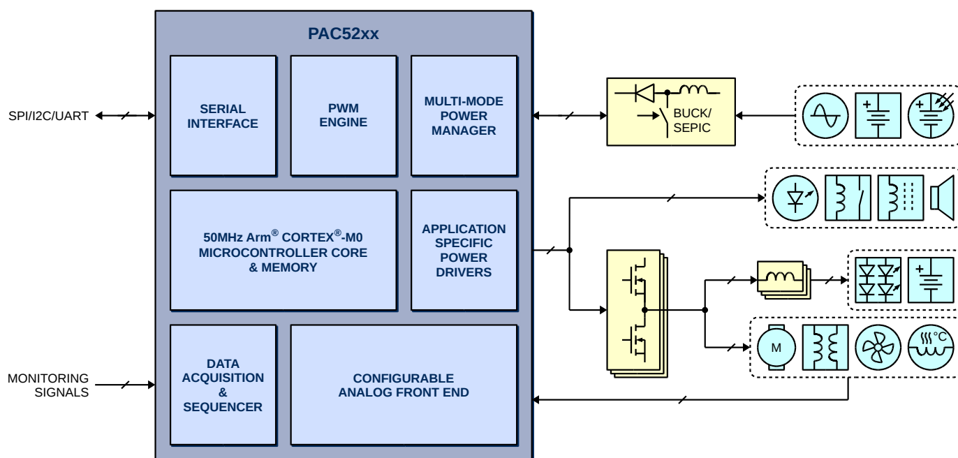
Figure 2-1 Simplified Application Diagram
