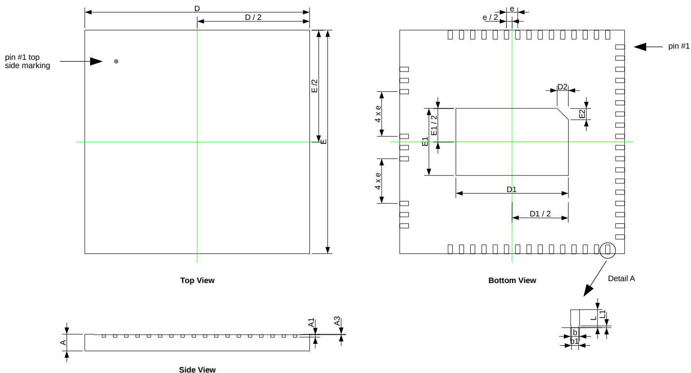
Figure 22-1 TQFN1010-57
