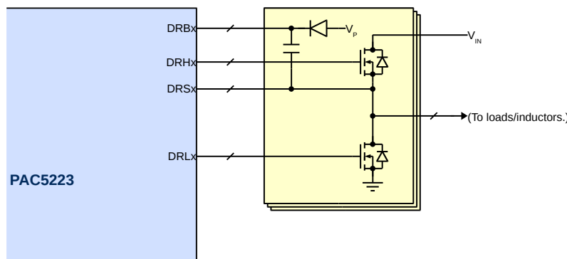
Figure 12-2 Typical Gate Driver Connections
