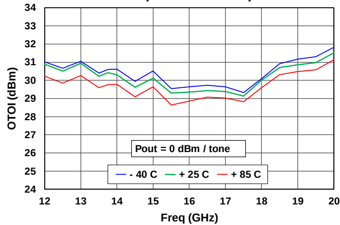
Output TOI vs Temp
