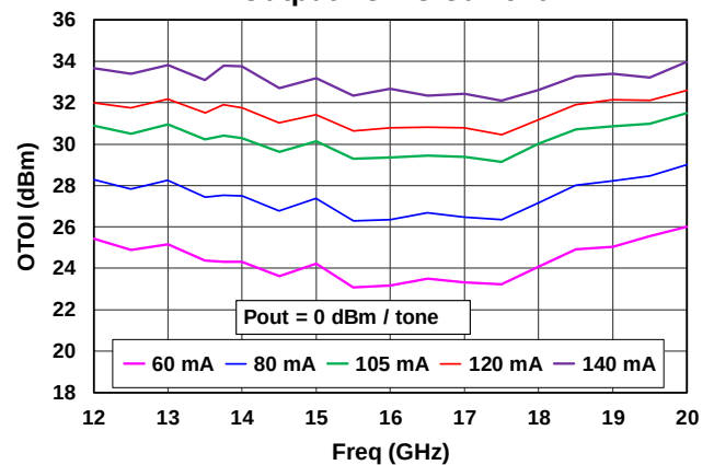
Output TOI vs Current
