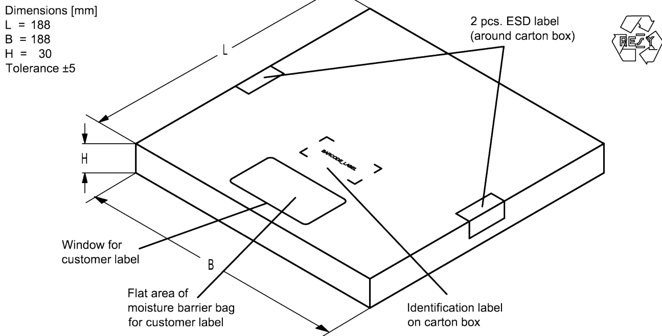
Figure 10: Drawing of folding box for reel with diameter of 180 mm.
