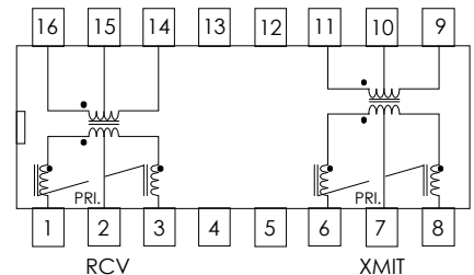
SCHEMATIC DIAGRAM "H"
