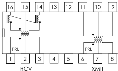
SCHEMATIC DIAGRAM "F"
