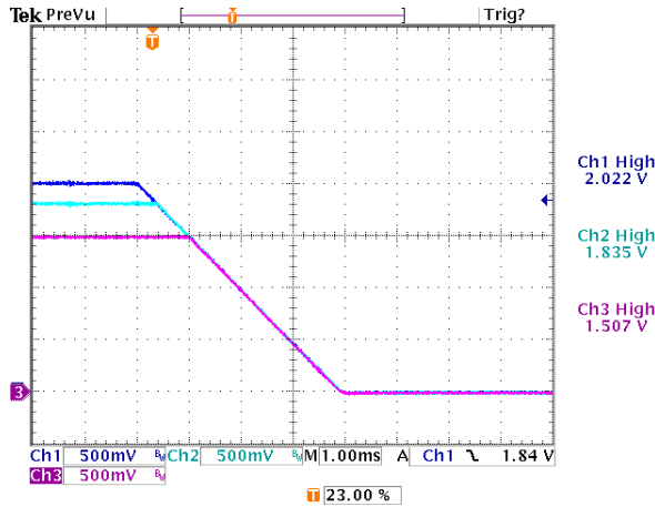
Figure 24. Tracking Turn-Off. Falling Slew Rate is Programmed at 0.5V/ms.
