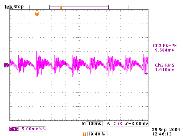
Figure 44. Output Voltage Noise, Full Load, 180° Interleave
