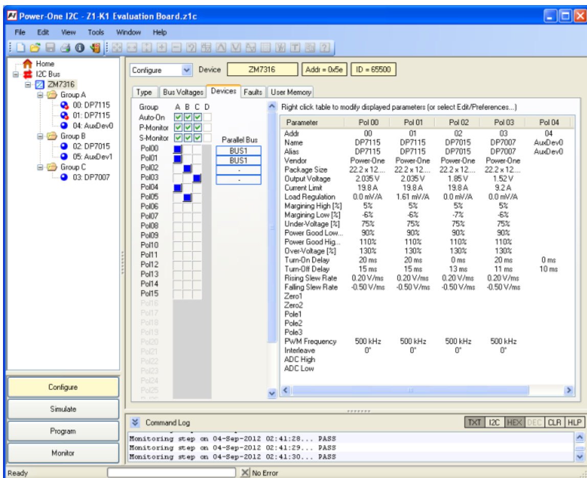
Figure 49 Evaluation Board Configuration showing Current Share Bus Assignment
