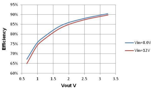
Figure 7. Efficiency vs V_{out} , Load=40A, F_{sw}=500kHz
