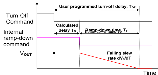
Figure 16. Relationship between Turn-Off Delay and Falling Slew Rate
