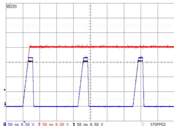
Figure 37. Turn-On into UVP on V3. The UV Fault Is Programmed To Be Non-Latching and Propagate From Group C to Group A. Ch1 – V3 (Group C), Ch2 – V2, Ch3 – V1 (Group A)
