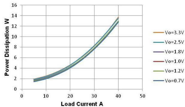
Figure 6. Dissipation vs Load, V_{in}=8V , F_{sw}=500kHz
