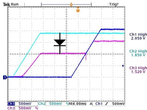
Figure 23. Turn On into Prebiased Load. V3 is Prebiased by V2 via a Diode.
