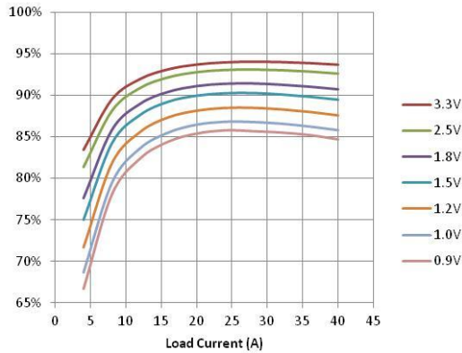
Figure 3. Efficiency vs. Load, V_{in}=12V , F_{sw}=500kHz
