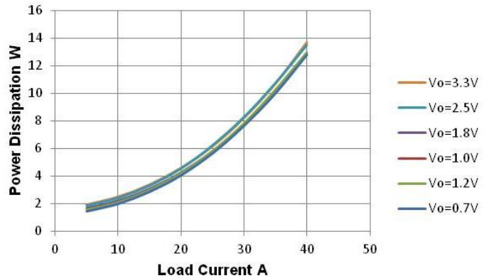
Figure 4. Dissipation vs Load, V_{in}=12V , F_{sw}=500kHz
