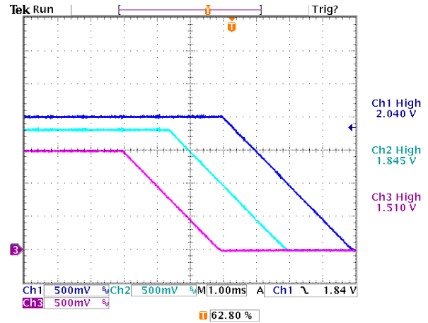
Figure 25. Turn-Off with Tracking and Sequencing. Falling Slew Rate is Programmed at 0.5V/ms.
