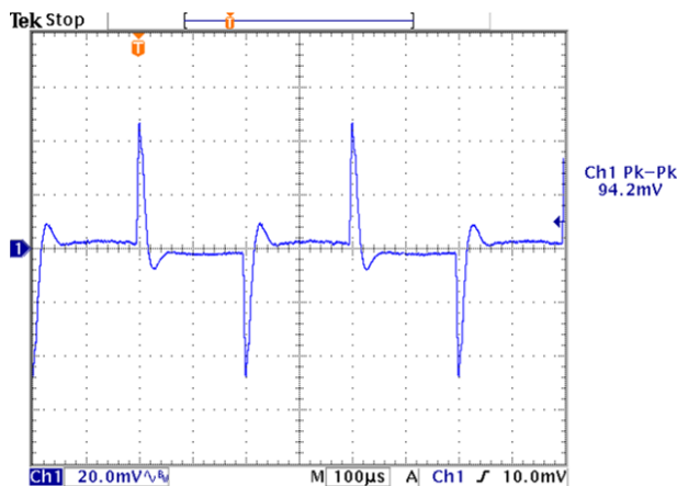
Figure 12 Transient Response with Regulation set to 0 mV/A.
