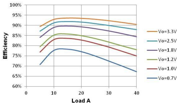
Figure 5. Efficiency vs Load, V_{in}=8V , F_{sw}=500kHz
