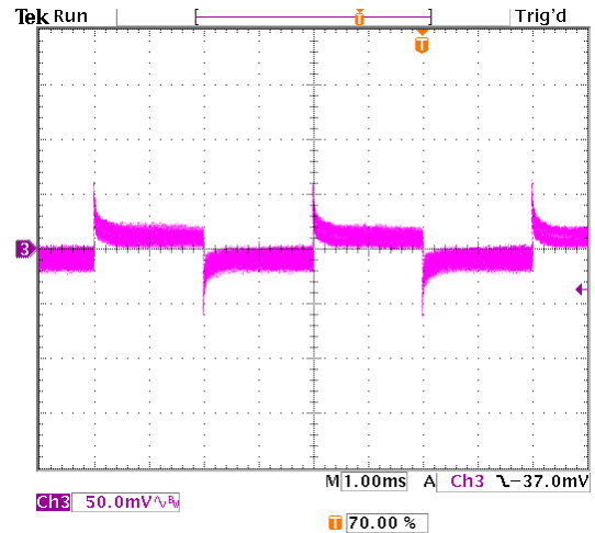
Figure 47. Transient Response with Regulation set to 0.55mV/A
