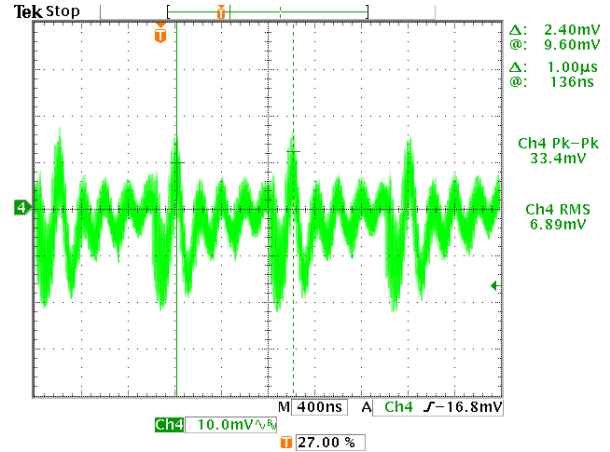
Figure 42. Input Voltage Noise with Interleave
