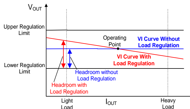
Figure 11. Optimal Voltage Positioning Concept
