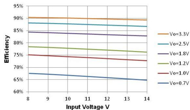
Figure 8. Efficiency vs V_{in} , Load=40A, F_{sw}=500kHz
