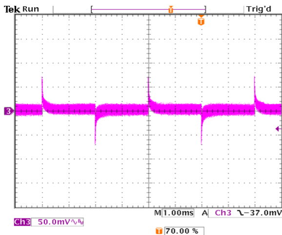
Figure 46. Transient Response with Regulation set to 0.0 mV/A
