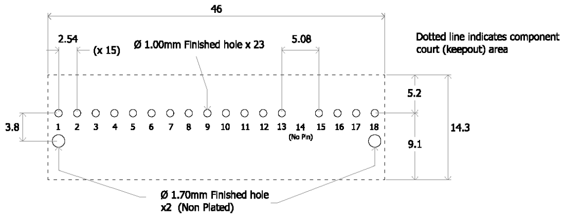
Figure 55. Pinout Diagram (Bottom View)
