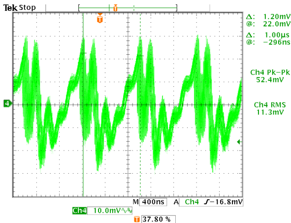
Figure 41. Input Voltage Noise, No Interleave
