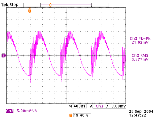
Figure 43. Output Voltage Noise, Full Load, No Interleave
