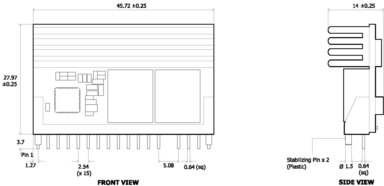
Figure 54. Mechanical Drawing
