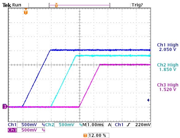
Figure 21. Sequenced Turn-On. Rising Slew Rate is Programmed at 1V/ms. V2 Delay is 2ms, V3 delay is 4ms.
