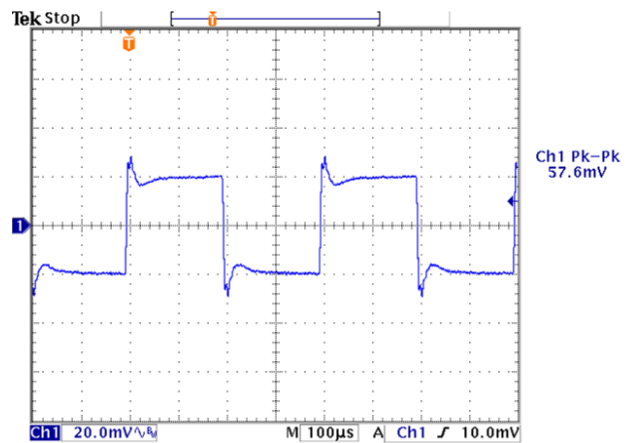
Figure 13 Transient response with non-zero Regulation.
