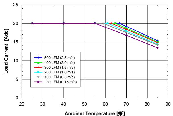
Figure 2. Available output current vs. ambient air temperature and airflow rates for converter DP8140G mounted horizontally with air flowing from input to output, MOSFET temperature \leq 120^\circ\text{C} , V_{in} = 12\text{ V} , V_{out} = 5\text{ V} , and F_{sw} = 500\text{ KHz}
