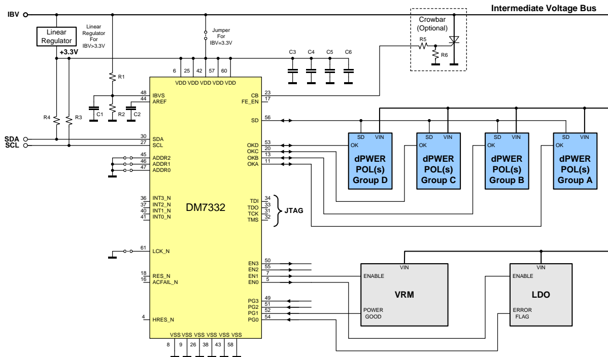
Figure 52. Multi-dPOL Power System Diagram
