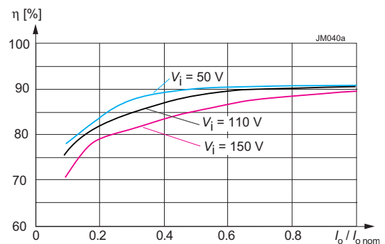
Fig. 10c Efficiency versus input voltage and load. Typical values (110IMY70-24-24)
