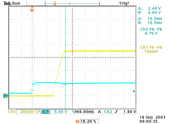
Figure 7. Vin=5V, Vout=0.7V, Iout=8.5A. Ch1 – Vout, Ch2 – Vin
