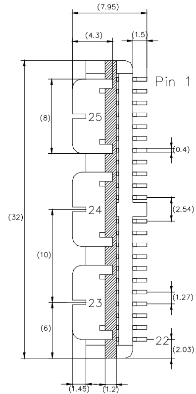
BOTTOM VIEW (Pin-out)
