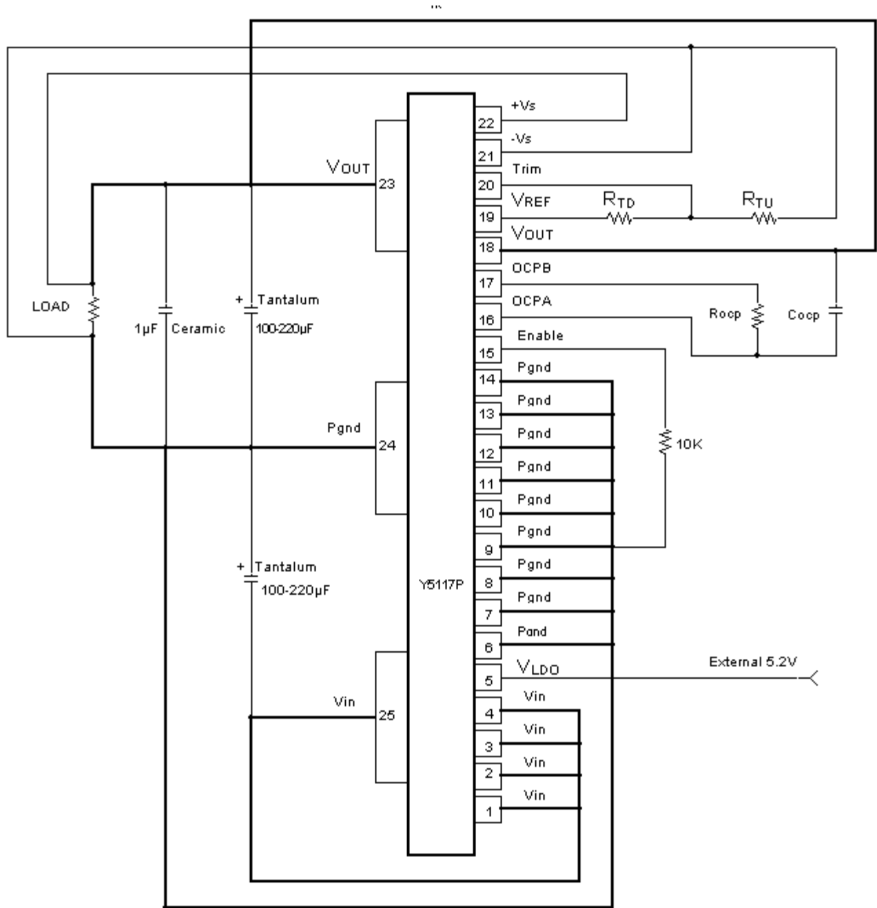
Figure 12. Typical Application Circuit for 5.2\text{VDC} > V_{in} \geq 3.0\text{VDC} . V_{LDO} is connected to the external voltage source. 10kOhm resistor is placed between the Enable pin and Pnd.
