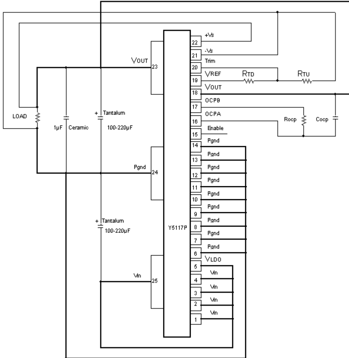
Figure 11. Typical Application Circuit for V_{in} \geq 5.2VDC . V_{LDO} is connected to V_{in}
