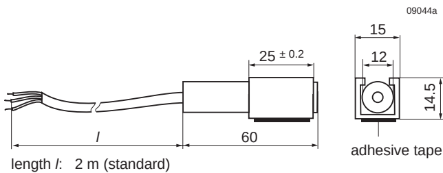
Fig. 58 Mechanical dimensions (in mm)
