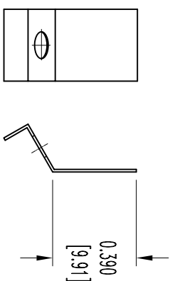
LOCKARM SPRING
