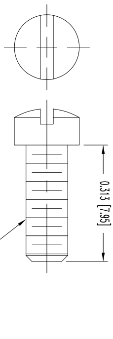
SCREW
