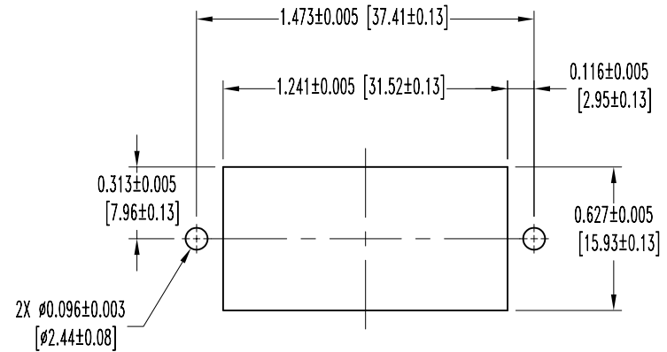
PANEL CUTOUT
