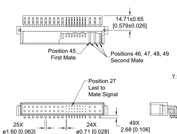
CONNECTOR DIMENSIONS
