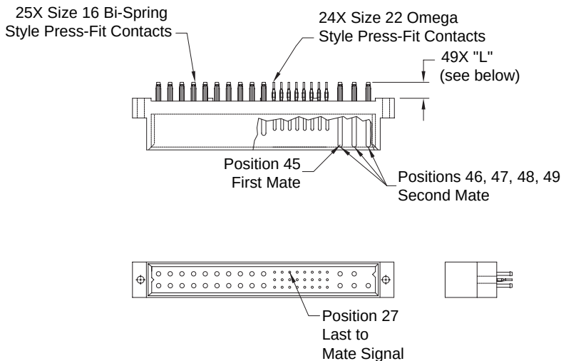
CONNECTOR DIMENSIONS
