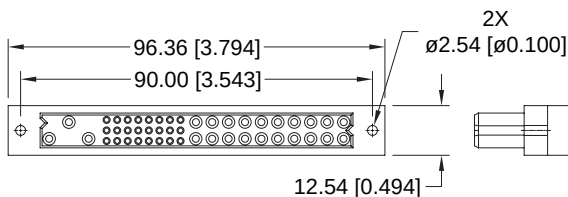
CONNECTOR DIMENSIONS
