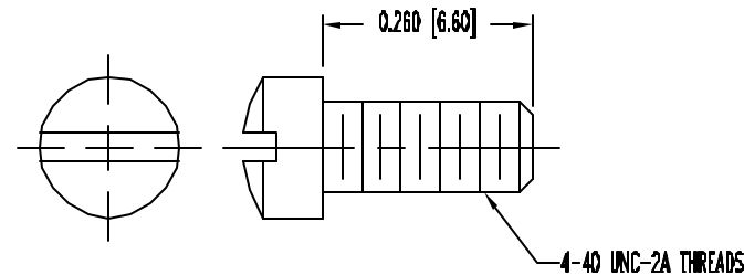
SCREW
