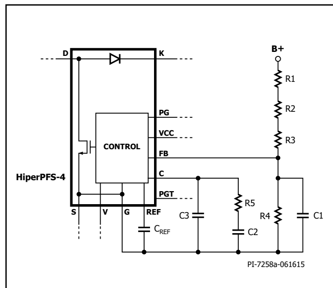
Figure 14b. Recommended Feedback Circuit with Integrated Diode.
