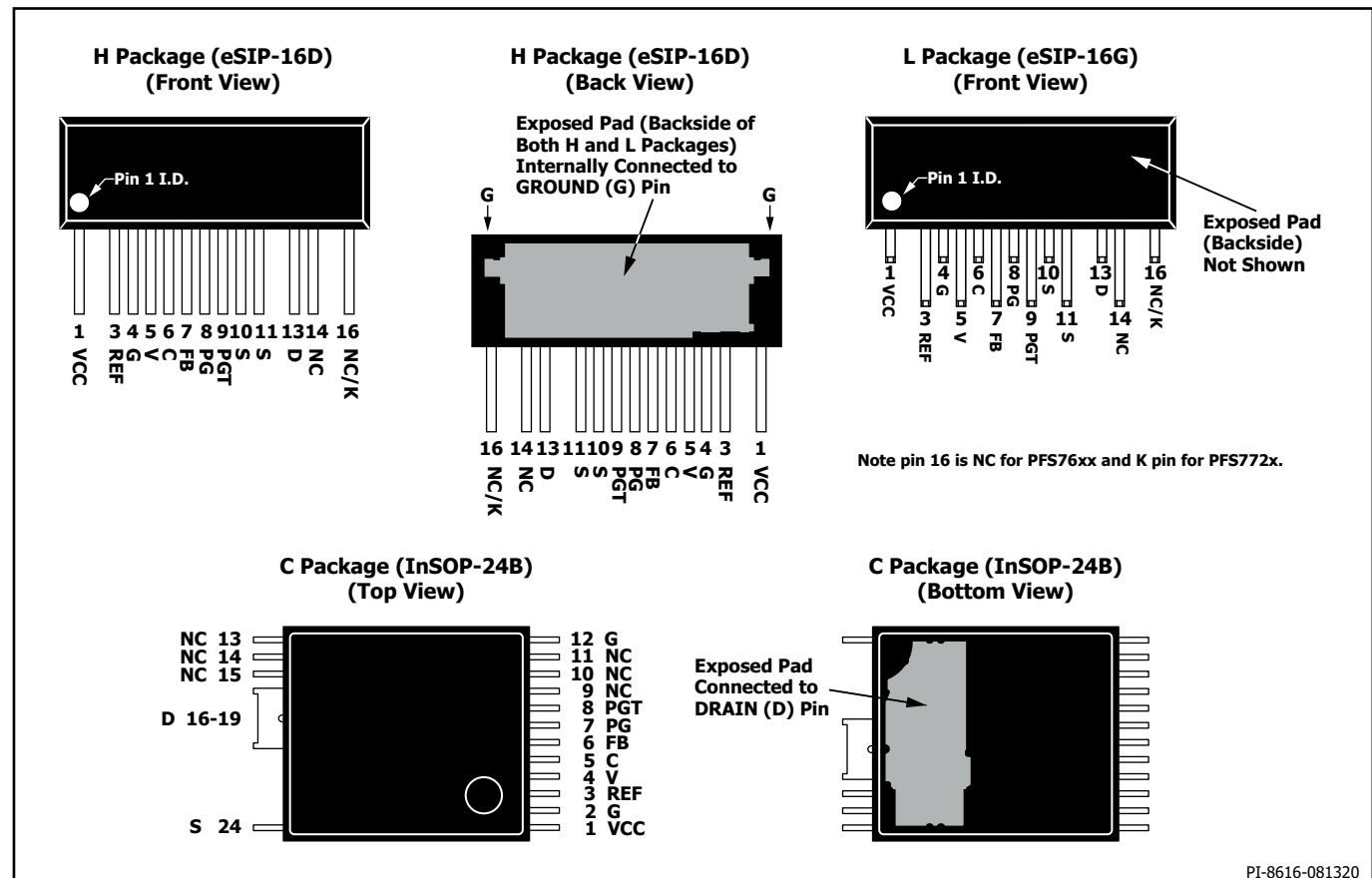
Figure 3. Pin Configuration.
