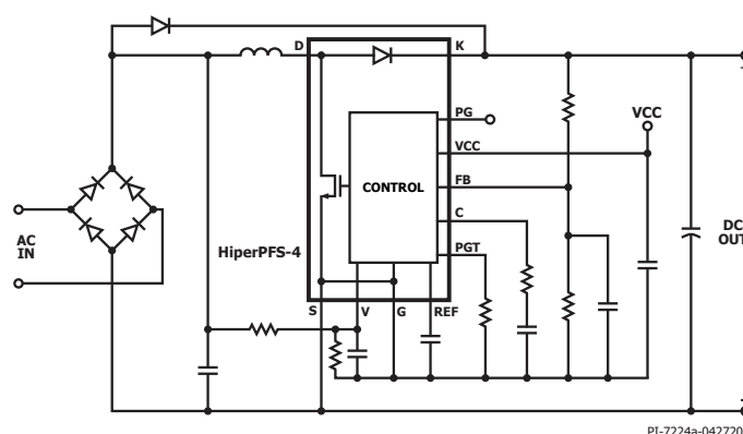
Figure 1b. Typical Application Schematic with Integrated Diode.
