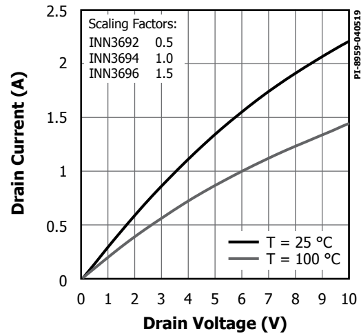
Figure 32. Output Characteristics.
