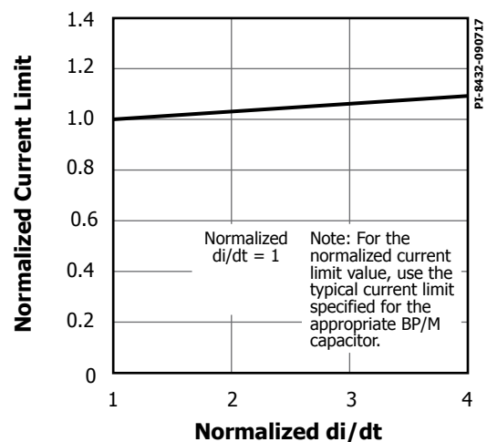
Figure 30. Standard Current Limit vs. di/dt.
