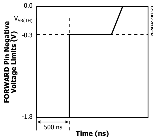
Figure 29. FORWARD Pin Negative Voltage Limits.
