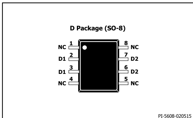
Figure 3. Pin Configuration.
